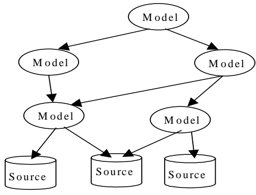
Figure 2. Model dependencies
