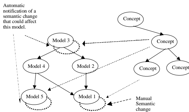
Figure 5. Semantic change
