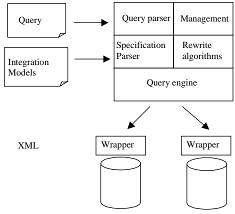
Figure 1. Architecture
