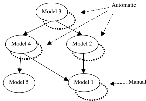
Figure 4. Propagated versioning
