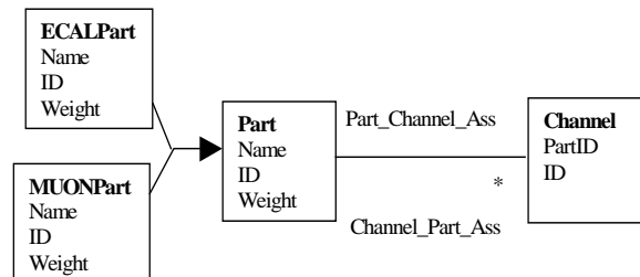
Figure 3 Integration models
