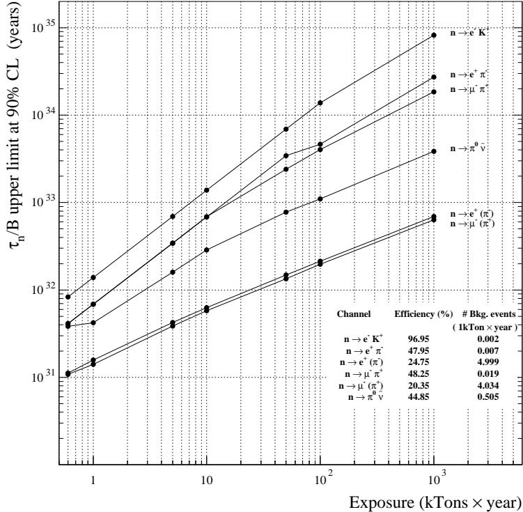
ICARUS: Limits on Neutron Decay
