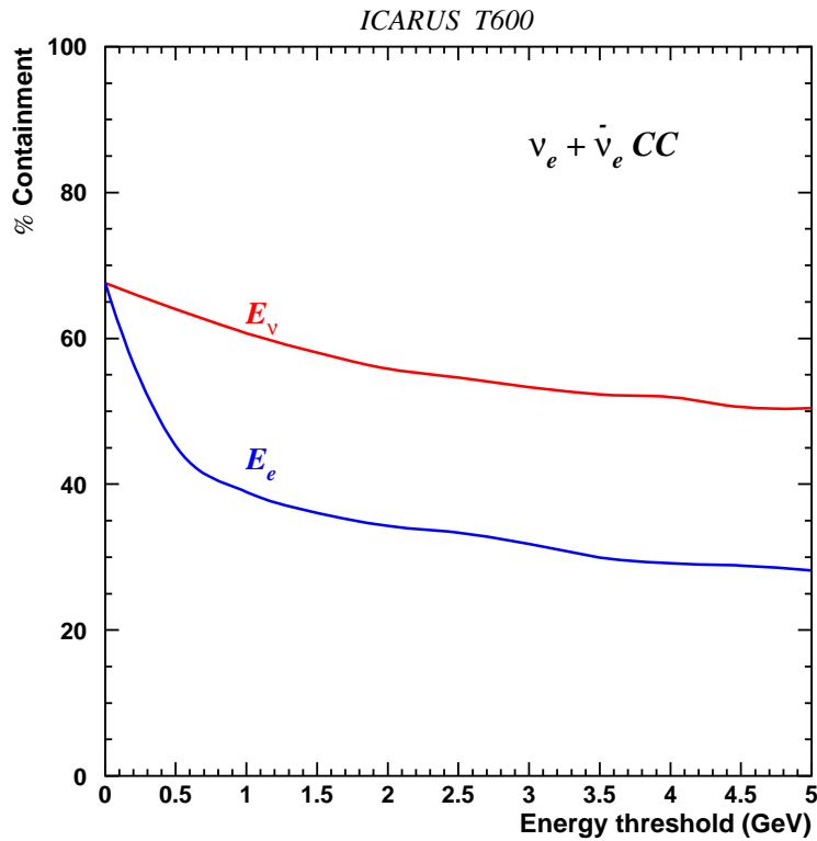
Figure 3: Integral distributions showing the containment for CC events as a function of the neutrino energy and the leading lepton momentum. Top plot: \nu_\mu + \bar{\nu}_\mu \text{ CC} . Bottom plot: \nu_e + \bar{\nu}_e \text{ CC} .
