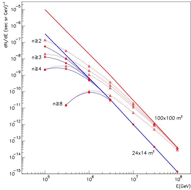
Figure 3.10. The primary cosmic ray energy spectrum for two arrays and the effect of a n -fold coincidence (as described in the text) on it.
