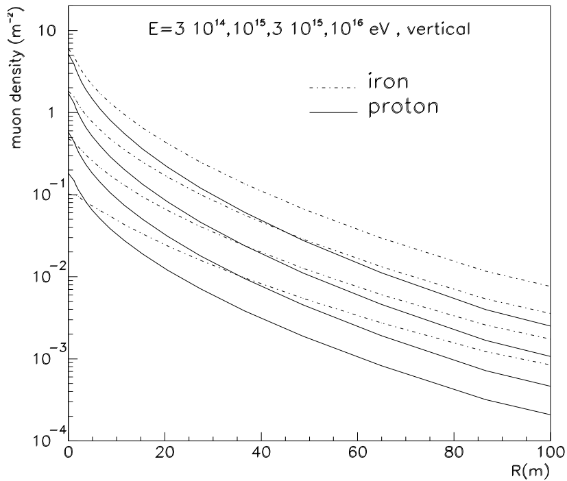
Figure 1.6. CORSIKA Monte-Carlo simulations of the muon density for proton and iron induced showers of various energies as a function of the radial distance from the shower center
