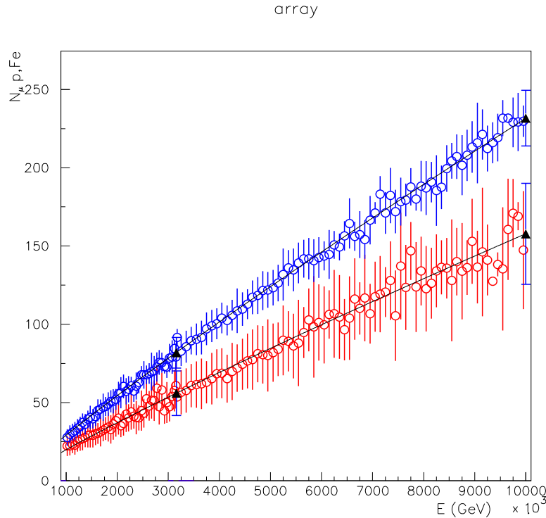
Figure 4.3. Number of muons ( N_{tot} ) in the array as function of energy, for p and Fe. The black triangles refer to simulation at fixed energy. The fit through these points is also shown (top curve: iron; bottom curve: proton).
