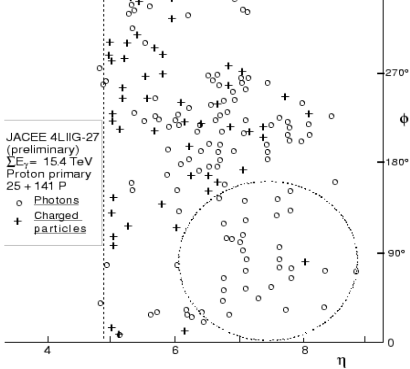
Figure 1.8. Example of a high multiplicity event with an anomalous concentration of photons in a limited range of phase space [31].
