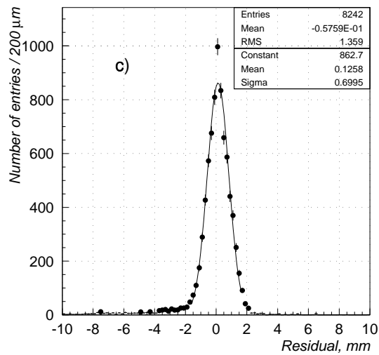
Figure 2.3. Calibration of DELPHI chambers: a) drift chamber efficiency as a function of anode voltage for the Ar:CO 2 :CH 4 90:5:5 gas mixture; b) drift chamber efficiency as a function of the drift distance for the same gas mixture and anode voltage 6.0 kV. Lines are drawn to guide the eye; c) hit residual distribution along the drift direction; d) hit residual distribution for the longitudinal read-out with delay lines.
