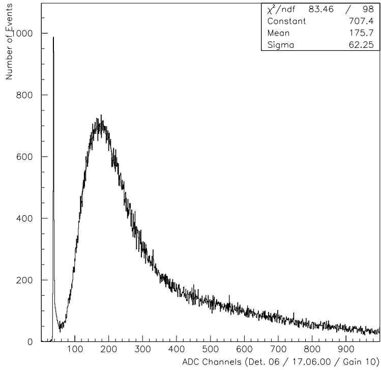
Figure 3.7. Response of the L3C air shower counters to a minimum ionizing particle.
