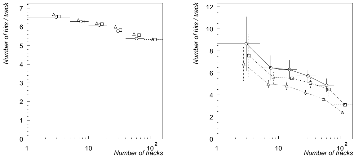
Figure 2.9. Number of used (left) and unused (right) hits per track after the 1'st and 2'nd iterations. Notations as in Fig. 2.8.
