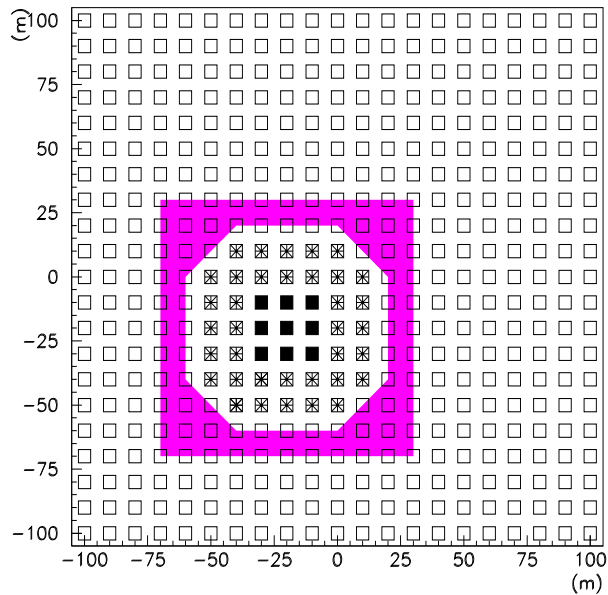
Figure 4.10. The different groupings of surface array detectors defined relative to the core of large zenith angle showers: “D0” - solid; “D3” - asterisk; “D6” - shaded.
