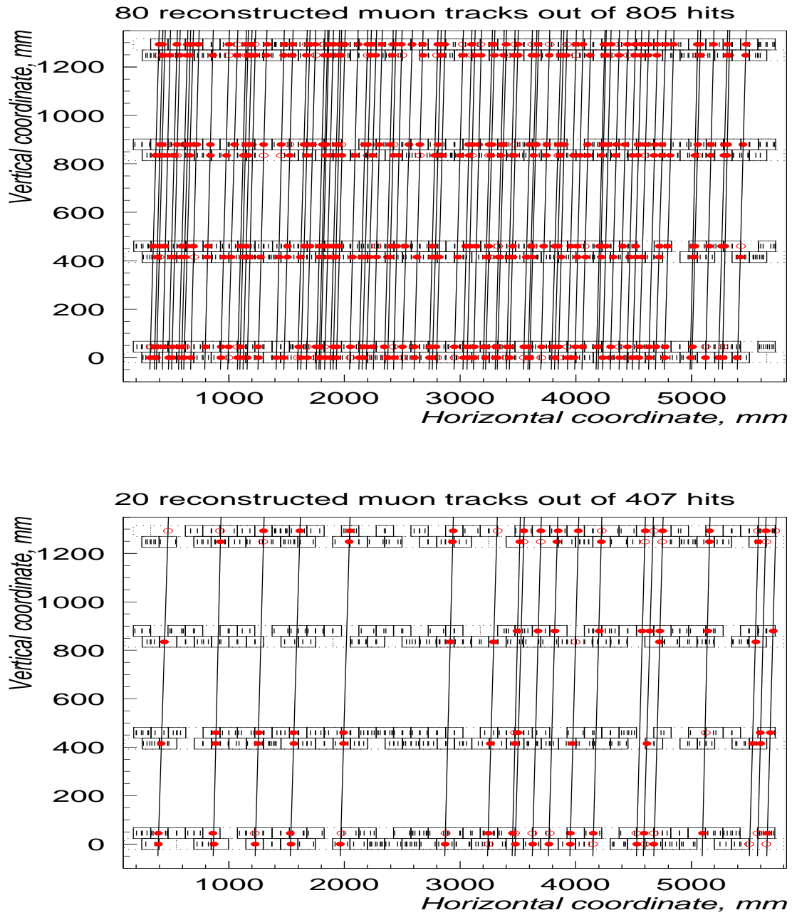
Figure 2.10. The highest multiplicity event found in the test run with the total multiplicity 100 tracks. Top: reconstructed tracks after the 1 st iteration. Bottom: the additional tracks after the 2 nd iteration.
