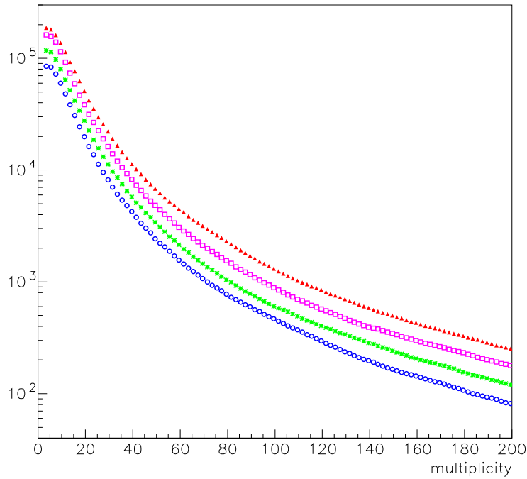
Figure 4.1. The integral muon multiplicity distributions in the underground array for different primary particles for a running time of 2 \cdot 10^7 sec.
