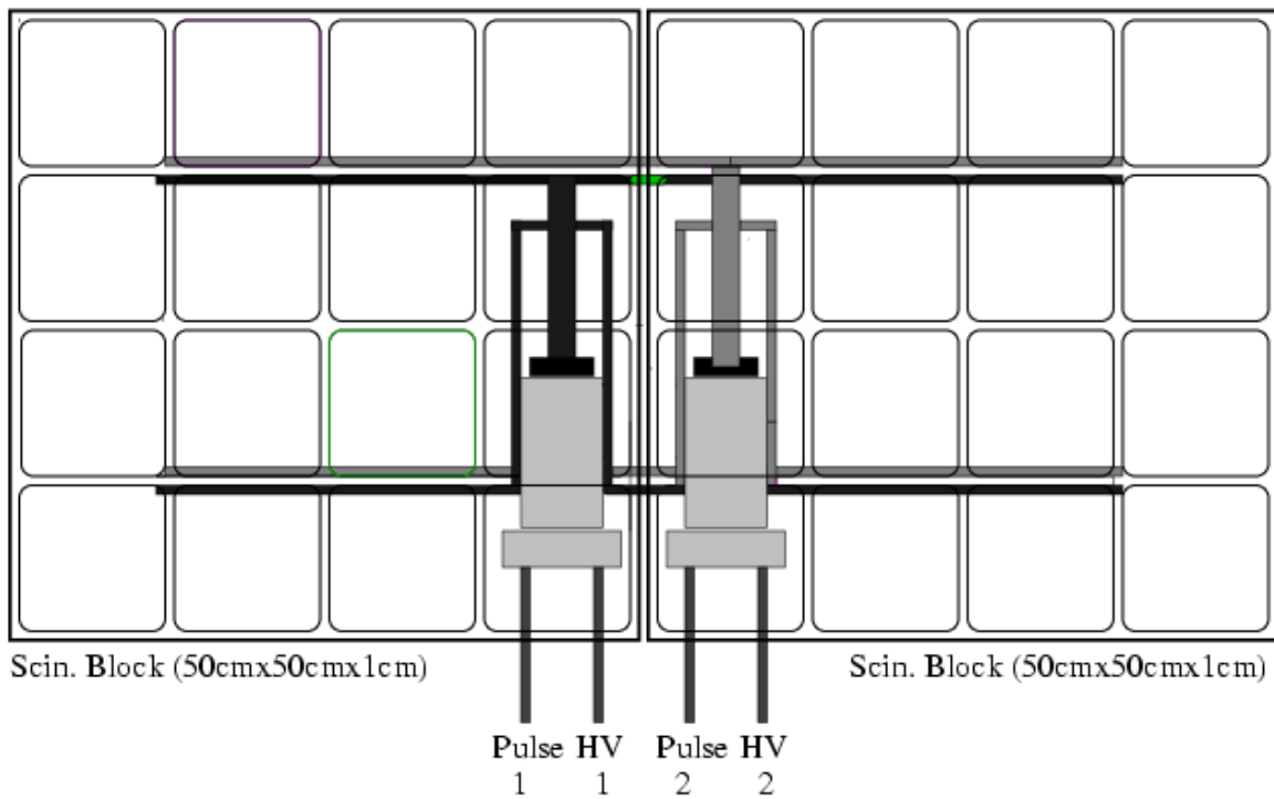
Figure 3.6. The L3C scintillator modules.
