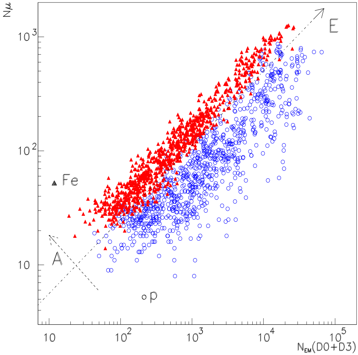
Figure 4.7. Number of muons versus number of electromagnetic particle in an area 60 \times 60 \text{ m}^2 , shower cores at a distance R < 10 \text{ m} , 10^{15} < E < 5 \cdot 10^{16} , 15^\circ < \theta < 30^\circ
