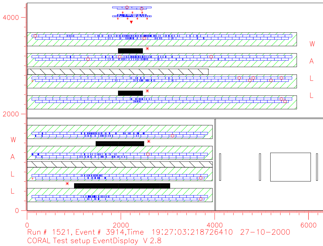
Figure 2.5. Shower from the rock of the overburden.
