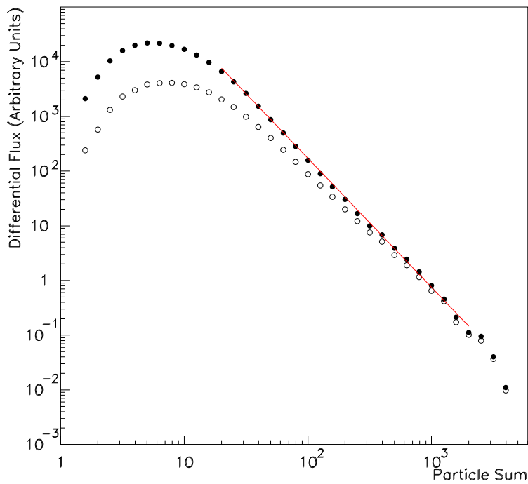
Figure 3.9. Flux (in arbitrary units) versus the sum of all particles, obtained from the pulse heights of the hit counters. The open circles represent events with at least one muon in the L3 muon chambers.
