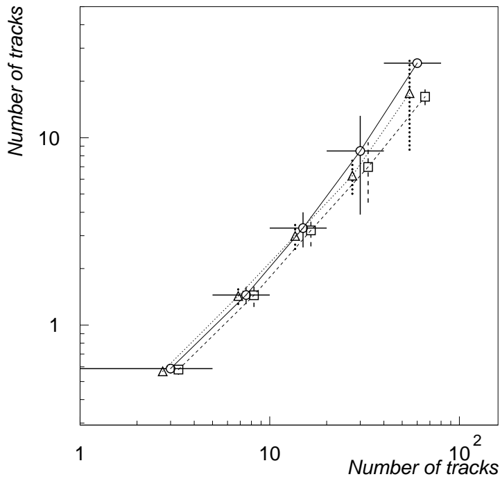
Figure 2.8. Number of reconstructed tracks in the 2'nd iteration vs that in the 1'st. Circles for 1 mm measurement error, squares for 1.5 mm and triangles for 2 mm.
