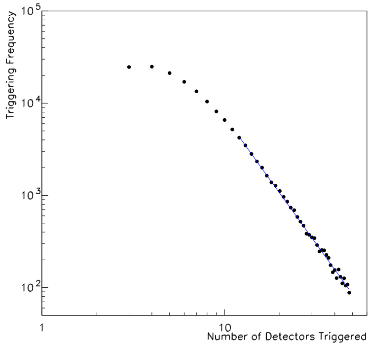
Figure 3.8. Trigger frequency (in arbitrary units) versus the number of hit counters from a 50 counters array above L3.
