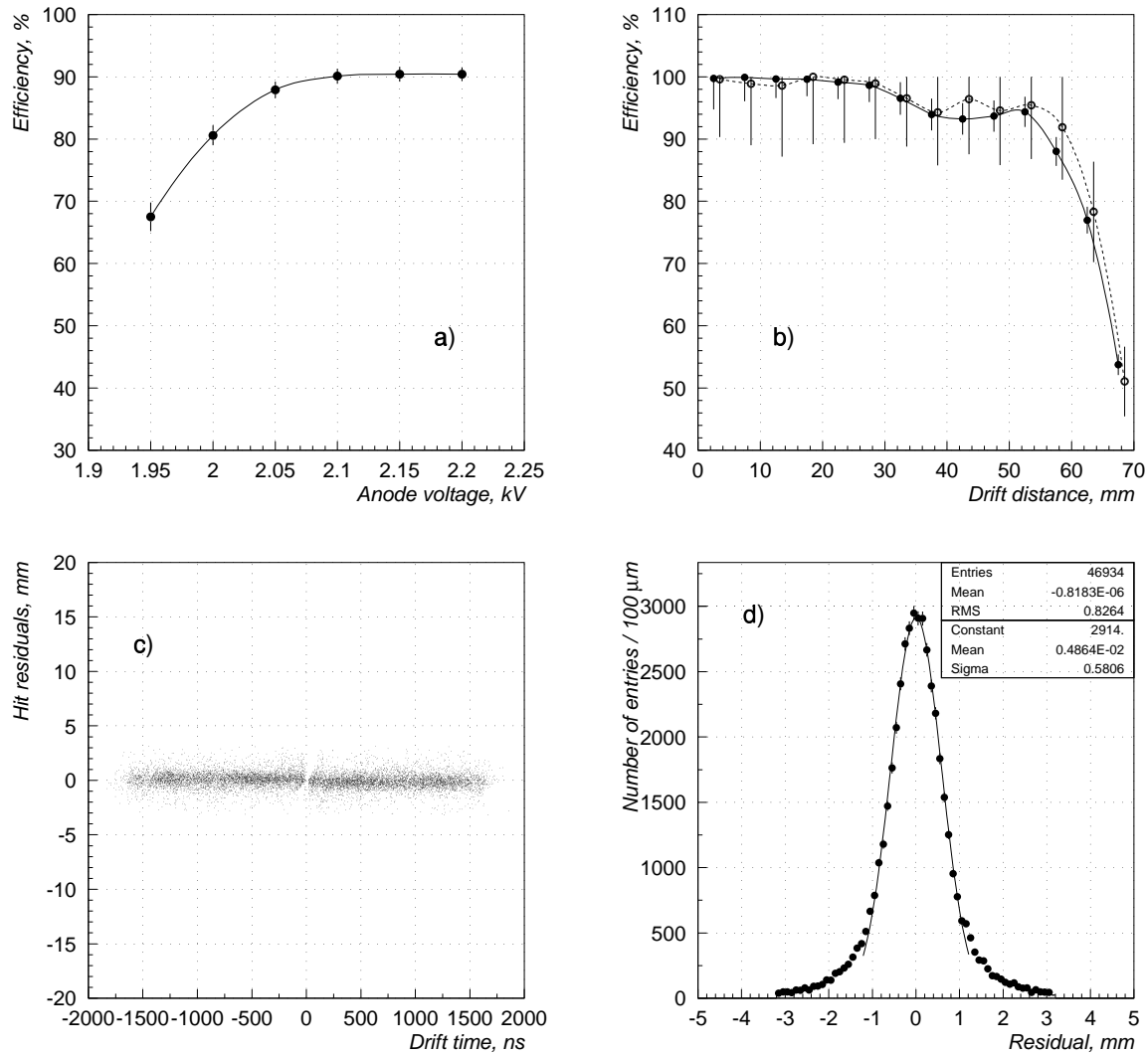
Figure 2.2. Calibration of UA1 chambers: a) drift chamber efficiency as a function of anode voltage for the Ar:CO 2 :CH 4 90:5:5 gas mixture; b) drift chamber efficiency as a function of the drift distance for the same gas mixture and anode voltage 2.1 kV. Full circles for track incident angles -15^\circ < \alpha < 15^\circ , open circles for 15^\circ < |\alpha| < 30^\circ . Lines are drawn to guide the eye; c) hit residuals vs signed drift time; d) hit residual distribution.
