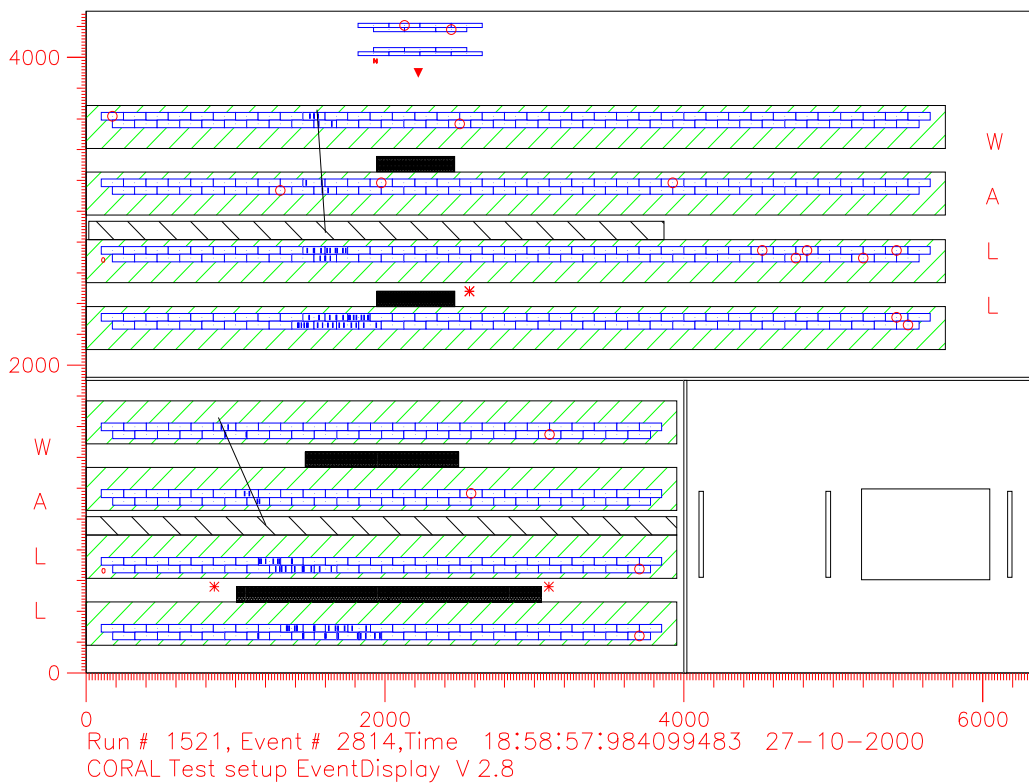
Figure 2.6. Muon-induced shower in the absorber
