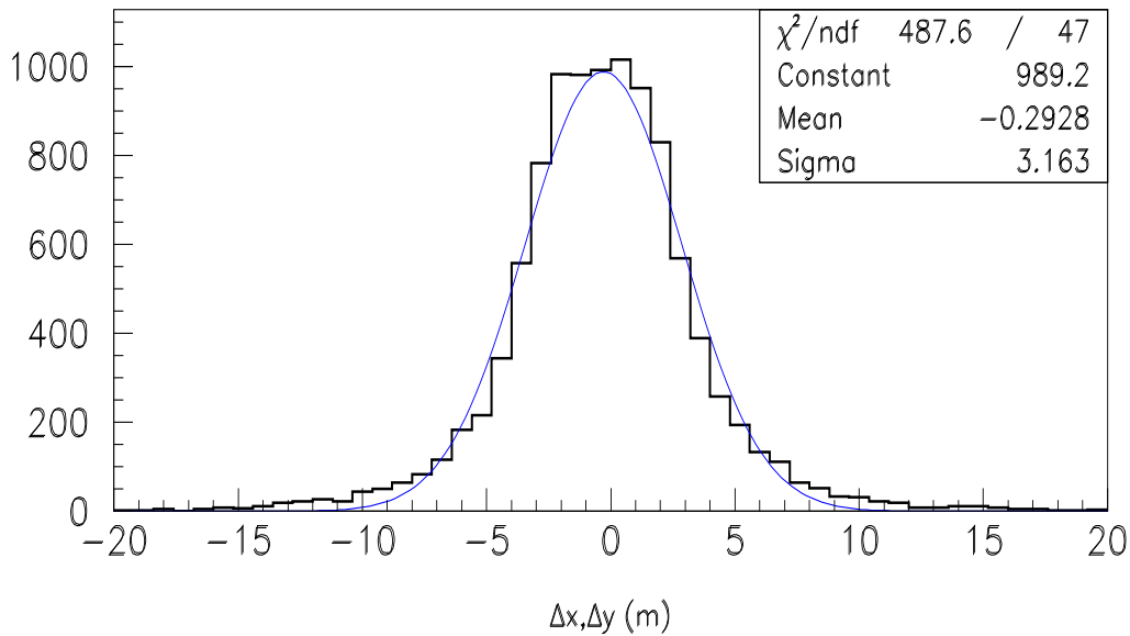
Figure 4.5. The difference between the real and the estimated position for proton induced showers, with \theta < 30^\circ , and energy between 10^{15} - 10^{16} eV.
