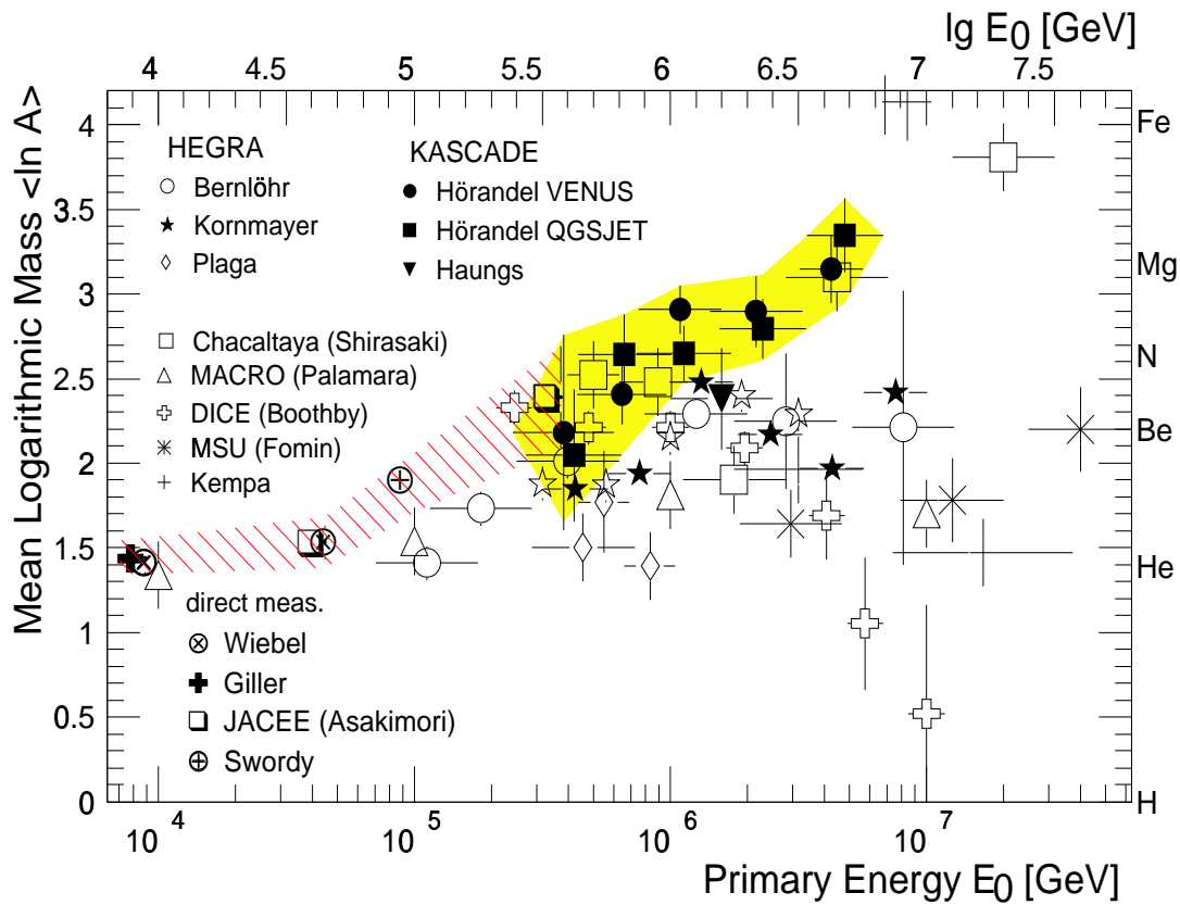
Figure 1.2. Chemical composition of primary cosmic rays (from [17]).
