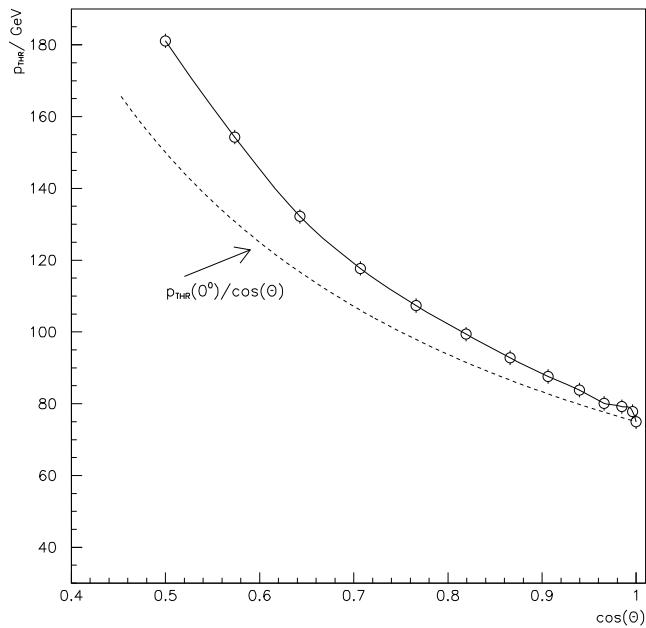
Figure A.4. Dependence of the muon threshold momentum p_{THR} as a function of zenith angle.
