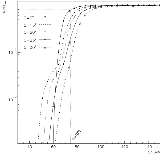
Figure A.2. Fraction of muons reaching the detector as a function initial muon momentum for several zenith angles, \theta . The definition of the threshold momentum, p_{THR} , is illustrated for \theta = 0^\circ .
