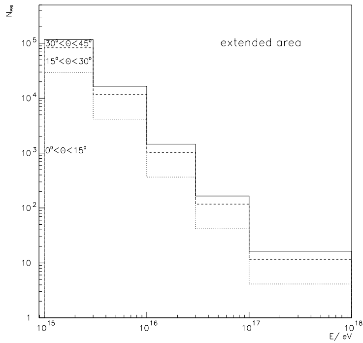
Figure 3.13. Number of events per energy bin, used in the analysis for the particle composition, for a run time of 6 \cdot 10^7 .
