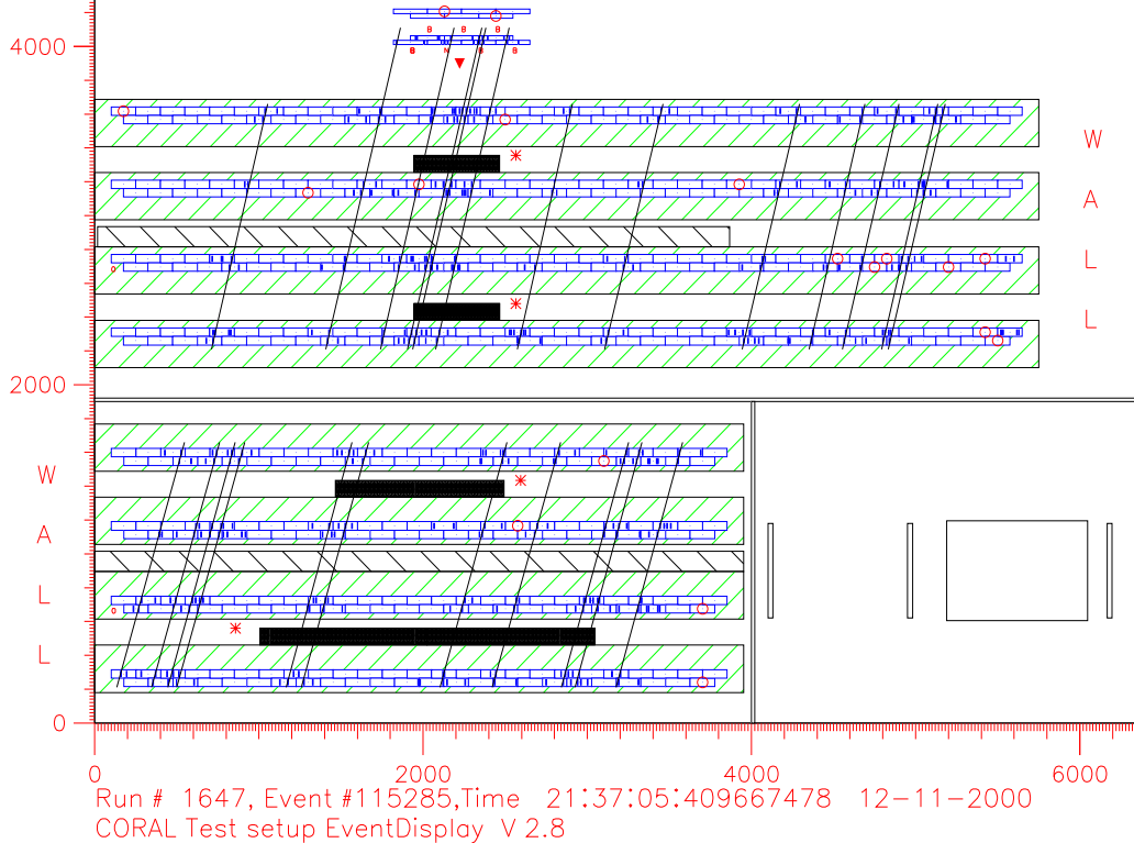
Figure 2.4. A multimuon event as displayed in two projections of the 6 m x 4 m muon chambers.
