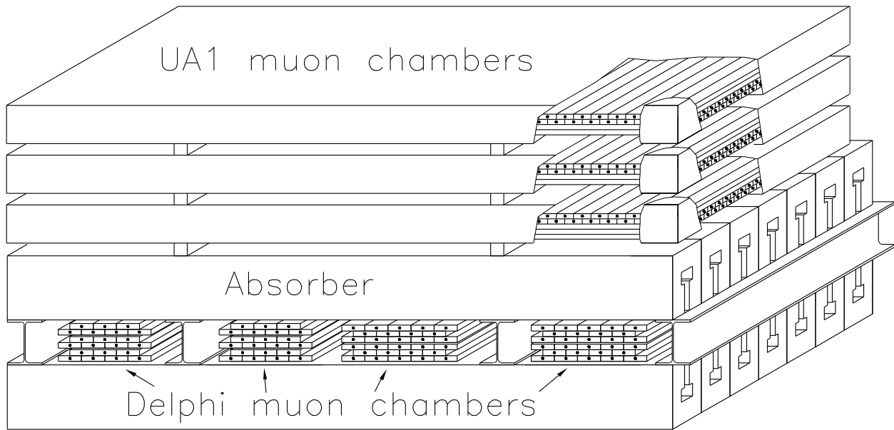
Figure 3.3. The principal set-up of the UA1 and DELPHI chambers with the 200 \text{ g/cm}^2 absorber in between
