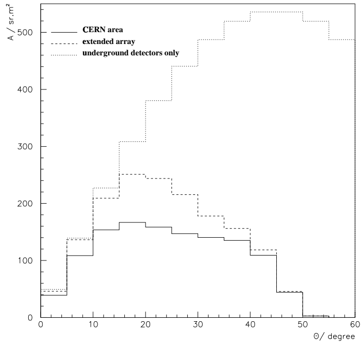
Figure 3.12. Geometrical acceptance of the combined surface - and muon array versus the zenith angle. Note that the top curve corresponds to an infinite surface array.
