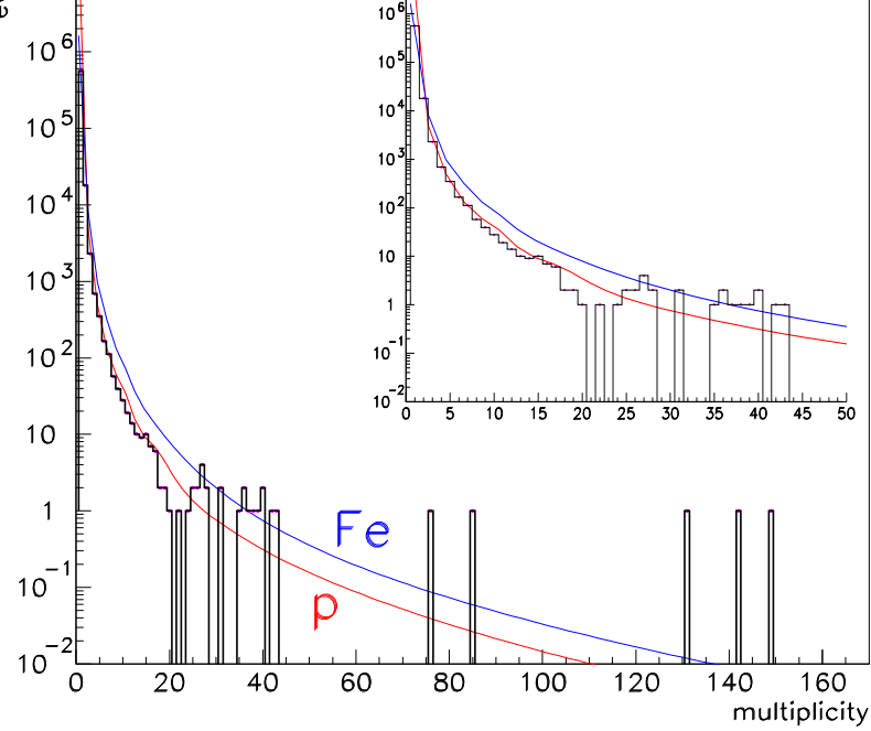
Figure 1.5. Multiplicity distribution of muons in the TPC compared to CORSIKA simulations for p and Fe as primary particle. The highest multiplicity event has twice the particle density (see Tab 1.1)
