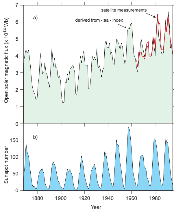
Figure 10: a) The total solar open magnetic flux (coronal source flux) derived from interplanetary observations for 1964–1996 (thick solid line) and derived from the \langle \text{aa} \rangle geomagnetic index for 1868–1996 (shaded curve) [2]. b) The variation of the annual mean sunspot number.
