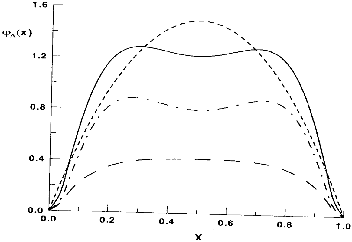
Figure 1: The axial projection of the pion distribution amplitude (solid line) at the low energy scale \mu_0^2 = 0.5 \text{ GeV}^2 . The contribution of the local part of vertex is shown by dash-dotted line and the contribution of nonlocal part by dashed line. The asymptotic distribution amplitude is shown by dotted line.
