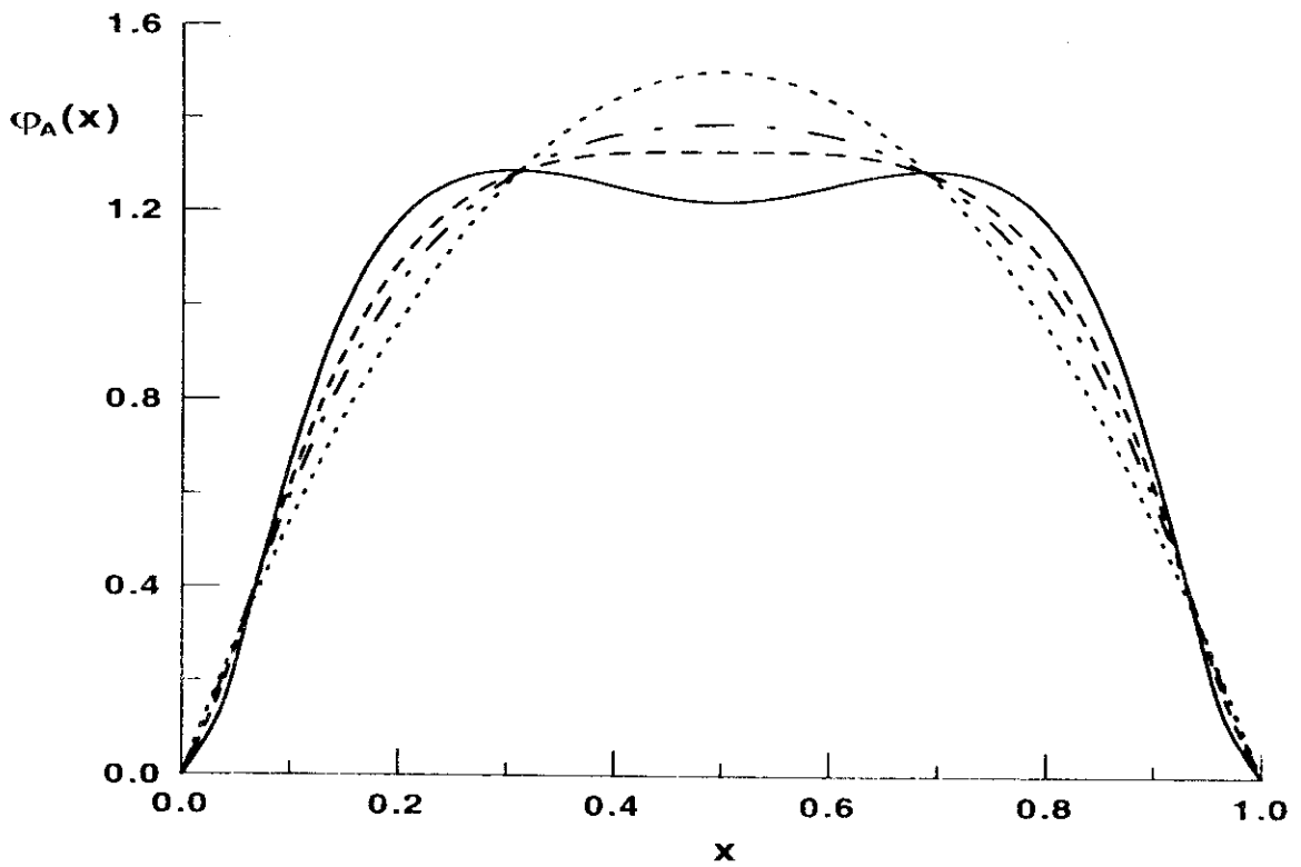
Figure 2: The axial projection of the pion distribution amplitude (solid line) at the low energy scale \mu_0^2 = 0.5 \text{ GeV}^2 and its evolution to higher momentum transfers squared: Q^2 = 1 \text{ GeV}^2 (dashed line), Q^2 = 10 \text{ GeV}^2 (dot-dashed line). The asymptotic distribution amplitude is shown by dotted line.
