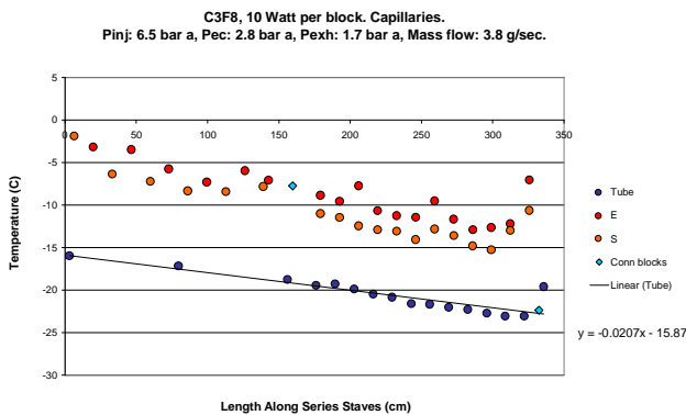
Figure 7: Barrel SCT Manifold Test with \text{C}_3\text{F}_8 : 10 Watts per block, two staves in series
