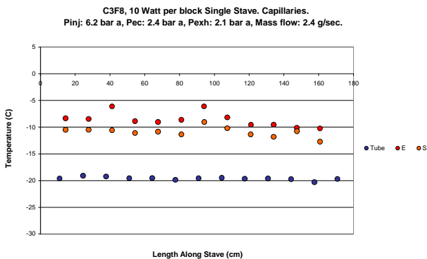
Figure 8: Forward SCT Manifold Test with \text{C}_3\text{F}_8 :
