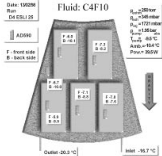
Figure 9: C Pixel Disk Sector Test Data (C- tube: \text{C}_4\text{F}_{10} )
