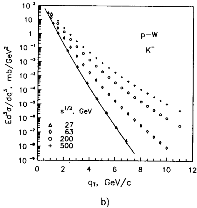
Figure 10. The dependence of inclusive differential cross section of K^- -meson production in p-Be (a) and p-W (b) collisions on the transverse momentum q_{\perp} at different colliding energy \sqrt{s} and \theta_{NN} \simeq 90^\circ . Points, \diamond —63 GeV, \circ —200 GeV, + —500 GeV, and solid line are calculation results. Experimental data, \triangle —27 GeV, are taken from [5].
