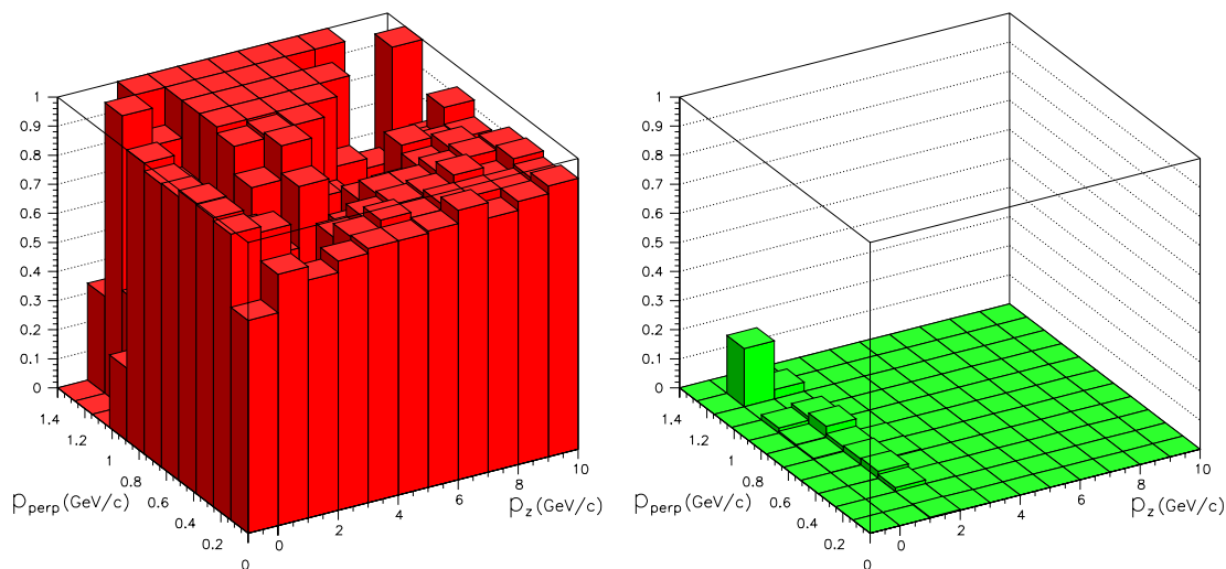
Figure 26: (left) Combined pion identification and geometrical acceptance of the detector and (right) global pion misidentification probability in bins of p_L , p_T from interactions of 15 GeV/ c protons.
