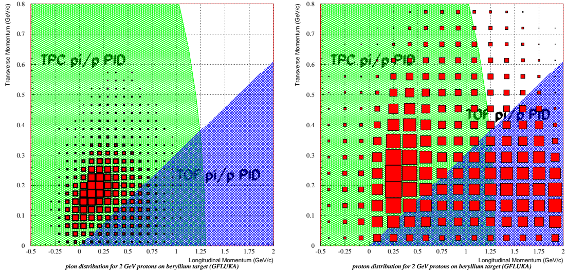
Figure 20: Production spectrum (by GEANT+FLUKA) d^2N/dp_T dp_L of (left) secondary pions and (right) secondary protons produced in collisions of protons of 2 GeV/c with a thin beryllium target. Superimposed are the areas of phase space expected to be covered by the \pi/p particle identification of the TPC and the TOF (at the 4\sigma level) in a simplified treatment.
