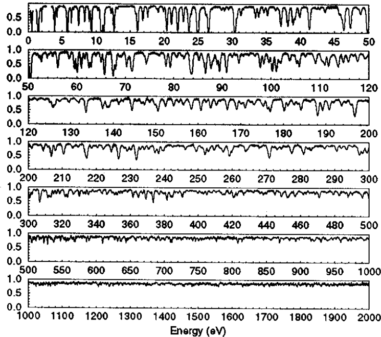
Figure 2 : Experimental transmission in function of the neutron energy between 0.3 eV and 2 keV for an \text{NpO}_2 sample with 2 \text{ g/cm}^2 of ^{237}\text{Np} placed at flight distance of 49,34 m and measured at room temperature.
