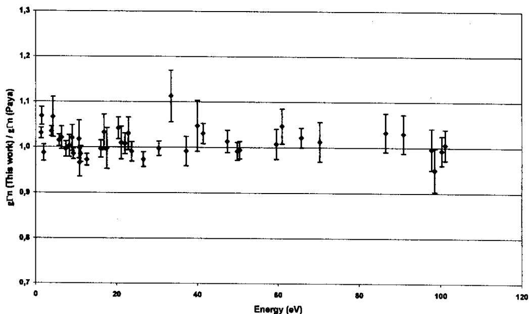
Figure 4 : Ratio between the values of neutron width determined in our experiments and the value of Paya [4] (used in JEF2.2 [15]) for selected resonances. The error is determined from the total uncertainty on each neutron width.
