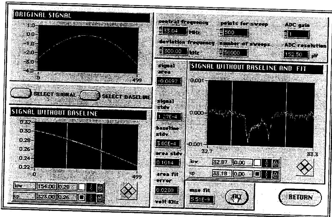
FIG 6: The TE peak on deuterated butanol (right) after a 50000 sweeps average. The signal was obtained after baseline subtraction and fitting (right).
