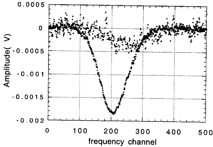
FIG. 5: The NMR TE peak in ammonia at 1.5 K (crosses) compared to the empty target measurement (open triangles). The amplitude of the signal in ammonia was divided by 10 to allow direct comparison. The small proton contamination (2%) in the empty target is essentially due to the Kapton window.
