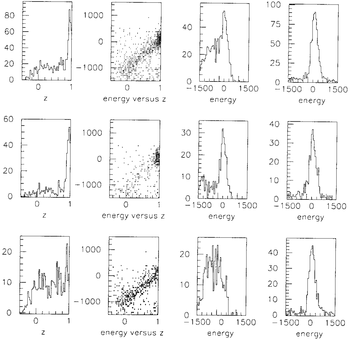
Figure 13: Energy and angular plots for coincidence events with the 6% radiator and 4 cm LH_2 target. The top row includes all the selected coincidence events, whereas the middle and bottom rows are those selected events satisfying the electron and photon cuts, respectively, in the veto detector. For each row, the first column is the parameter z , which is the cosine of the \pi^0 decay angle in its rest frame relative to the \pi^0 direction in the Lab and is reconstructed from the proton kinematics and photon angle measured in the calorimeter. The third column is the difference between the measured photon energy and that reconstructed based on ep kinematics. The second column is a scatter plot of the energy difference and z . The fourth column is the difference between the measured photon energy and that reconstructed based on (\gamma, \pi^0) kinematics (using the z information). In the z distribution, the peak near z = 1 comes from events having two-body kinematics, primarily ep scattering and RCS.
