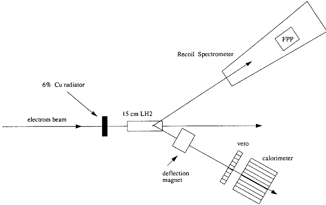
Figure 9: Plan view of the proposed experiment in Hall A.
