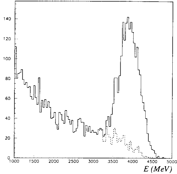
Figure 16: Monte Carlo calculation of the energy spectrum of RCS plus ep\gamma photons (solid) and ep\gamma photons alone (dashed) for E=6 GeV, \theta_{cm}=70^\circ . It has been assumed that backgrounds from ep elastic scattering and \pi^0 photons have been removed by appropriate kinematic cuts. The ratio of ep\gamma to RCS events in the region above 3500 MeV is \approx 0.20 .
