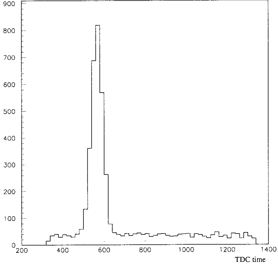
Figure 12: TDC spectrum for coincidences between the calorimeter and the HRS for the run with a 6% radiator, the 4 cm LH 2 target, the off-endpoint kinematics, and a beam current of 10 \mu A.
