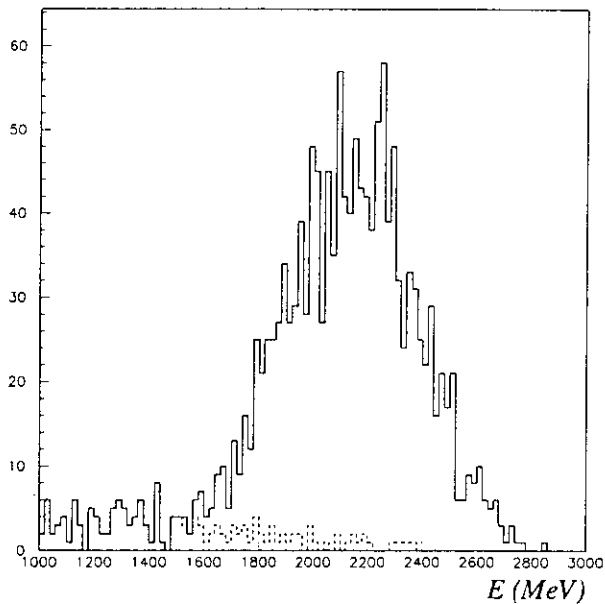
Figure 17: Monte Carlo calculation of the energy spectrum of RCS plus ep\gamma photons (solid) and ep\gamma photons alone (dashed) for E=6 GeV, \theta_{cm}=110^\circ . It has been assumed that backgrounds from ep elastic scattering and \pi^0 photons have been removed by appropriate kinematic cuts. The ratio of ep\gamma to RCS events in the region above 1500 MeV is \approx 0.06 .
