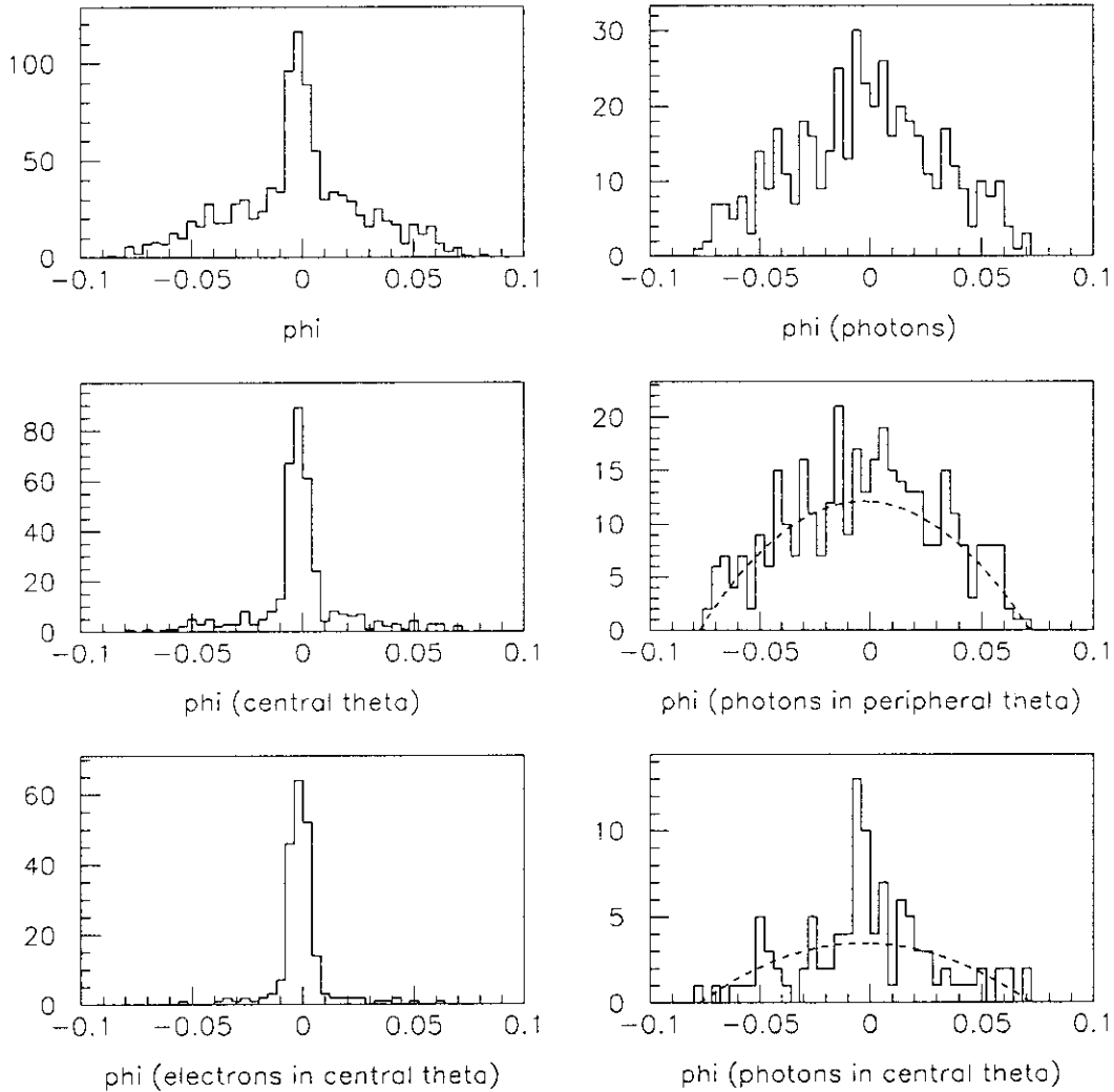
Figure 14: Proof of principle experiment for RCS at 4 GeV and \theta_{cm} = 90^\circ . All panels show the difference between the measured out-of-plane angle \phi in the calorimeter and the reconstructed angle based on the HRS measurement and two-body kinematics. The upper left panel shows all coincidence events. The peak at \phi = 0 is due primarily to ep scattering and secondarily to RCS, whereas the continuum is due to \pi^0 decay photons. For the middle left panel, a cut is made requiring that the in-plane angle \theta be close to that expected for two-body kinematics; this clearly enhances the central peak. The lower left panel in addition demands a signal in the veto detector, thereby selective picking out the ep events. The right panels demand no signal in the veto, thereby picking out photons. An anti-cut on the in-plane angle (middle right) preferentially picks out \pi^0 decay photons, whereas a cut on the in-plane angle (bottom right) selectively enhances the RCS events, with some continuum mixed in. Therefore, the events above the dashed line in the lower right panel represent RCS events, with a 10% contamination due to the inefficiency of the veto detector. The number of RCS events agree within statistics with the Cornell measurements.
