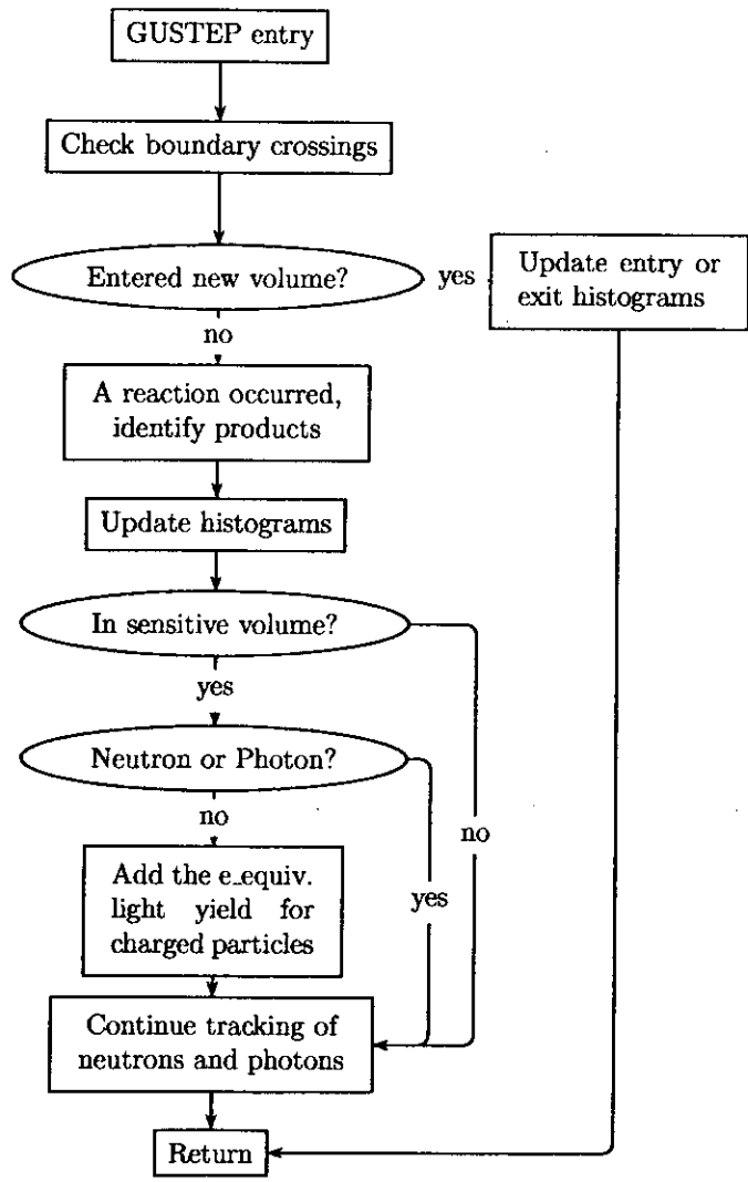
Figure 2: Stream diagram of routine GUSTEP
