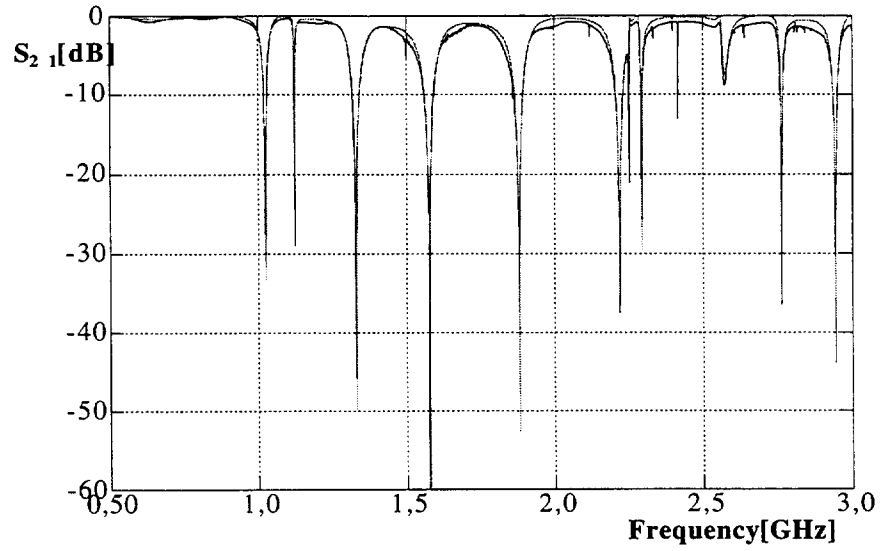
FIG. 4: Transmission scattering coefficient: comparison between theory and measurements.
