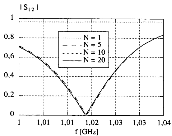
FIG. 3: the convergence of the proposed method around the a resonance.
