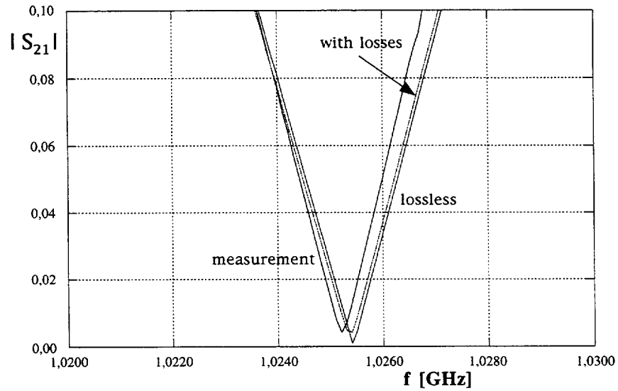
FIG. 5 : Pill-box cavity first resonance: comparison between the measured data and the theoretical ones (with and without losses).
