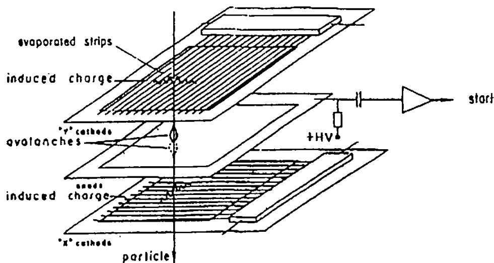
Figure 5.10: Parallel Plate Avalanche Counter schematic diagram.
