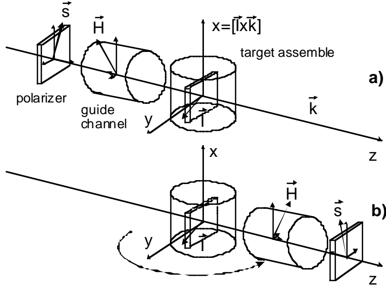
Figure 3.3 : Experimental set-up
