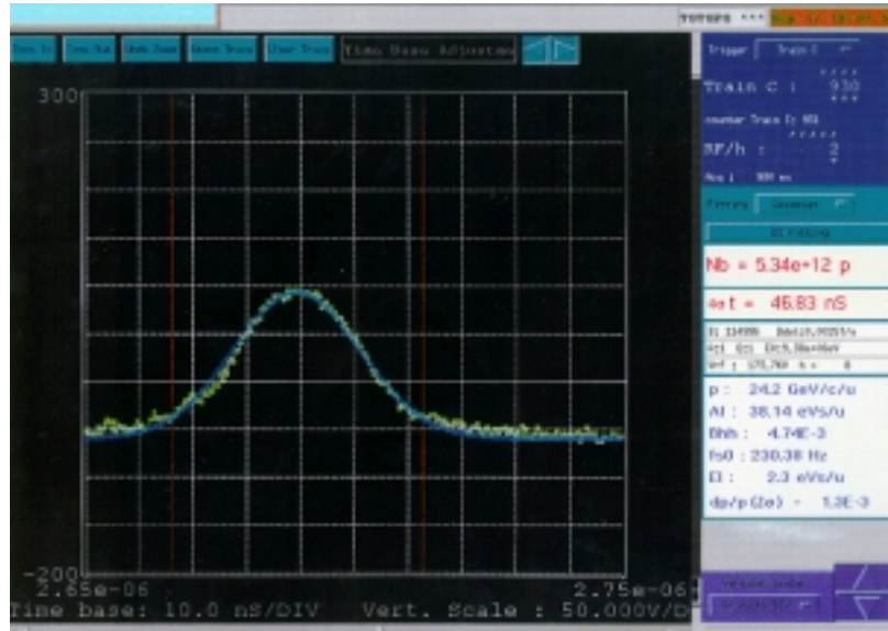
Figure 2.3a: A proton bunch of 0.5 \cdot 10^{13} p/bunch at 24 GeV/c before bunch rotation. The r.m.s. bunch length is \approx 12 ns and \epsilon_1 = 2.3 eVs (time base: 10 ns/div.).
