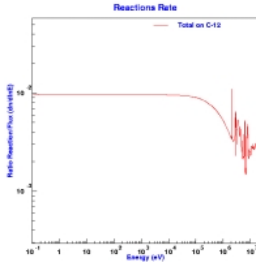
Figure 5.14: Absorption losses in Carbon walls ( \phi=40 cm)
