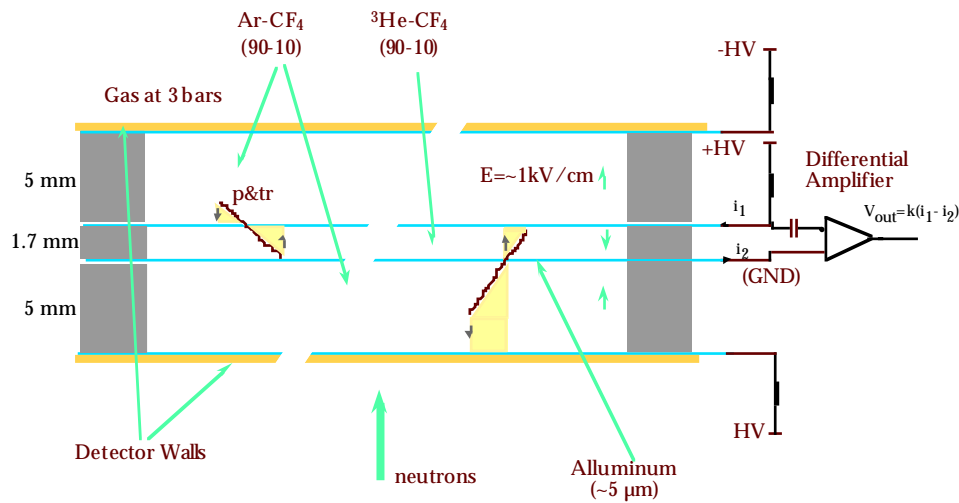
Figure 5.7: Detector lay-out.
