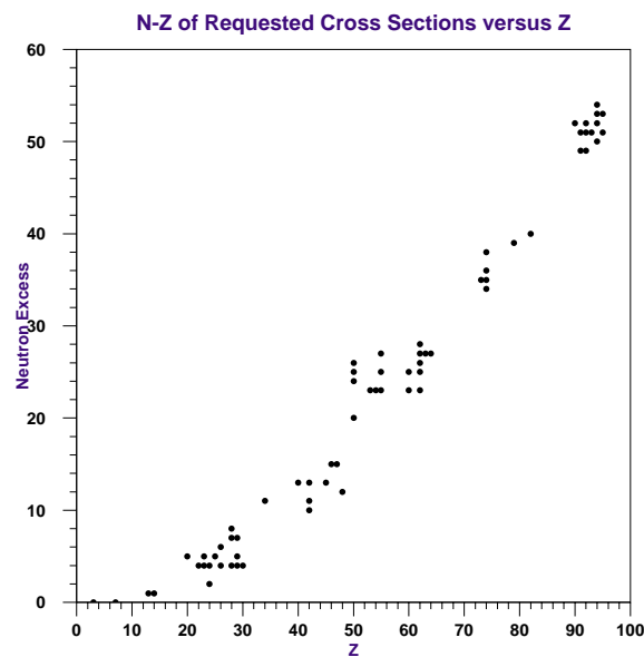
Figure 3.2: The requested isotopes in the OECD/NEA 1998 High Priority List [3.8] as function of the charge number and the neutron excess.
