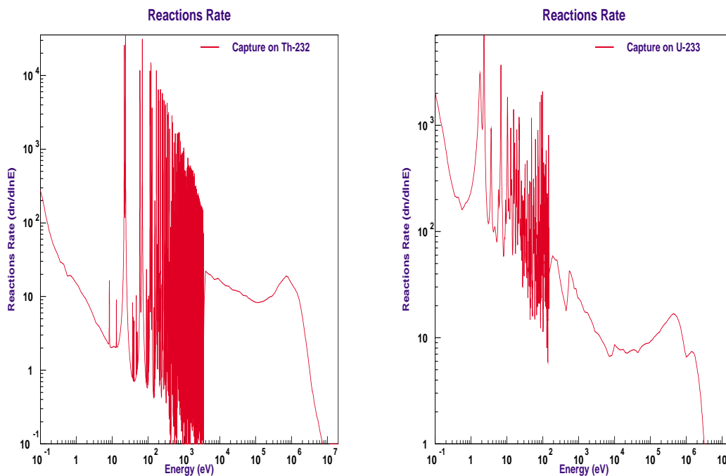
Figure 5.18: The simulated capture rates per day and per energy bin corresponding to a resolution of 2 \times 10^{-4} or 12,000 bins per energy decade.
