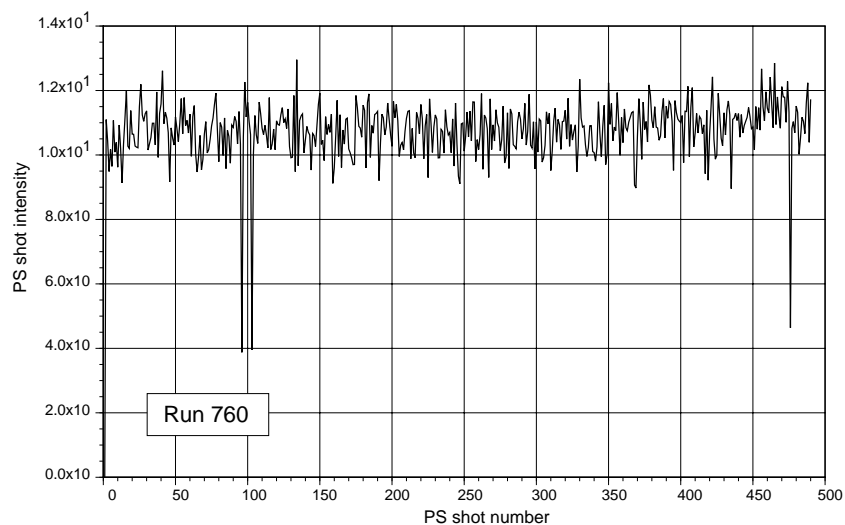
Figure 5.2: Example of measurement of the beam intensity (TARC run 760) showing the number of protons for each PS shot.
