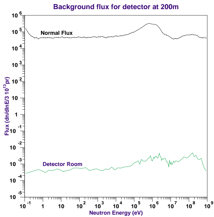
Figure 2.10: Energy of neutrons inside the detector station at 80 m. The spectra at 200 m have the same shape.
