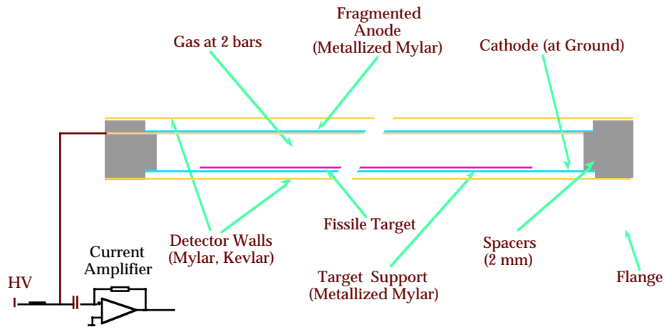
Figure 5.11: Detector geometry
