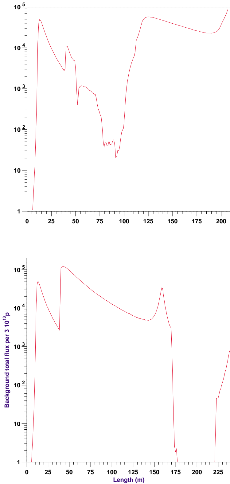
Figure 2.11: The neutron flux along the TOF beam axis for the 80 m and 200 m target station. The flux in the beam tube amounts for the 80 m distance to 1.7 \times 10^7 and for the 200 m distance to 2.7 \times 10^6 neutrons per \text{cm}^2 per high intensity pulse.
