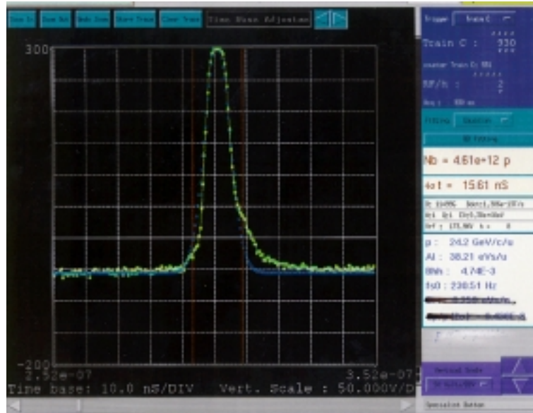
Figure 2.3b: The proton bunch after the bunch rotation in phase space. The r.m.s. bunch length is \approx 4 ns (time base: 10 ns/div).
