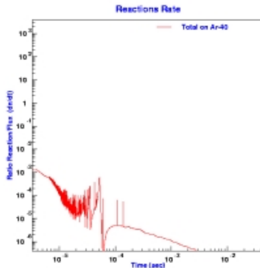
Figure 5.8: Relative reaction rate in 10 mm of Ar.
