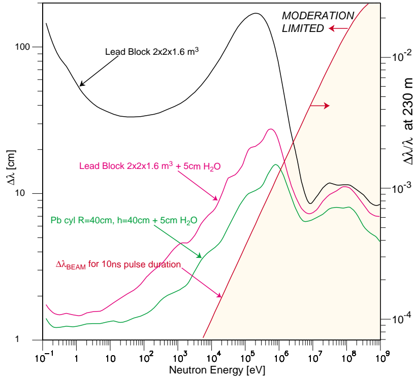
Figure 2.7: The uncertainty in the path \Delta\lambda as a function of neutron energy for various target configurations. The reflected \Delta\lambda uncertainty due to the CERN-PS pulse duration is also shown.
