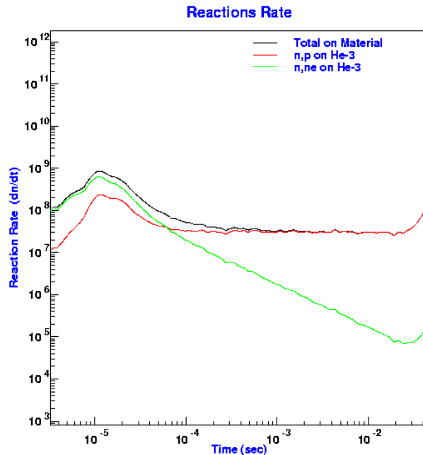
Figure 5.6: Event Rates for (n,p) and elastic reaction in ^3\text{He} (1.7 mm, 3 bar)
