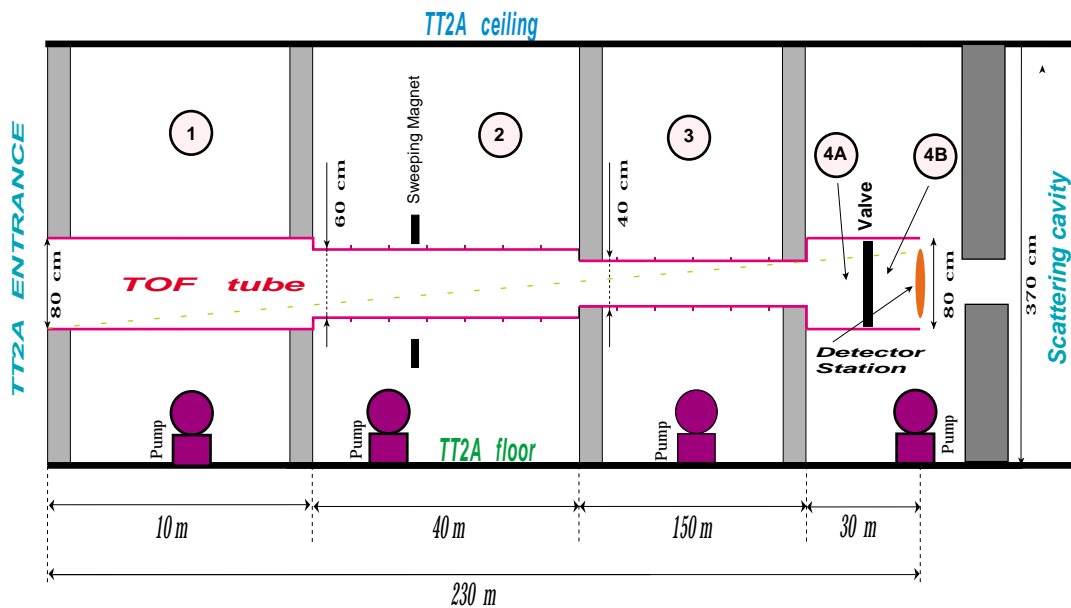
Figure 2.5: Schematic view of the TOF tube.
