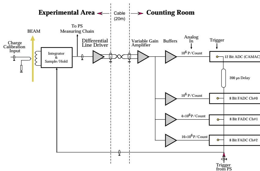
Figure 5.1: Beam Transformer Read-out and Calibration Block diagram.
