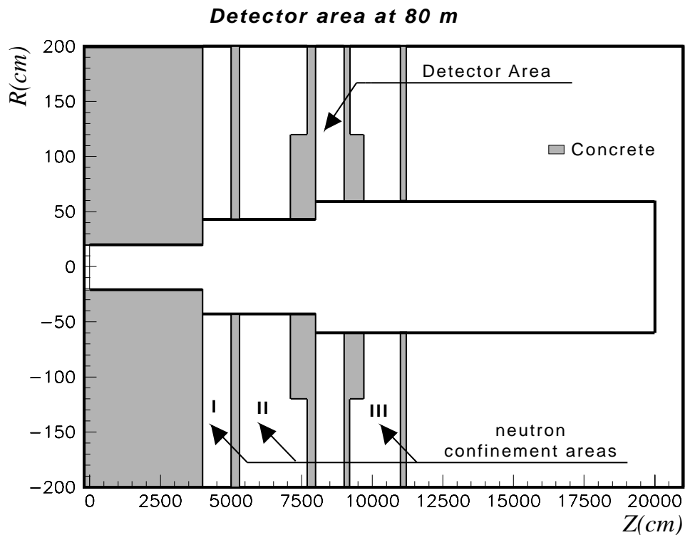
Figure 2.8: Schematic view of the TOF tube geometry and neutron traps before and after the detector station.
