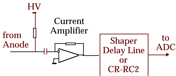
Figure 5.15: Front-end Electronics.
