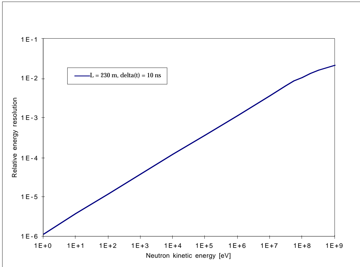
Figure 2.1: Neutron energy relative uncertainty after 230 m of flight path due to 10 ns beam time spread.
