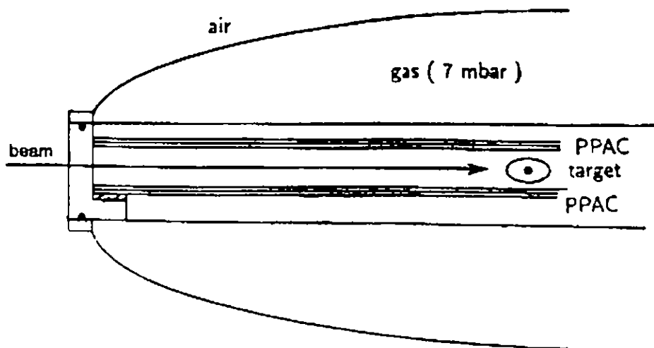
Figure 5.9: Experimental set-up (half part)
