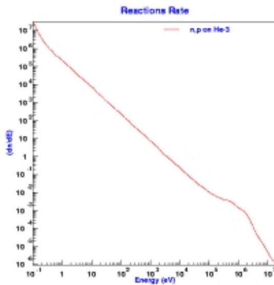
Figure 5.5: Event Rates versus Energy for (n,p) reaction in ^3\text{He} (1.7 mm, 3 bar)
