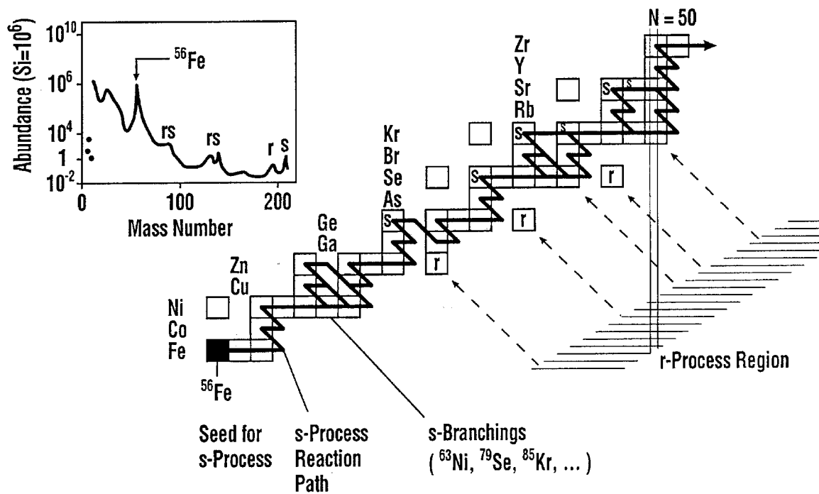
Figure 3.1: An illustration of the neutron capture processes responsible for the origin of the elements between iron and the actinides. The observed abundance distribution in the inset shows characteristic twin peaks. These result from the nuclear properties at magic neutron numbers under typical s- and r-process conditions, an obvious example for the intimate correlation between the observed abundance and the physical conditions during nucleosynthesis.
