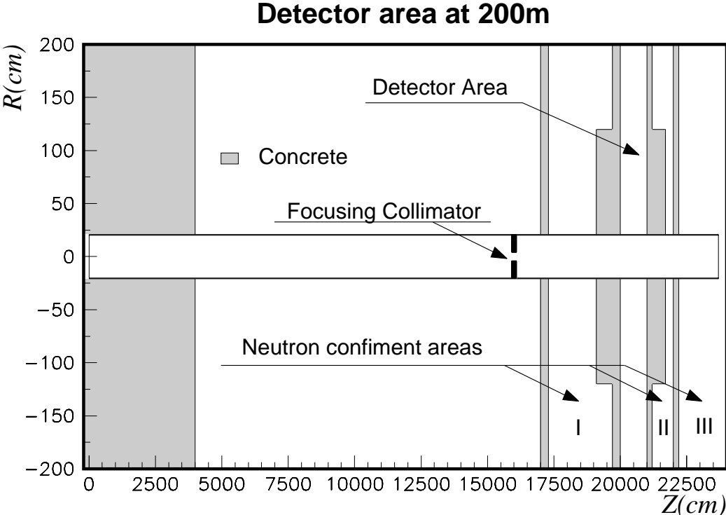
Figure 2.9: Schematic view of the TOF tube geometry and neutron traps before and after the detector station.
