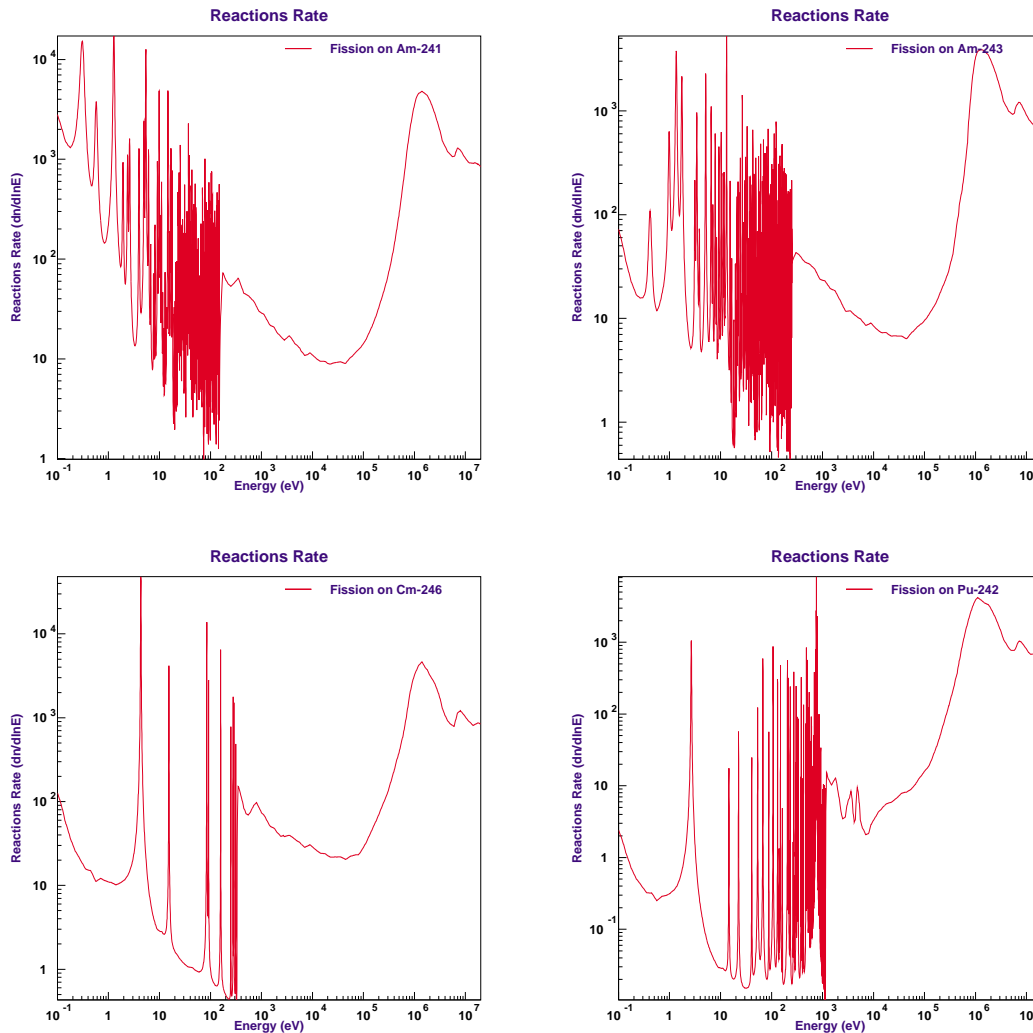
Figure 5.16: The simulated fission rates for a 10 days run and per energy bin corresponding to a bin-width of 0.05 \cdot E_N or 50 bins per energy decade.
