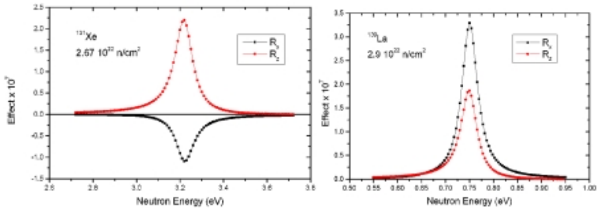
Figure 3.5: The expected magnitudes of the P and T violation effects near the neutron p -wave resonances of 131 Xe and 139 La. See text for details.
