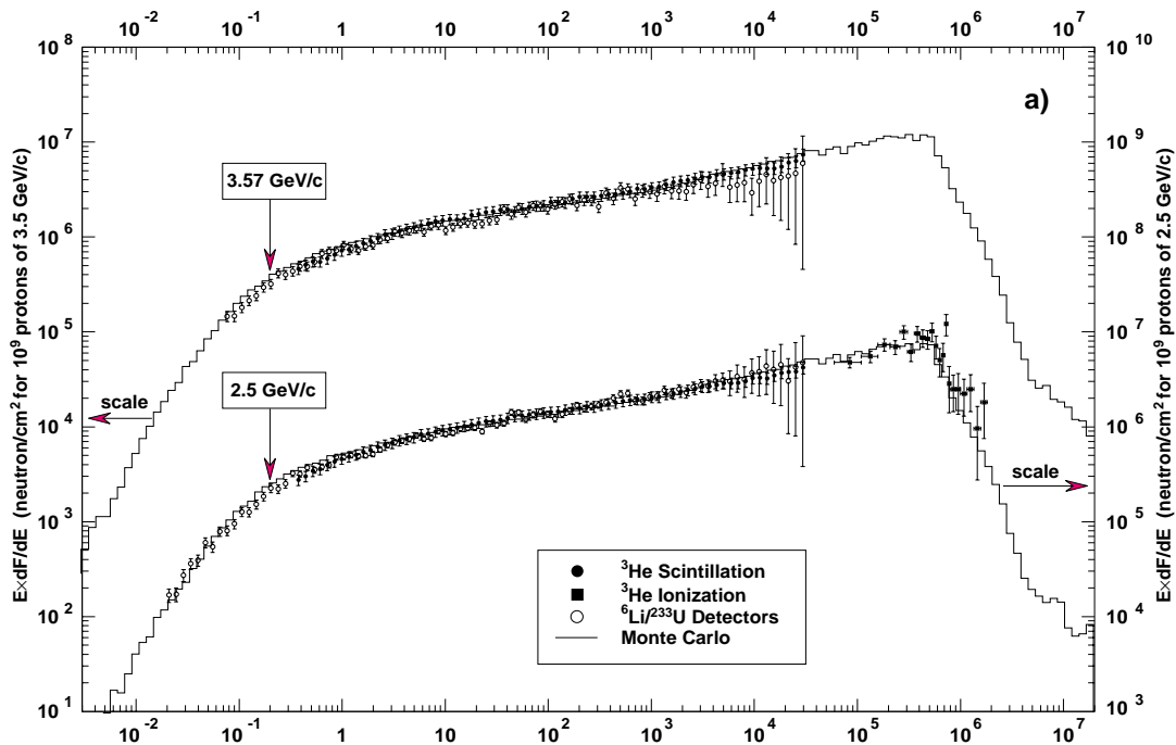
Figure 5.4: Example of TARC measurements of the neutron fluence. E \cdot dF/dE is shown as a function of neutron energy, from 2.5 and 3.57 GeV/c protons in hole number 10 ( Z = 7.5 cm, at a distance of 45.6 cm from the centre of the lead volume). The Montecarlo predictions are shown as histograms. The data are from ^6\text{Li}/^{233}\text{U} detectors (open circles), ^3\text{He} in the scintillation mode (full circles) and ^3\text{He} in the ionisation mode (full squares). The error bars include both statistical and systematic errors added in quadrature;
