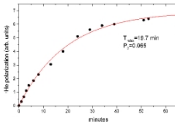
Figure 3.4: Time dependence of the {}^3\text{He} - neutron polariser prototype.
