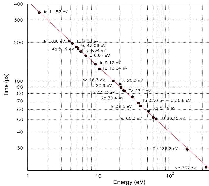
Figure 5.3: Experimental relation from the TARC experiment between time and energy from the multiplier measurements. The curve is a fit to the function K/(t + t_0)^2
