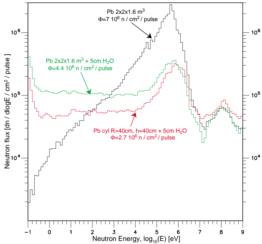
Figure 2.6: Neutron energy spectrum for various lead target configuration, with and without a 5 cm water moderator. The TOF path is 230 m.
