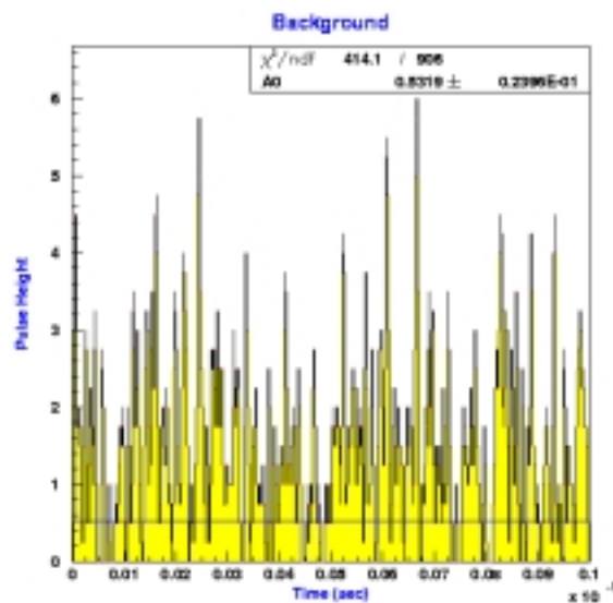
Figure 5.12: Simulation of 5 mCi background pile-up.
