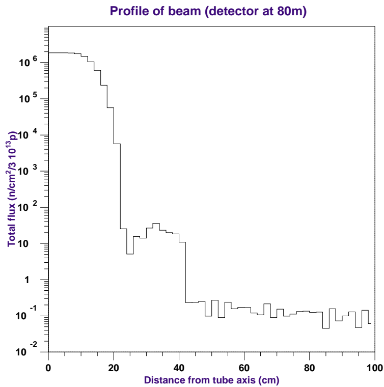
Figure 2 .12: The neutron profile versus the distance of the neutron-tube axis. The halo is evident in the case of 80 m with the use of 2 collimators, where in the 200 m, the profile is more sharp, even with the use of a single collimator.
