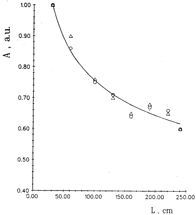
Fig. 6. Ratio of anode amplitudes vs the position of the 55 Fe-source along the straw. (o) – straws with 10 mm in diameter; (Δ) – straws with 6 mm in diameter.
