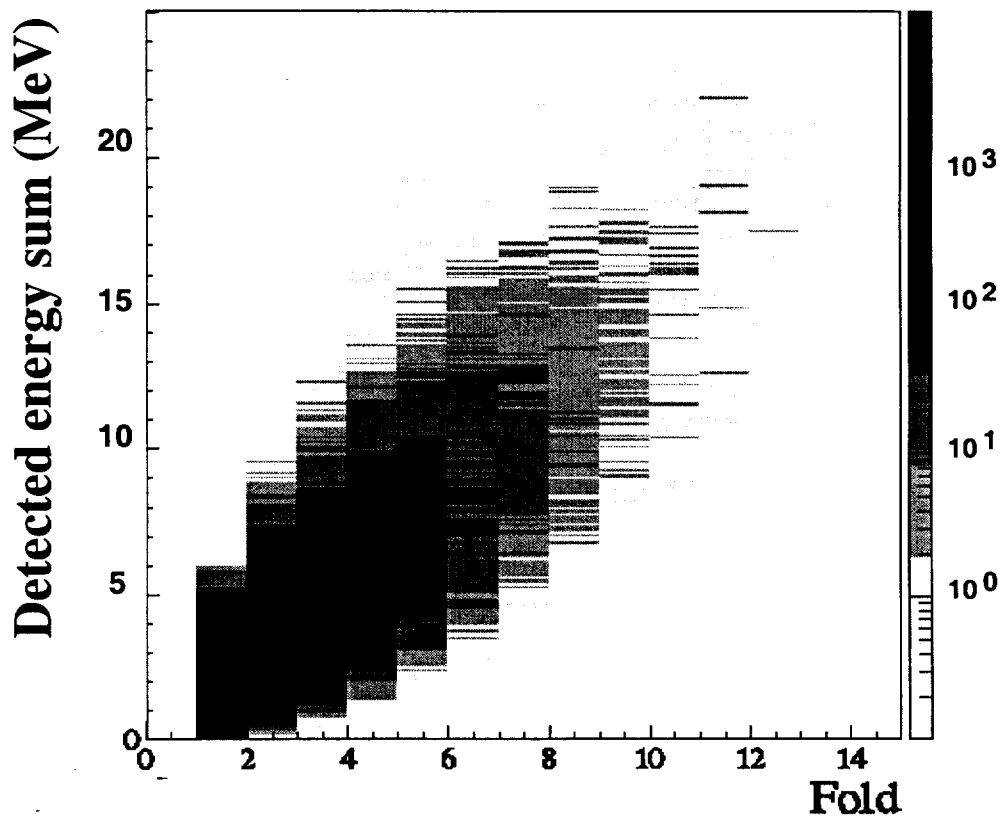
Fig.2 : The BaF2 detected energy sum versus the BaF2 detected fold for ^{32}\text{Mg} fragments. This experimental spectrum is not corrected for the detector efficiency and neutrons contribution. Only the background corresponding to random coincidences was subtracted. The detected average fold and energy sum are respectively 2 units and 2.91 MeV (see text).
