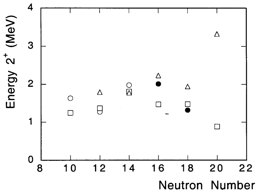
Fig. 6 : Gamma energy in MeV of the first 2^+ levels in isotopic chains : circle = Neon, square = Magnesium and triangle = Silicon. The black points are preliminary new results of this work.
