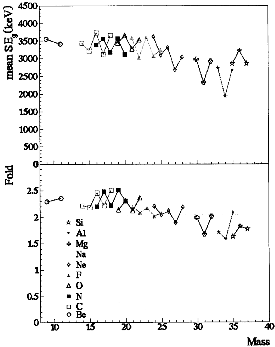
Fig. 3 : Dependence of the detected average BaF2 fold (lower part) and the detected average BaF2 energy sum (upper part) versus fragment products mass. These experimental spectra are not corrected by the detection efficiency. Only the background corresponding to random coincidences was subtracted (see text).
