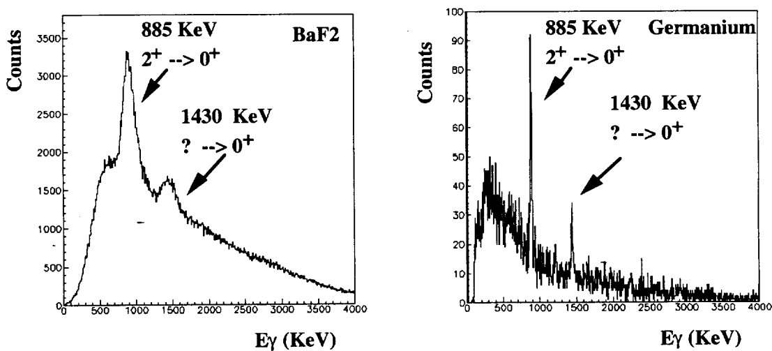
Fig. 4 : Gamma energy spectra of ^{32}\text{Mg} in the \text{BaF}_2 (left) and in the germanium (right).
