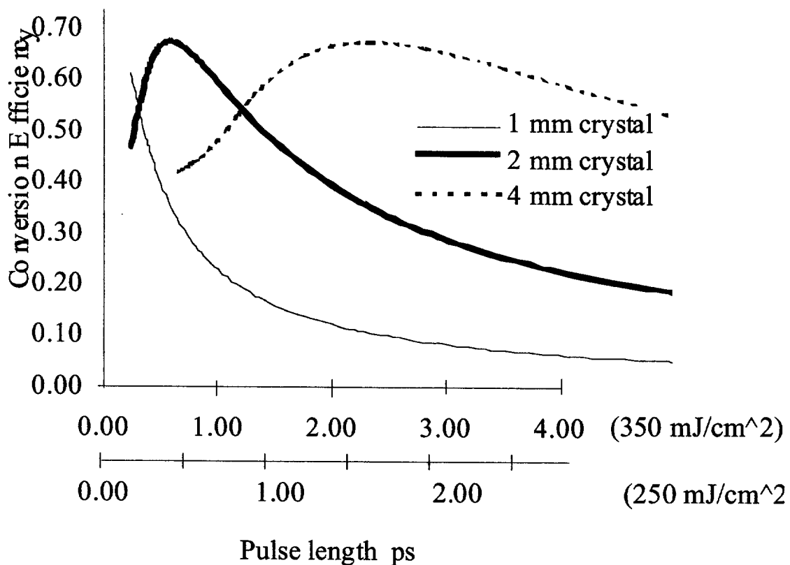
Figure 2. Predicted conversion efficiency for 1, 2 and 4 mm Type 1 frequency crystals as a function of pulse length for incident energy densities of 250 and 350 mJ/cm 2 .
