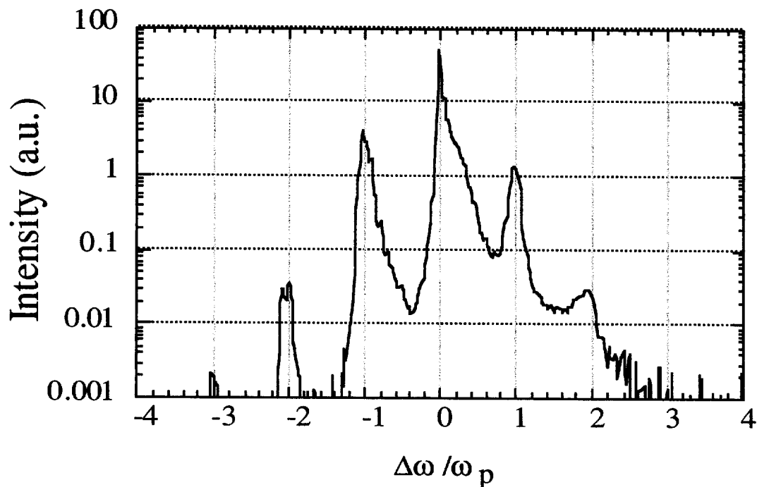
Figure 2. Typical FRS spectra showing cascading. Plasma density was 4.4 \cdot 10^{19} \text{ cm}^{-3} , average |a_0|=0.32 .
