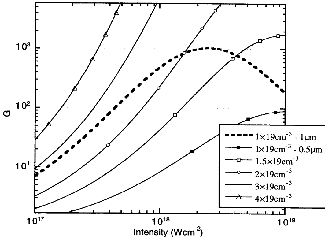
Figure 1. Gain of FRS for either 1 \mu\text{m} at n_e=1\cdot 10^{19}\text{cm}^{-3} or 0.5 \mu\text{m} at a variety of densities as a function of intensity
