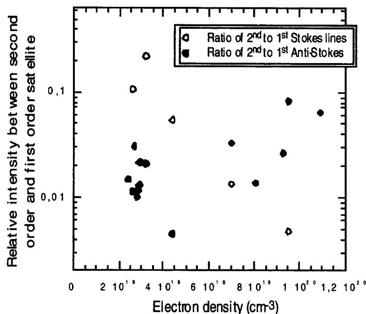
Figure 4. Ratio of 2 nd to first 1 st Stokes and Anti-Stokes lines as a function of density
