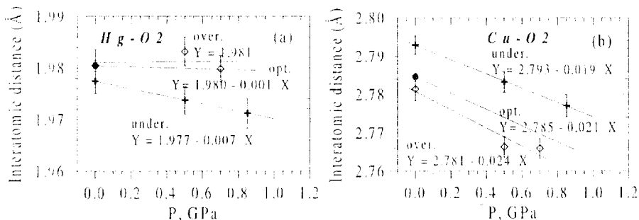
Figure 5. The dependence on pressure of the Hg-O2 (a) and the Cu-O2 (b) apical distances.
