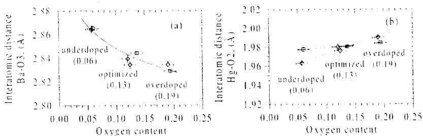
Figure 3. Dependence of the Ba-O3 (a) and Hg-O2 (b) interatomic distances on the oxygen content \delta . The marks are the same as for Fig.2.
