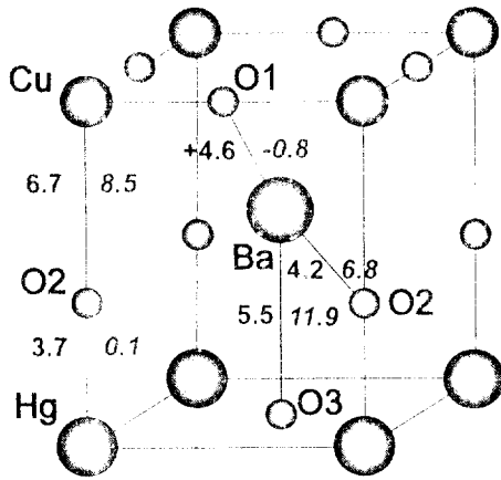
Figure 8. Schematic representation of the Hg-1201 structure. The values of the compressibilities of the selected bond distances are written on the left for the underdoped sample, and on the right for the overdoped sample.
