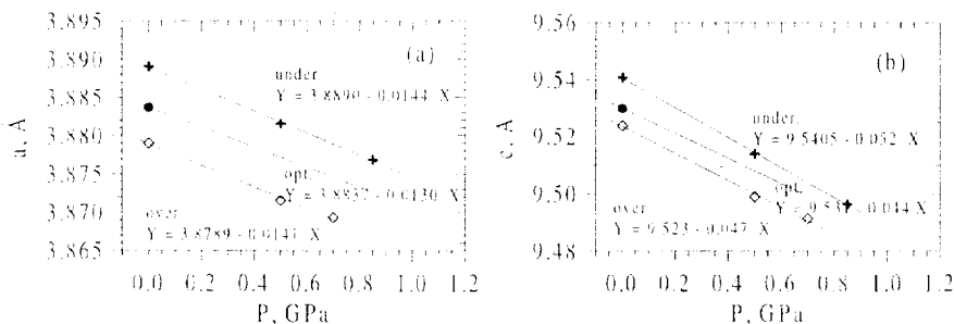
Figure 4. The unit cell parameters of Hg-1201 as a function of external pressure for three samples. For the optimally doped state the point measured at P=0 is shown together with the line slope determined in 13 . The experimental errors are smaller than the symbols.
