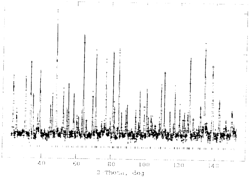
Figure 1. The diffraction pattern of the sample C, measured at D2B at a pressure P=0.5 GPa and analyzed with the Rietveld method.
