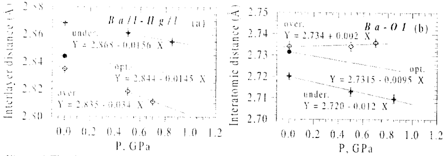
Figure 6. The distances between the Ba-layer and the Hg-layer (a) and between Ba and O I atoms (b) as a function of pressure.
