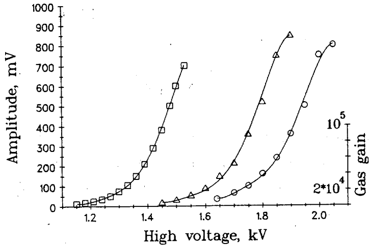
Fig. 2. Gas gain and amplitude of the anode signals depending on high voltage.
