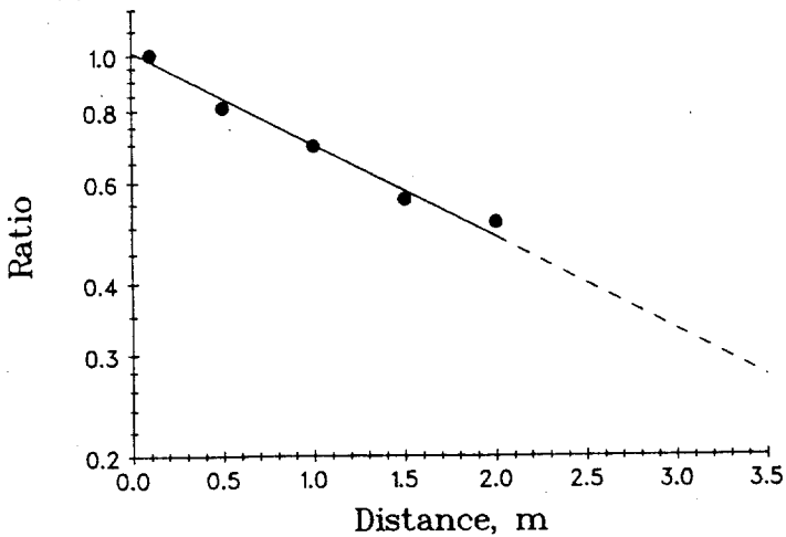
Fig. 3 The attenuation length is obtained from the curve showing the ratio of the amplitude. Width of the strips is 8 mm, R_{str} is 3.1 \text{ Ohm} / \text{mm}^2 .
