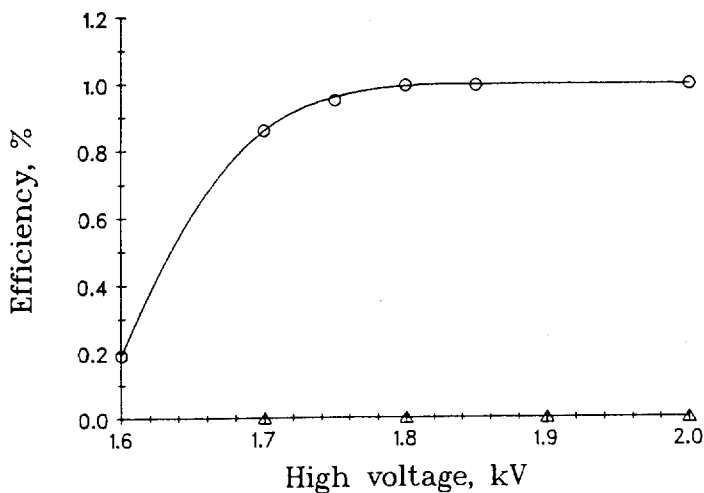
Fig. 6 Efficiency of the \beta - particles registration by the straw with the inner mylar tube.
