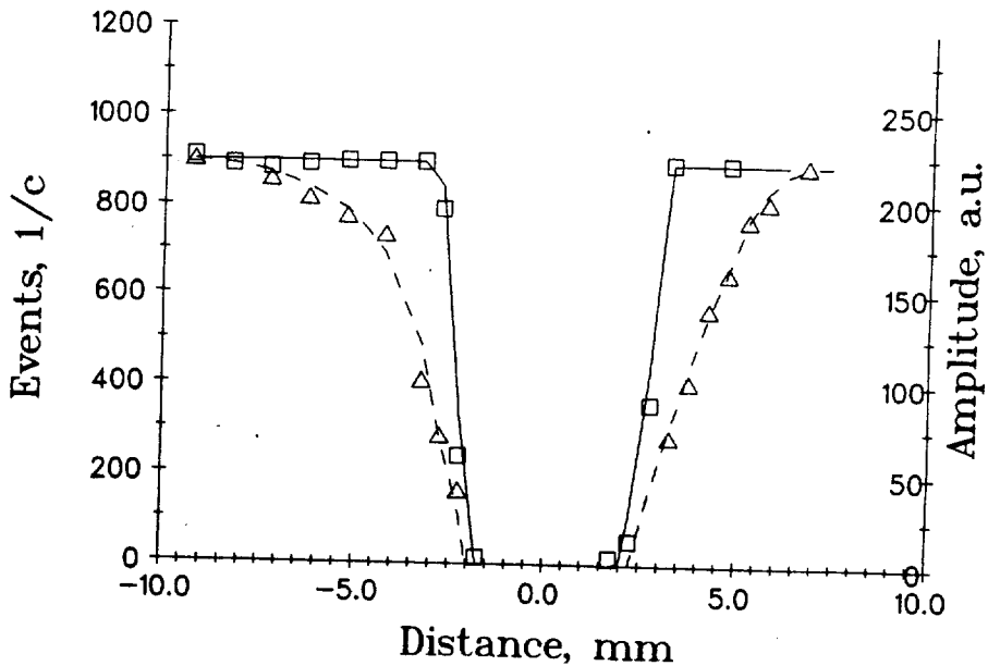
Fig. 7 Count curve (solid curve) dependence on the displacement of the source position from the center of the spacer installed in the straw with the diameter of 10 mm. The ^{55}\text{Fe} source was collimated. The width of the collimator was about 3 mm.
