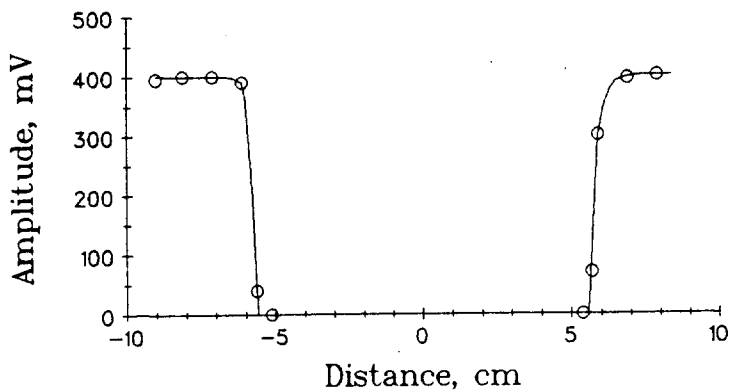
Fig. 5 Amplitude of the pulses vs the position of the ^{55}\text{Fe} along the straw. The straw with the diameter of 10 mm contains the inner mylar tube with the length of nearly 10 cm.
