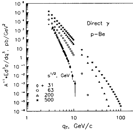
Figure 2. Inclusive cross section of direct photon production in pBe collisions as a function of transverse momentum q_{\perp} for different cms energies \sqrt{s} = 31, 63, 200 and 500 GeV at an angle of \theta = 90^{\circ} . The experimental data on cross section ( \diamond - E706) are taken from [39].
