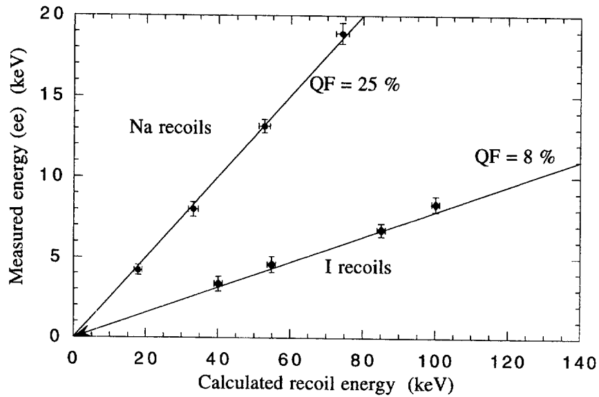
Figure 2: Measured recoil energy in NaI(Tl) as a function of the true real kinetic energy of the recoils on Na and I nuclei.
