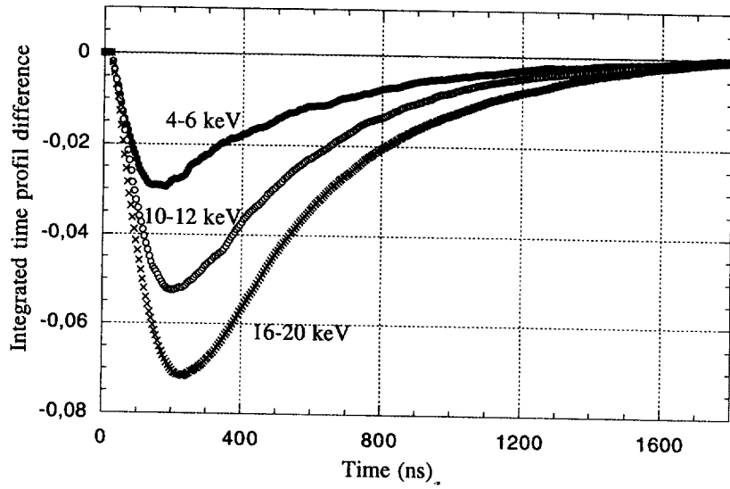
Figure 11: Integrated time profil difference between Compton and Na recoils (neutron source, 9.7 kg crystal).
