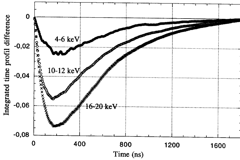
Figure 5: Integrated time profil difference between Compton and Na recoils (neutron beam, 1" by 1" crystal) for 3 energy bins 4-6, 10-12 and 16-20 keV. The amplitude of the difference (defined at 200 ns) increases with energy.
