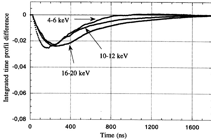
Figure 13: Integrated time profil difference between Compton and betas from an external ^{57}\text{Co} source.
