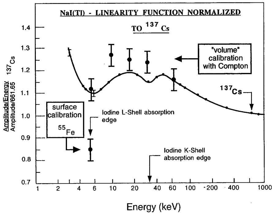
Figure 10: Variation with energy of the response (surface and volume for low energy) of NaI(Tl).
