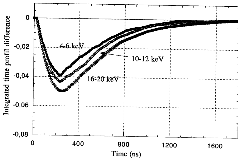
Figure 12: Integrated time profil difference between Compton and X rays from an external ^{241}\text{Am} source.
