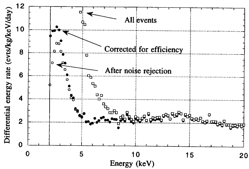
Figure 15: Low energy spectra of data acquired during 83 days : raw rate, after cleaning of noise, and correction for event losses.
