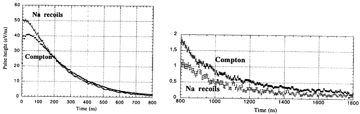
Figure 4: Reference pulses for Compton and Na recoil events for the 12-14 keV equivalent electron energy bin up to 1800 ns. The integrals up to 1800 ns are normalised to the same area.
