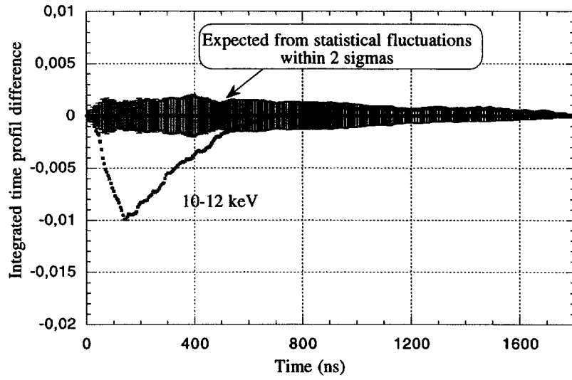
Figure 17: Integrated time profil difference between Compton and data together with the expected statistical fluctuations zone for the 10-12 keV energy bin.
