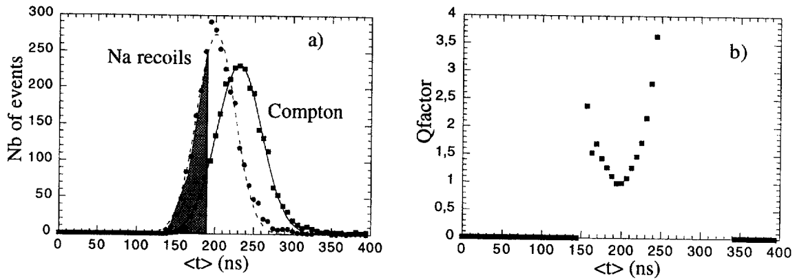
Figure 6: a) distribution of the \langle t \rangle variable for the recoils and Compton populations in the 12-14 keV bin .The 190 ns cut gives \alpha=0.43 and \beta=0.11 , b) variation of Q with the \langle t \rangle cut.
