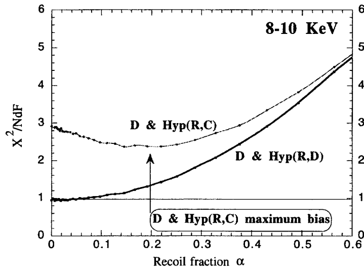
Figure 18: Variation of \chi^2 between the Data population shape and hypothesis built of mixtures of populations R (Nuclear recoils) and C (Compton), D (Data) for the 8-10 keV energy slice. See text for details. When comparing Data and a mixture of Recoils/Compton no value of recoil fraction provides a \chi^2 close to 1.
