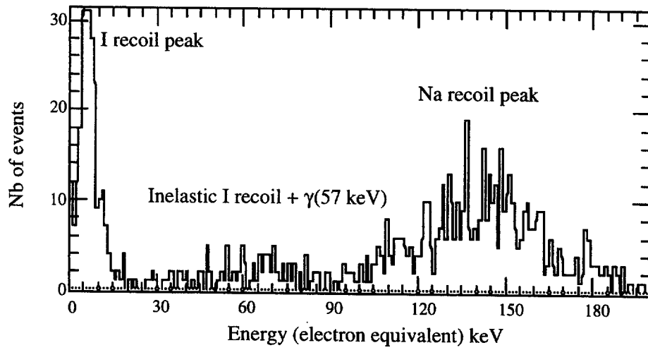
Figure 1: Energy (electron equivalent) distribution of the recoil events selected at a fixed neutron scattering angle. Peaks due to Iodine and Sodium recoils can be easily observed.
