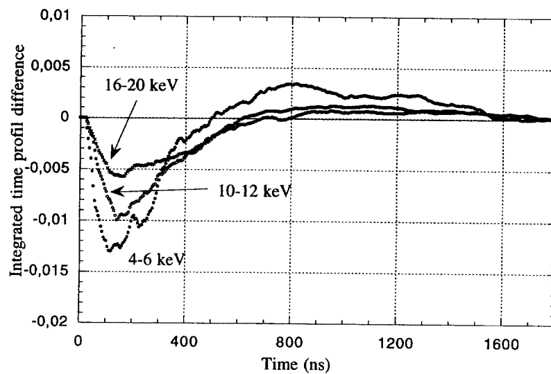
Figure 16: Integrated time profil difference between Compton and data acquired during 83 days.
