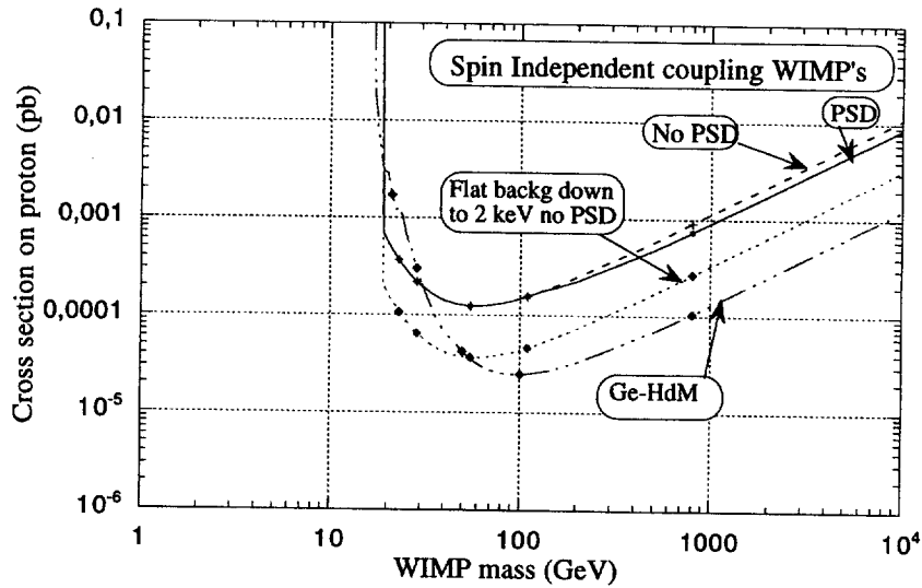
Figure 19: Exclusion diagrams in the WIMP Mass/(WIMP-nucleon cross section) plane, for Spin Independent coupling WIMP's. Little improvement comes from the PSD (curves "PSD and "No PSD") because recoils occur mostly on Iodine, at energies below 4 keV, where the PSD is not efficient. The sensitivity to the rate at the threshold is illustrated by the curve "flat back down to 2 keV" obtained by extrapolating the rate of 2.2 evts/kg/keV/day at 6 keV constant down to 2 keV (See text). Also shown for reference is the exclusion curve from the Heidelberg-Moscow experiment [17].
