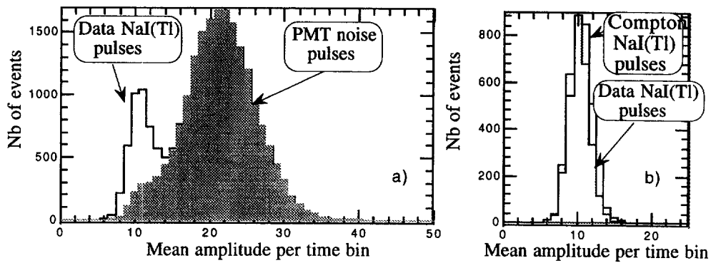
Figure 14: Noise discrimination parameter (mean amplitude per time bin) distributions for the 2-5 keV bin a) all events, noise (shaded) and data (blank) selected events b) selected data and compton events.
