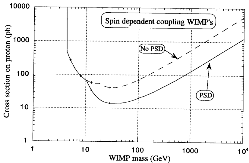
Figure 20: Exclusion diagrams in the WIMP Mass/(WIMP-nucleon cross section) plane, for Spin Dependent coupling WIMP's. Here is clearly seen the importance of the PSD.
