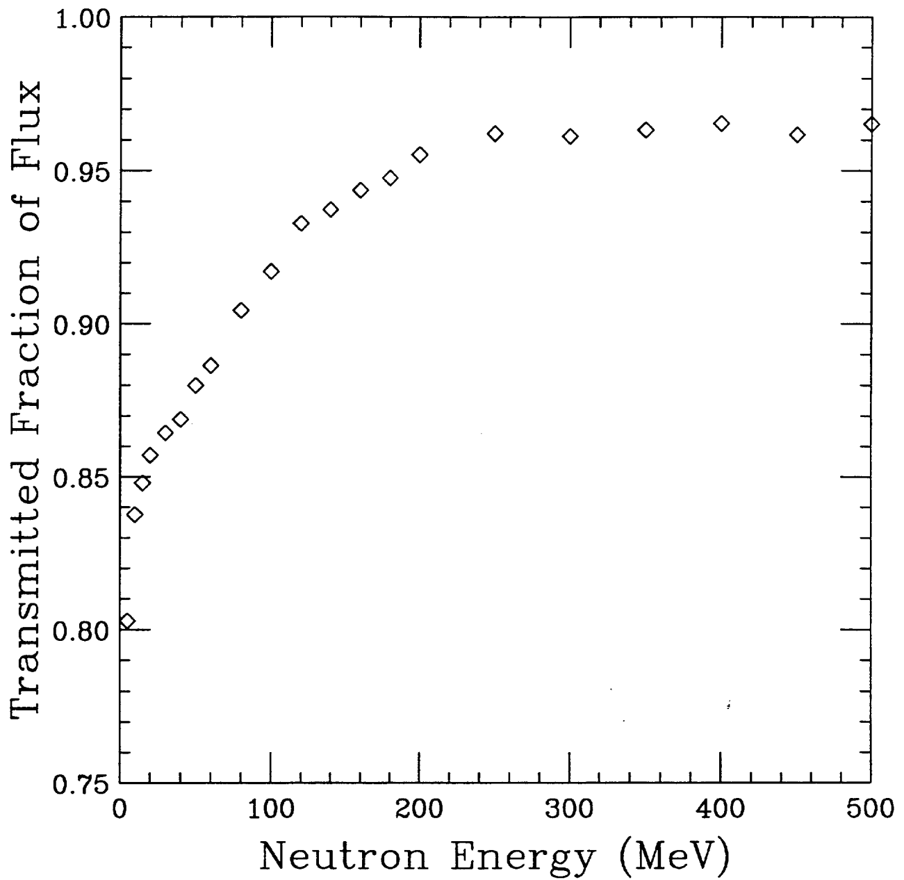
Fig. 5 - Fraction of the incident neutron flux transmitted to detector #9, as a function of energy. Flux lost is due to outscattering by materials between the target and the detector.
