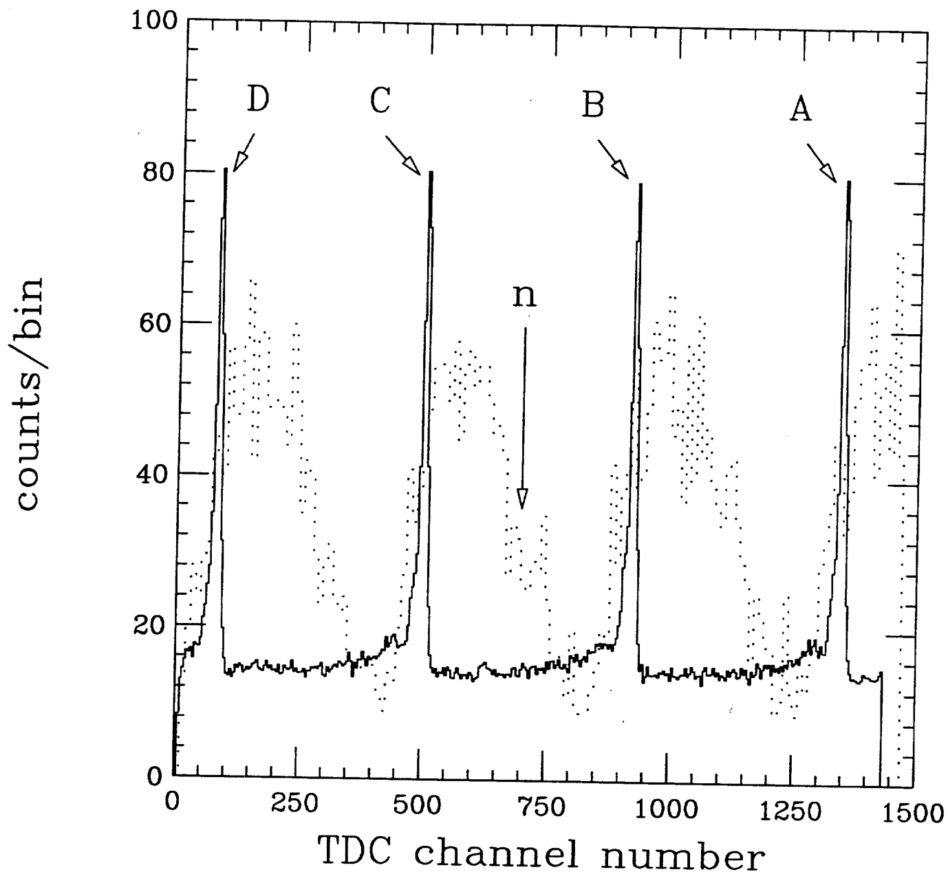
Fig. 2 - Time-to-digital convertor (TDC) spectrum for detector #33. Time increases from right to left. Gamma-ray events are indicated with the solid histogram, and neutron events are indicated with the dotted histogram. The peaks labeled A, B, C, and D are due to prompt gamma rays created by successive beam bursts striking the target.
