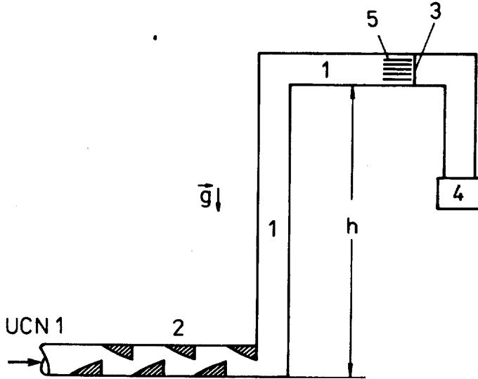
Fig.1 The scheme of the experiment for the search for the anomalous transmission of UCN through metal foils: 1. Vacuum stainless steel neutron guides \phi 60mm 2. Spectral filter for UCN 3. Foil 4. Detector of UCN ( ^3He proportional counter) 5. Additional UCN scatterer.
