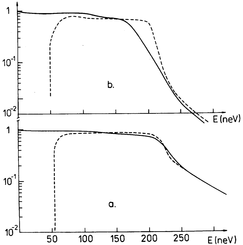
Fig.2. Results of Monte Carlo simulations of UCN detector ( ^3\text{He} counter with aluminium membrane) efficiency for two different positions of the detector in respect to the foil position: dashed line - horizontal one, and solid line - at the level 60\text{cm} lower, and for two different probabilities \eta of UCN diffuse reflection during the transport from the foil to detector through the stainless steel neutron guide with diameter 60\text{mm} : a - \eta = 0.1 ; b - \eta = 0.5 .
