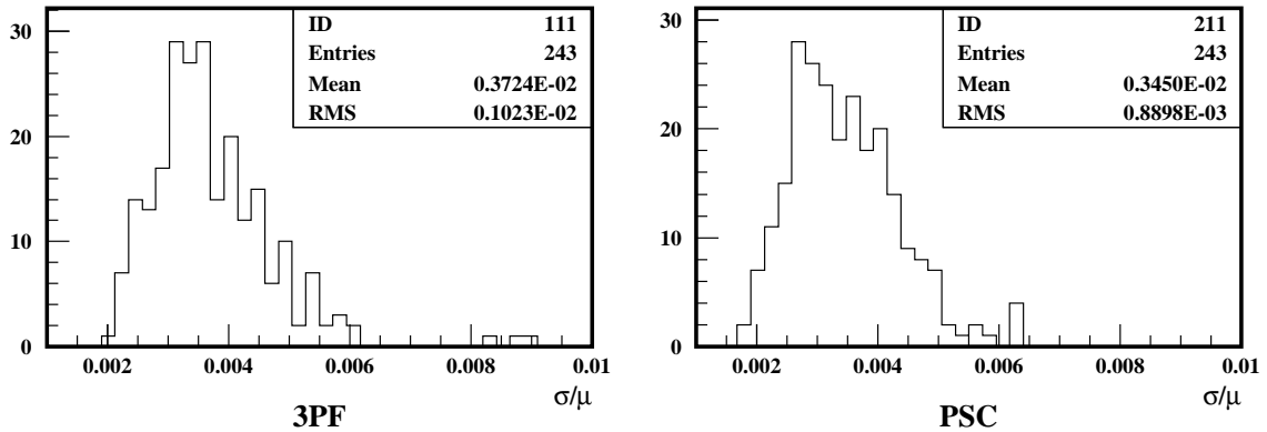
Figure 14: Resolution for all channels with adders of length 11 using three parameter fit (left) or pulse shape comparison (right). PPG pulses below an amplitude of 0.07 pC have been cut.
