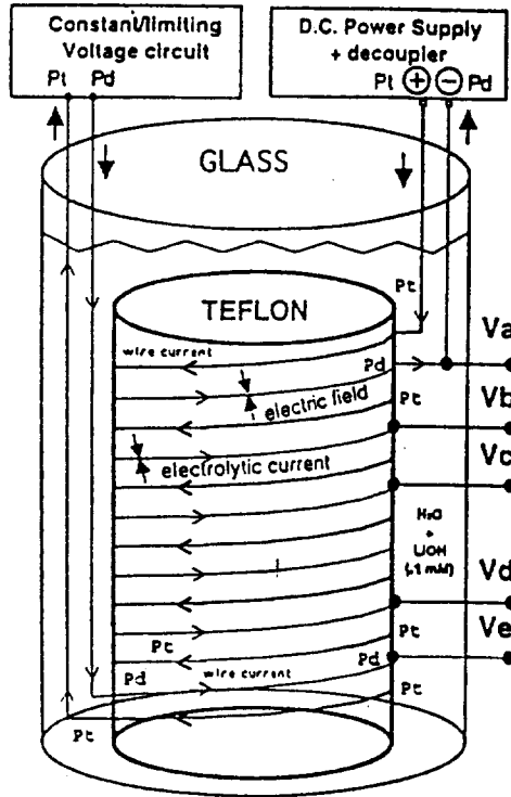
FIG. 1 – Electrolytic Device: Pd cathode and Pt anode wires are twisted around a PTFE cylinder. The electrolytic solution is very diluted. Along the Pd wire, some electric sensors are pointed
