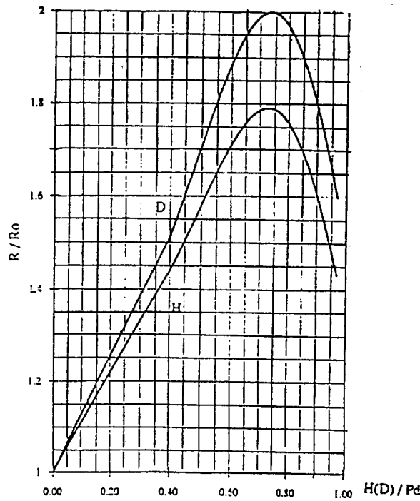
FIG. 2 – D/Pd Resistance curve: in this curve the resistance almost linearly increases with the loading. At the D/Pd=0.75 the normalized resistance has the peak value of 2 (1.8 for H/Pd). The curve is known up to the point D/Pd=0.95 and R/R 0 =1.6.
