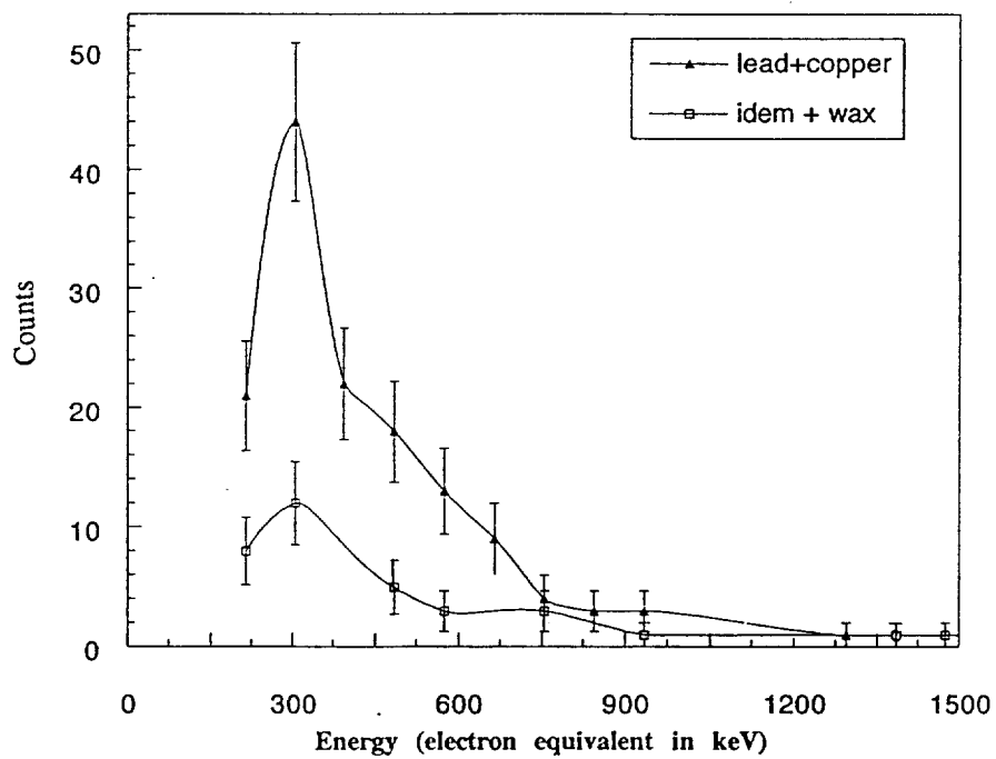
Fig. 6. Experimental neutron energy spectrum, in electron equivalent energy, for the first and second phase.
