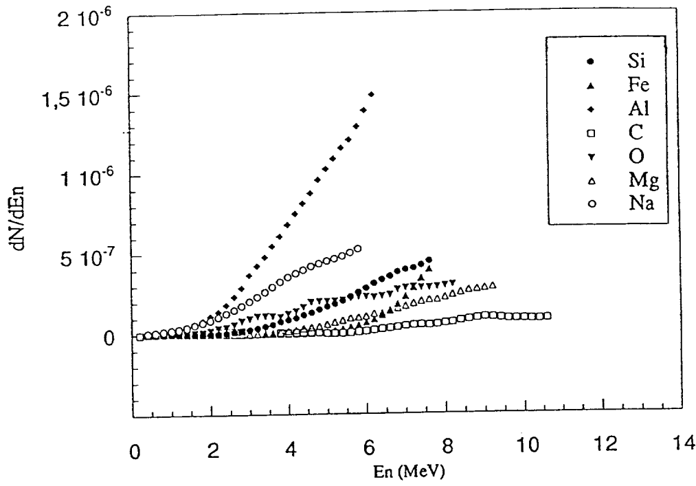
Fig.9. Neutron production rate dN / dE_n per \alpha -particle, element per element, obtained as a function of neutron energy.
