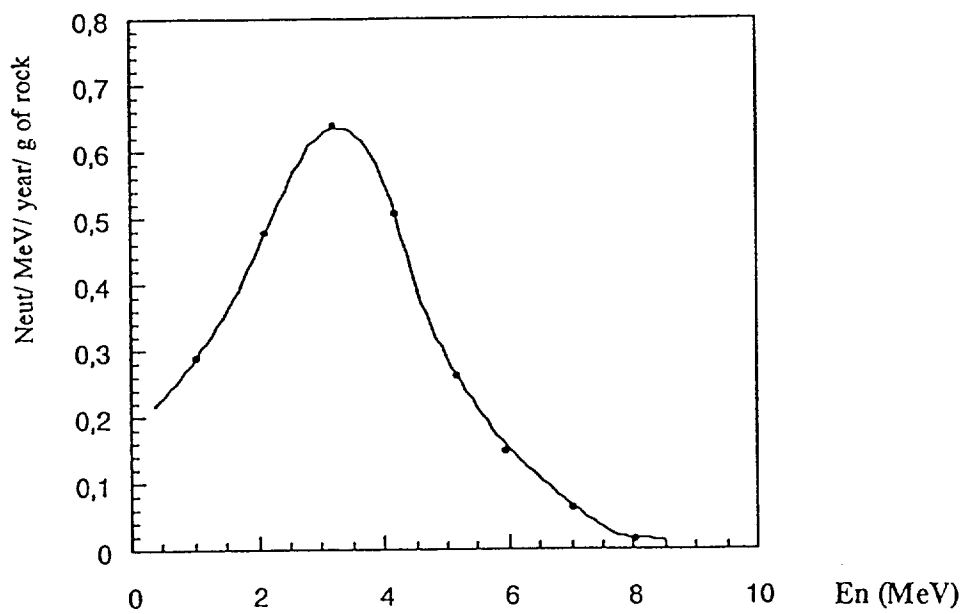
Fig. 11. Neutron energy distribution in the rock, from the spontaneous fission contribution plus the (\alpha,n) reactions contribution.
