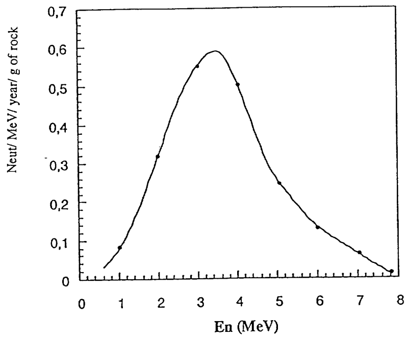
Fig. 10. Neutron energy distribution obtained by (\alpha,n) reactions in the rock.
