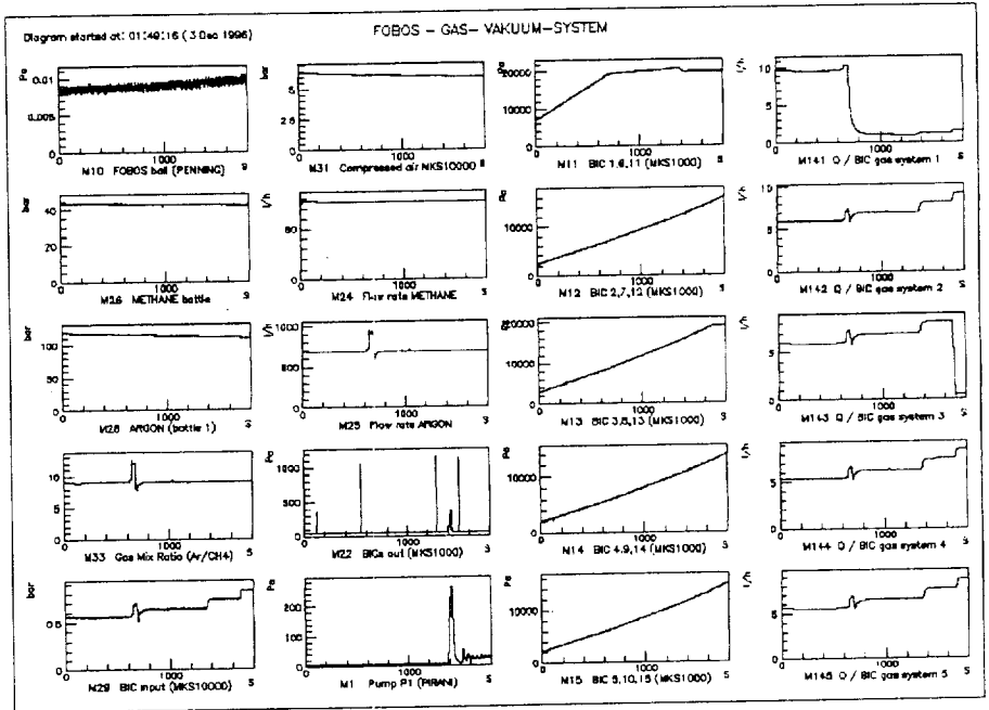
Fig. 16 Snapshot of the on-line protocol of the operation of the evacuation and gas-supply system generated on the SUN SparcSLC terminal.
