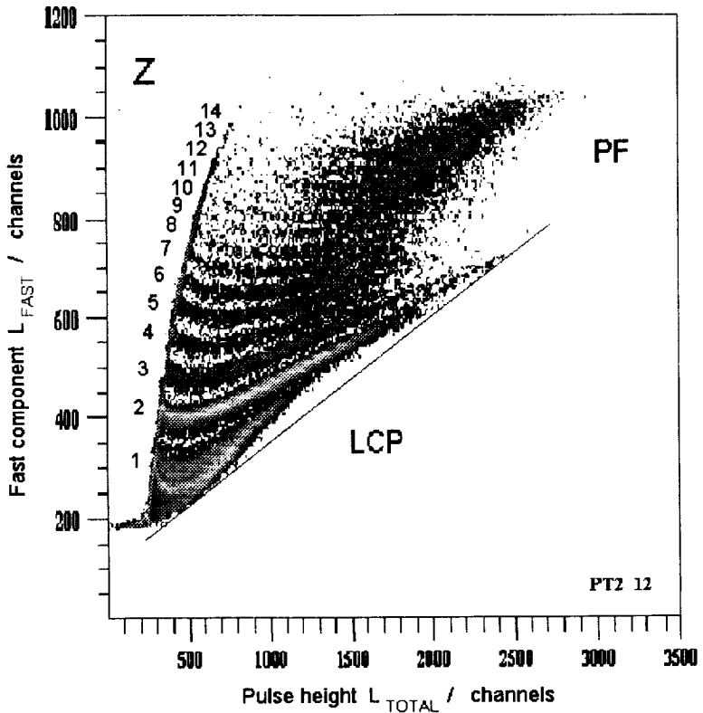
Fig. 21 Charged - particle identification matrix ( L_{\text{FAST}} versus L_{\text{TOTAL}} ) measured by a phoswich detector of the forward array at \theta = 8^\circ for the reaction ^{40}\text{Ar} (36 AMeV) + ^{248}\text{Cm} (PF - projectile-like fragments, Z - atomic number of charged particles identified).
