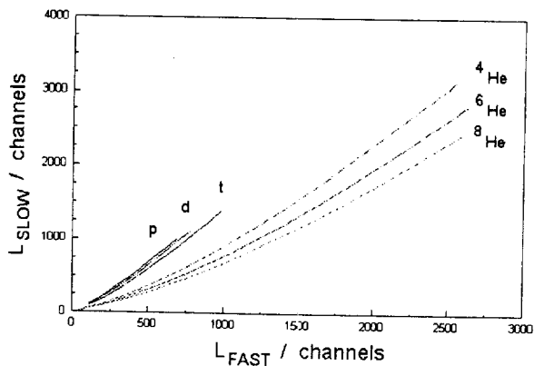
Fig. 31 Simulation of the particle branches of an LCP-identification matrix for CsI(Tl) as it follows from the application of the pulse-shape analysis method (a).
