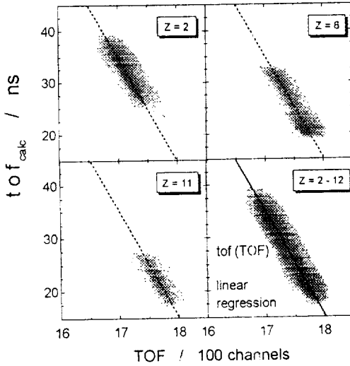
Fig. 30 Absolute calibration of the TOF-scale. The measured values (TOF) are compared with those calculated by eq. 2 ( tof_{calc} ) for selected events generated by particles with known parameters. A linear regression analysis delivers the curve tof(TOF) for the determination of the constant TOF_0 of eq. 3.
