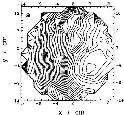
Fig. 5 Contour plots of calibrated time - of - flight signals of a PSAC with a step of 0.05 ns.
