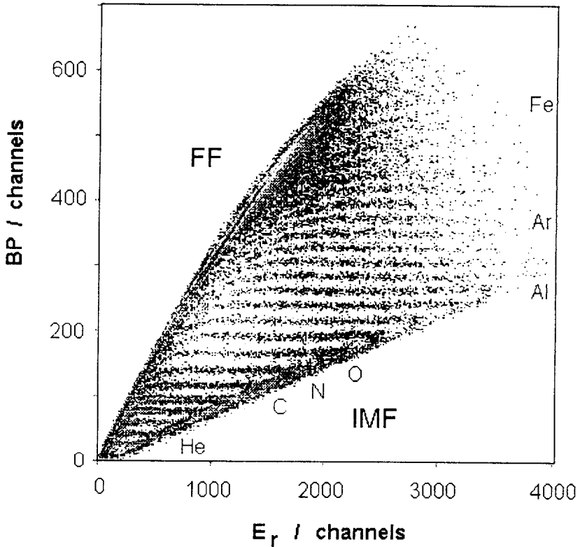
Fig. 13 Bragg peak-height (BP) versus residual energy ( E_R ) scatterplot of inclusive fragments measured by a BIC for the reaction ^{14}\text{N} (34 AMeV) + ^{197}\text{Au} . Particle branches of several resolved elements are indicated. (FF - fission fragments; IMF - intermediate mass fragments)
