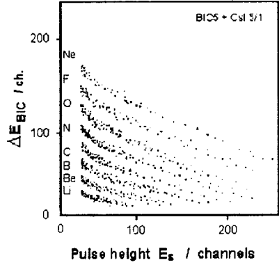
Fig. 20 Charged-particle identification matrix measured by application of the \Delta E -E-method. ( \Delta E_{BIC} - energy loss in the BIC; E_S - residual pulse-height of the fast part ( L_{FAST} ) of the CsI(Tl)-detector signal)
