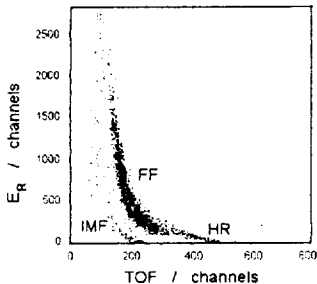
Fig. 9 E_R versus TOF scatterplot measured by a gas - detector module for the reaction ^{14}\text{N} (53 AMeV) + ^{197}\text{Au} . (Note that the time interval of the registration of heavy residues is considerably shorter than in the case shown in fig. 8.)
