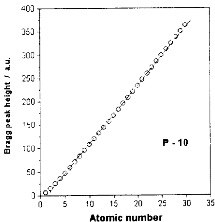
Fig. 24 Dependence of the Bragg peak-height (BP) on the atomic number ( Z ) of charged fragments stopped in a P-10 gas-mixture. The calculated values (eq. 1) are indicated by open circles. The line results from a linear regression analysis. It is defined by the expression
