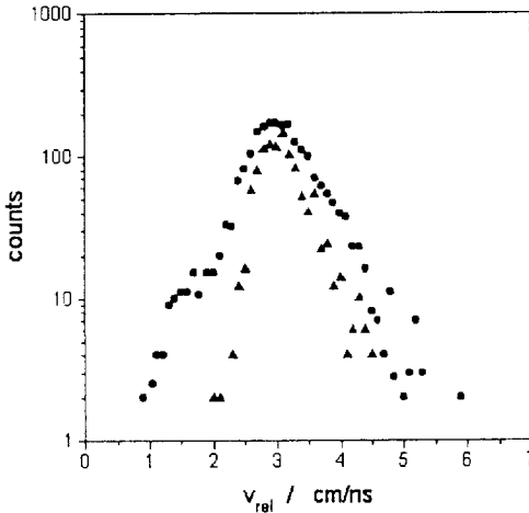
Fig. 38 Relative velocity ( v_{rel} ) distribution of fragments from binary and ternary decays of the composite system created in the reaction ^{14}\text{N} (34 \text{ AMeV}) + ^{197}\text{Au} . (full triangles: v_{rel} between fragment pairs in very asymmetric binary decays; full circles: v_{rel} between the IMF accompanying fission and the c.m. of the fissioning system in ternary decays)
