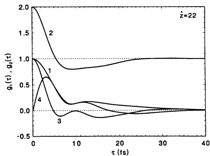
Fig. 5.22. The first and the second order time correlation functions, |g_1(\tau)| (curve 1), g_2(\tau) (curve 2), \text{Re}(g_1(\tau)) (curve 3) and \text{Im}(g_1(\tau)) (curve 4) of the radiation pulse at different reduced length of the FEL amplifier operating in nonlinear regime. Calculations have been performed with nonlinear simulation code over 10^4 independent statistical events.
