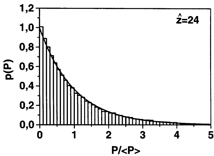
Fig. 5.30. Histograms of the probability density distribution, p(P) , of the instant output power at different reduced length of the FEL amplifier. Calculations have been performed with nonlinear simulation code over 10^4 independent statistical events. \langle P \rangle denotes the average power. Solid curve represents the negative exponential distribution p(P) = \exp(-P/\langle P \rangle) .
