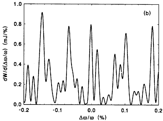
Fig. 5.2. Typical spectrum of the radiation pulse (one shot) at the reduced length of the FEL amplifier \hat{z} = 11 . Graph (a) is plotted over the full spectrum width and graph (b) presents enlarged fraction of graph (a). Calculations have been performed with linear simulation code.
