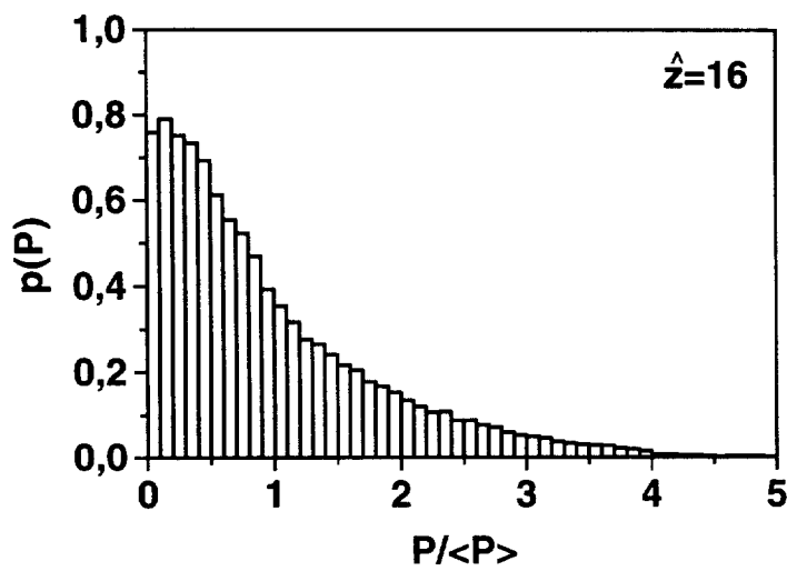
Fig. 5.29. Histograms of the probability density distribution, p(P) , of the instant output power at different reduced length of the FEL amplifier. Calculations have been performed with nonlinear simulation code over 10^4 independent statistical events. \langle P \rangle denotes the average power.
