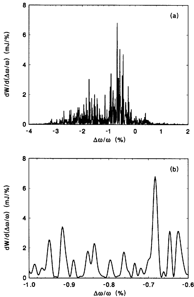
Fig. 5.19. Typical spectrum of the radiation pulse (one shot) at the reduced length of the FEL amplifier \hat{z} = 20 . Graph (a) is plotted over the full spectrum width and graph (b) presents enlarged fraction of graph (a). Calculations have been performed with nonlinear simulation code.
