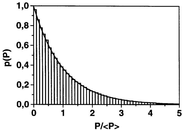
Fig. 5.3. A histogram of probability density distribution, p(P) , of instant output power at the reduced length of the FEL amplifier \hat{z} = 11 . Calculations have been performed with linear simulation code over 2 \times 10^5 independent statistical events (see Fig. 5.1). \langle P \rangle denotes the average power. The solid curve represents the negative exponential distribution p(P) = \exp(-P/\langle P \rangle) .
