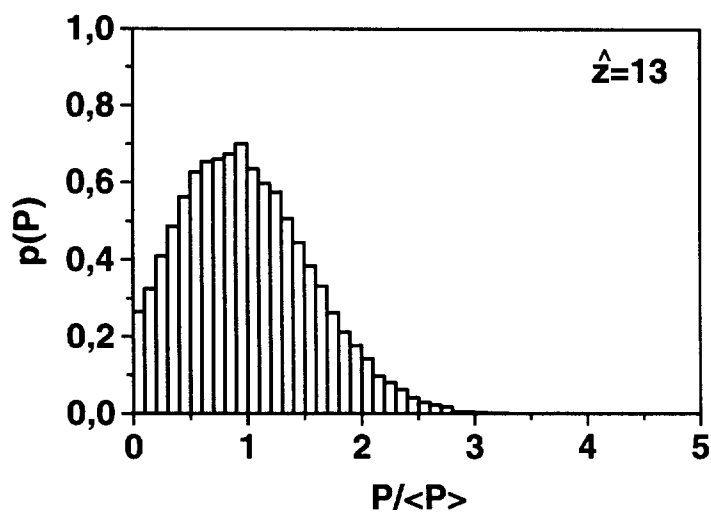
Fig. 5.28. Histograms of the probability density distribution, p(P) , of the instant output power at different reduced length of the FEL amplifier. Calculations have been performed with nonlinear simulation code over 10^4 independent statistical events. \langle P \rangle denotes the average power.
