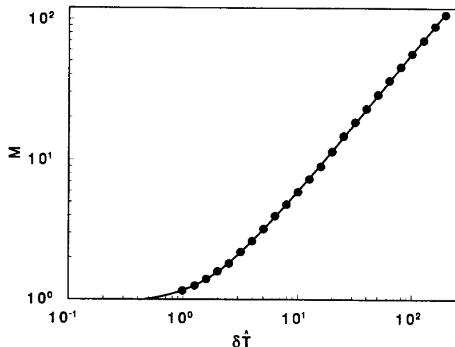
Fig. 5.10. The dependence of the parameter M on the value of the time interval \delta\hat{T} = \delta T\sigma_A . FEL amplifier operates in the linear regime at the reduced length of the FEL amplifier \hat{z} = 11 . Solid curve is the result of calculations with analytical formula (2.62). Circles are the result of calculations with linear simulation code over 2400 shots.
