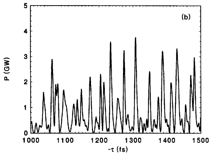
Fig. 5.18. Typical temporal structure of the radiation pulse (one shot) at the reduced length of the FEL amplifier \hat{z} = 20 . Graph (a) is plotted over the full length of the radiation pulse and graph (b) presents enlarged fraction of graph (a). Calculations have been performed with nonlinear simulation code.
