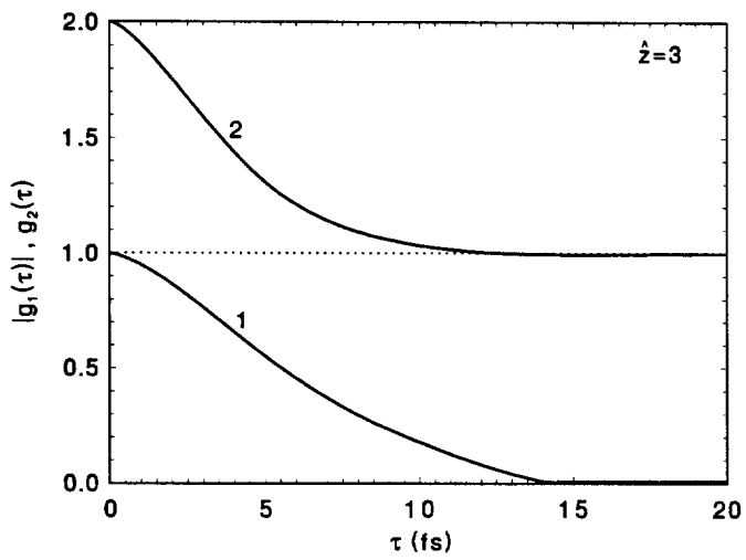
Fig. 5.15. The first and the second order time correlation functions, g_1(\tau) (curve 1) and g_2(\tau) (curve 2), of the radiation pulse at different reduced length of the FEL amplifier. Calculations have been performed with linear simulation code over 10^4 independent statistical events.
