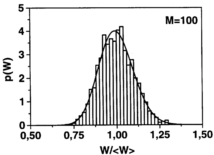
Fig. 5.14. Histograms of the probability density distribution, p(W) , of the radiation energy after monochromator for different values of parameter M . Calculations have been performed with linear simulation code over 2400 shots (see Fig. 5.2). \langle W \rangle denotes the average energy. The solid curves represent the gamma distribution (2.43) where values of M have been calculated with formula (2.44) (see also Figs. 5.11 and 5.12).
