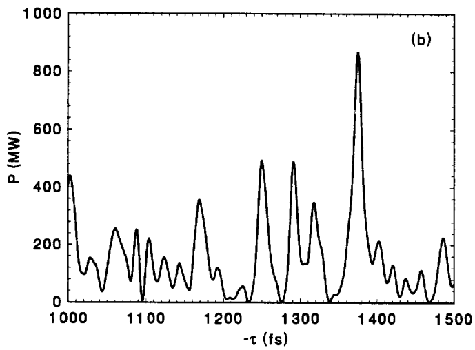
Fig. 5.1. Typical temporal structure of the radiation pulse (one shot) at the reduced length of the FEL amplifier \hat{z} = 11 . Graph (a) is plotted over the full length of the radiation pulse and graph (b) presents enlarged fraction of graph (a). Calculations have been performed with linear simulation code.
