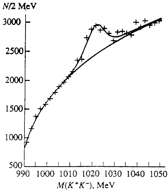
Fig. 2. Effective mass spectrum of K^+K^- system in OZI-suppressed reaction (8): \pi^- + p \rightarrow K^+K^- + (n; \Delta; N^*) .
