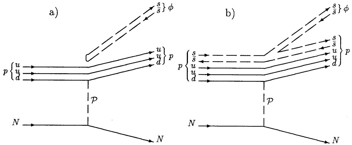
Fig. 14. \phi production in proton-nucleon or proton-nucleus diffractive reactions: a) disconnected quark diagram for ordinary proton wave function (OZI-suppressed process); b) connected quark diagram for the model in which proton wave function has small exotic component with hidden strangeness (see (39)). This process can explain apparent violation of the OZI rule in proton reactions.
