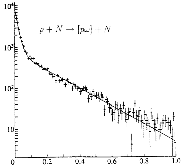
Fig. 8. Distribution of the p\omega system in the square of the transverse momentum P_T^2 for reaction (27).
