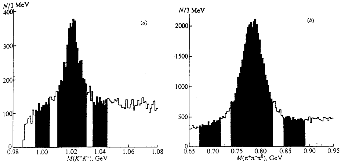
Fig. 6. Selection of the reactions p + N \rightarrow [p\phi] + N (26) and p + N \rightarrow [p\omega] + N (27) and illustration of sideband method for background subtraction to separate these processes: a) effective mass spectrum M(K^+K^-) in p + N \rightarrow [pK^+K^-] + N (29); b) effective mass spectrum M(\pi^+\pi^-\pi^0) in p + N \rightarrow [p\pi^+\pi^-\pi^0] + N (30). The regions of the \phi and \omega peaks and sideband regions for background subtraction to obtain all distributions in (26) and (27) are shown on these spectra.
