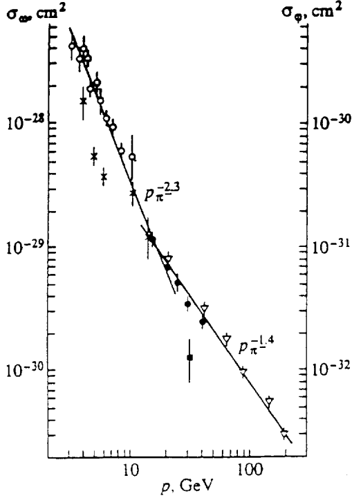
Fig. 4. Total cross sections for the reactions \pi^- + p \rightarrow \phi + n and \pi^- + p \rightarrow \omega + n as functions of the beam momentum P_{\pi^-} . Results for the reaction \pi^- + p \rightarrow \omega + n correspond to the left-hand scale: (o) low-energy data [35], (•) data from [33], \nabla data from [34]. Straight lines correspond to power-law parametrizations \sigma \sim P_{\pi^-}^{-2.3} and \sigma \sim P_{\pi^-}^{-1.4} . Results for the reaction \pi^- + p \rightarrow \phi + n correspond to the right-hand scale: \times — data from [35] for relatively low energies; \blacksquare — results of this investigation with the LEPTON-F detector.
