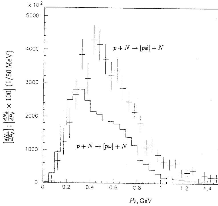
Fig. 10. The weighted distributions dN/dP_v for reactions (26) and (27) as functions of momentum P_v in the rest frame of pV system. The distribution for p\phi is scale by a factor of 100.
