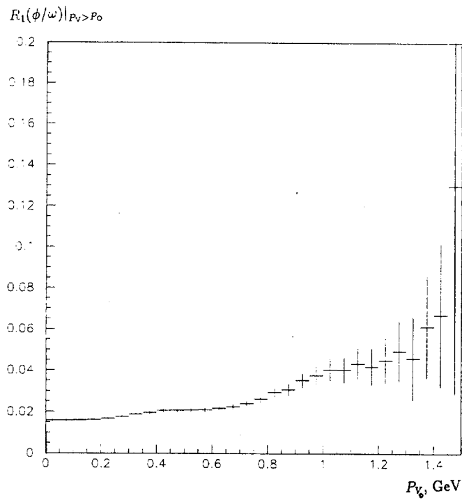
Fig. 11. Integrated ratio R_1(\phi/\omega) (see(33)) as a function of minimal momentum P_{v\min} = P_0 .
