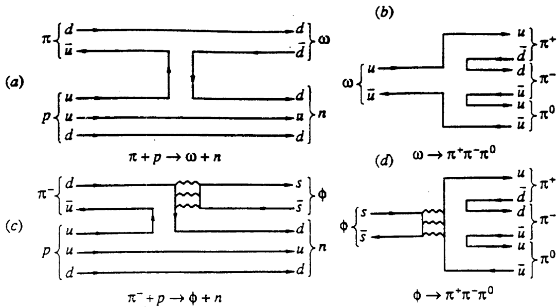
Fig. 1. Diagrams for: (a,b) OZI-allowed and (c,d) OZI-suppressed production and decay processes: (a) reaction \pi^- + p \rightarrow \omega + n ; (b) decay \omega \rightarrow \pi^+ \pi^- \pi^0 (connected quark diagrams); (c) reaction \pi^- + p \rightarrow \phi + n , and (d) decay \phi \rightarrow \pi^+ \pi^- \pi^0 (disconnected quark diagrams).
