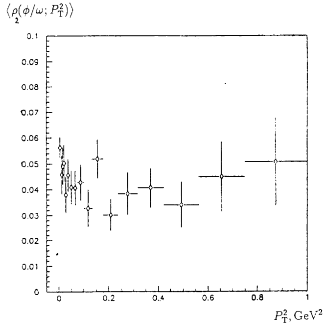
Fig. 13. Weighted ratio \langle \rho_2(\phi/\omega) \rangle_{|M > M_p + M_\phi} as a function of squared transverse momentum P_T^2 of the pV system.
