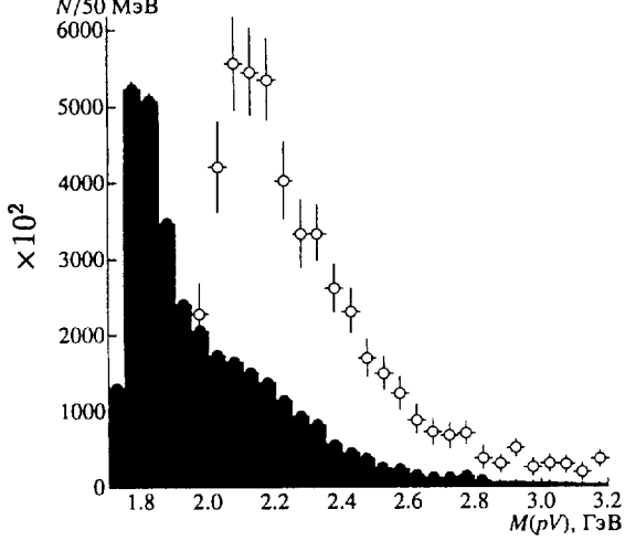
Fig. 9. Weighted distributions of events in the mass M(pV) (here and in other figures of this subsection all distributions are weighted with efficiency of the setup). Closed and open circles represent, respectively, the distribution on p\omega and the scale distribution of p\phi (scale factor is 100).
