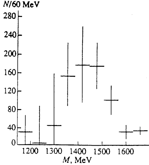
Fig. 5. Effective mass spectrum of the \phi\pi^0 system in the reaction \pi^- + p \rightarrow (\phi\pi^0) + n (the results are weighted with detector efficiency). An “anti-OPE” selection |t'| > 0.1 \text{ (GeV)}^2 is applied, which affects only slightly the efficiency for the reaction \pi^- + p \rightarrow B/b_1(1235) + n (not proceeding via OPE exchange), but which reduces the background from the OPE-mediated reaction \pi^- + p \rightarrow C(1480)^0 + n by a factor close to 5.
