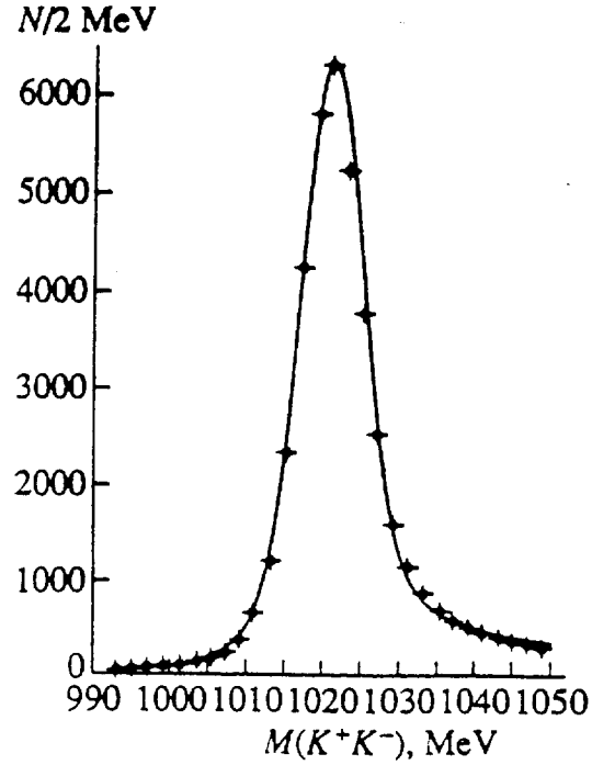
Fig. 3. Effective mass spectrum of K^+K^- system in OZI-allowed reaction (9): K^- + p \rightarrow K^+K^- + Y .
