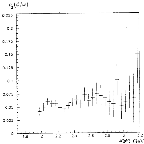
Fig. 12. Differential ratio \rho_2(\phi/\omega; M) (see (35)) as a function of effective mass M(pV) .
