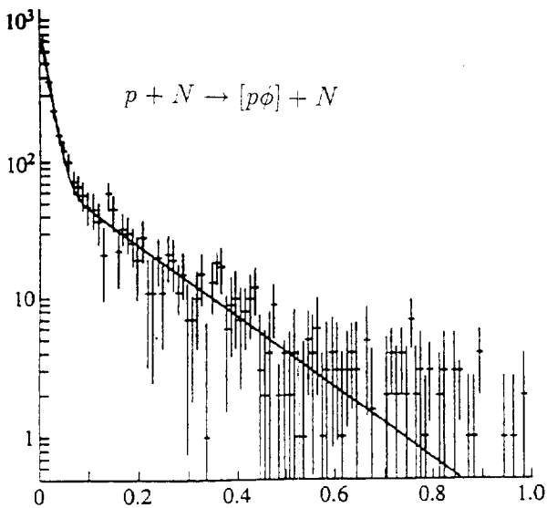
Fig. 7. Distribution of the p\phi system in the square of the transverse momentum P_T^2 for reaction (26).
