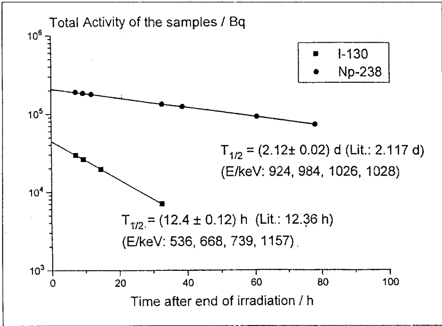
Fig.4. The decay curves of iodine-130 and neptunium-238, formed in the reactions ^{129}\text{I}(n, \gamma)^{130}\text{I} and ^{237}\text{Np}(n, \gamma)^{238}\text{Np}
