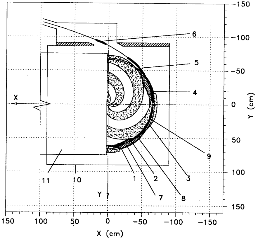
Figure 2: Extraction system layout. 1,2,3 - electrostatic deflector sections ESD-1,2,3; 4,5,6 - magnetic channel sections MC-1,2,3; 7 - valley shim; 8 - harmonic coil; 9 - spiral shim; 10 - vacuum chamber; 11 - dee
