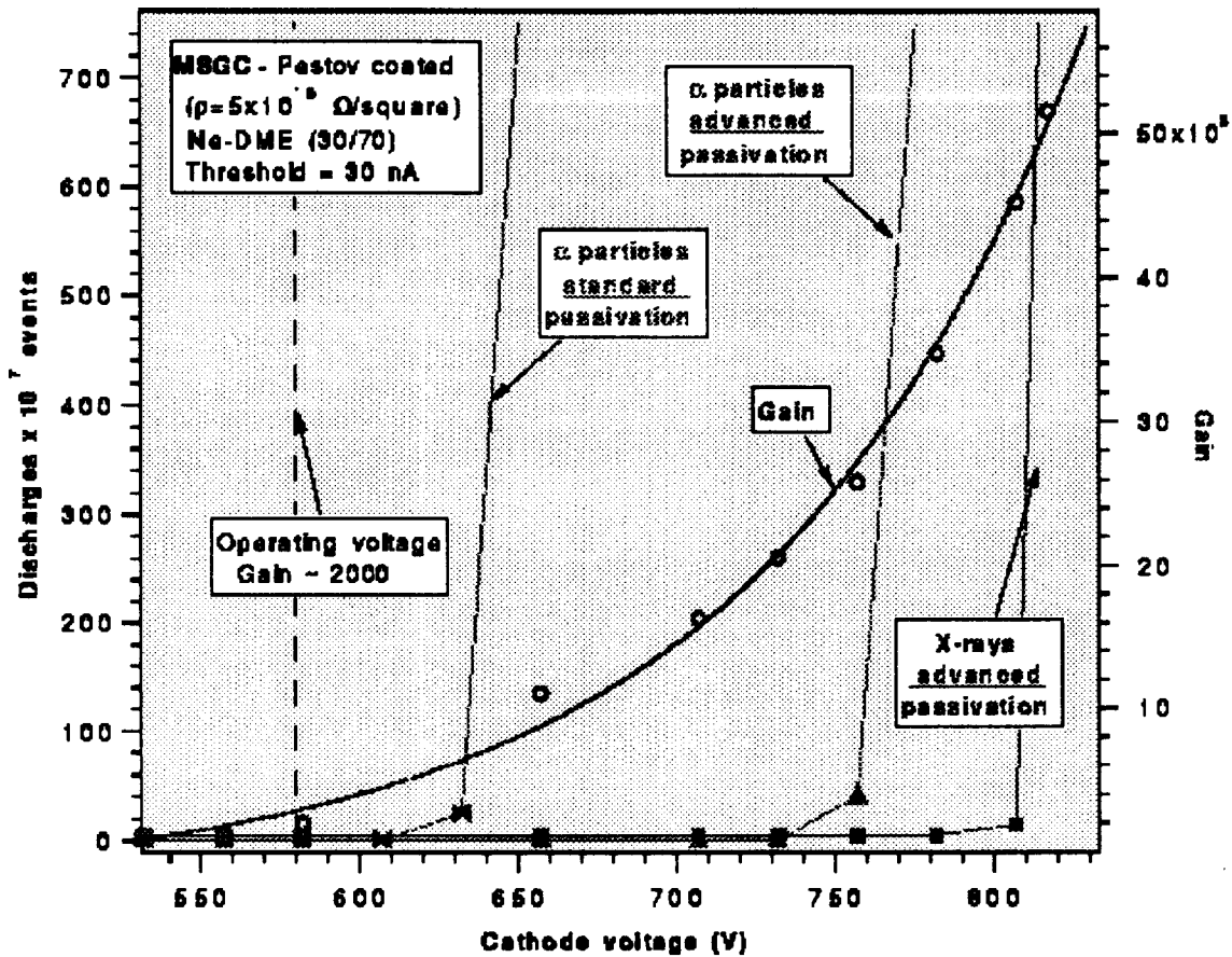
Fig. 3. Example results showing sparking rate as a function of cathode voltage, for two types of passivation.
