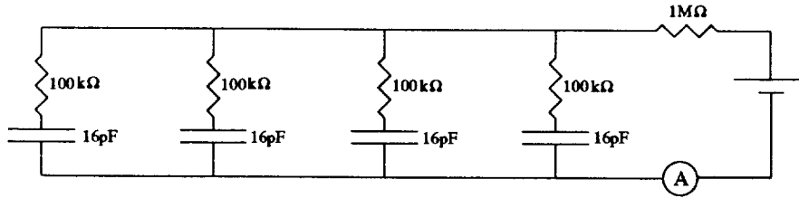
Fig. 1. Electrical model of MSGCs used in the tests.
