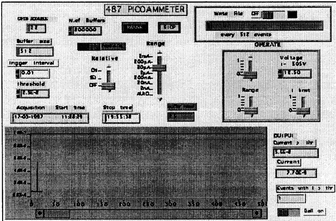
Fig. 2. Labview display showing typical micro-discharge event.
