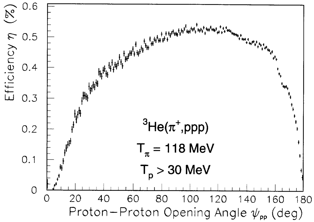
FIG. 5. Differential efficiency for the proton-proton opening angle \psi_{pp} in the laboratory system. The steep fall-off at low and high angles is mainly caused by the finite segmentation of the detector.
