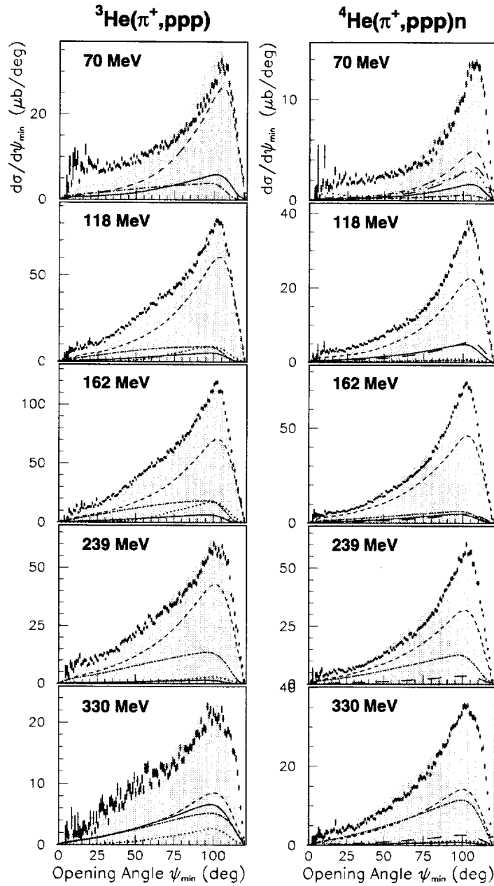
FIG. 16. Minimum opening angle \psi_{min} distributions of the {}^3\text{He}(\pi^+, ppp) (left column) and {}^4\text{He}(\pi^+, ppp)n (right column) reactions for T_\pi = 70, 118, 162, 239 and 330 MeV. All spectra are acceptance corrected with a threshold of T_p = 30 MeV. The dots with the error bars are the data and the shaded areas the sums of the simulations. The lines are the fitted contributions of the simulations for 2NA (solid), summed 3N phase space for L \geq 0 and L \geq 1 (short-dashed), ISI (dashed-dotted), and HFSI (dotted). The long-dashed lines of the {}^4\text{He} fits are the sums of the tails of the 4NA_{(pppn)} and 3NA_{(ppn)p} simulations.
