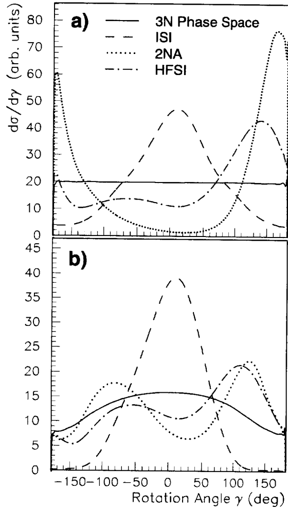
FIG. 14. Comparison of the rotation angle distributions of the ppp final state from {}^3\text{He} at T_\pi = 162 MeV for the different simulations used in the analysis with T_p > 0 MeV (a) and with T_p > 30 MeV (b).
