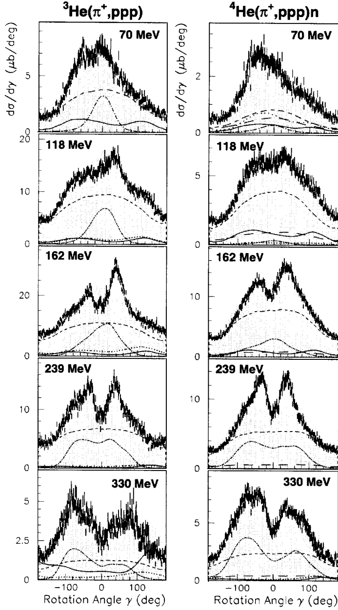
FIG. 15. Rotation angle \gamma distributions of the {}^3\text{He}(\pi^+, ppp) (left column) and {}^4\text{He}(\pi^+, ppp)n (right column) reactions for T_\pi = 70, 118, 162, 239 and 330 MeV. All spectra are acceptance corrected with a threshold of T_p = 30 MeV. The dots with the error bars are the data and the shaded areas the sums of the simulations. The lines are the fitted contributions of the simulations for 2NA (solid), summed 3N phase space for L \geq 0 and L \geq 1 (short-dashed), ISI (dashed-dotted), and HFSI (dotted). The long-dashed lines of the {}^4\text{He} fits are the sums of the tails of the 4NA_{(pppn)} and 3NA_{(ppn)p} simulations.
