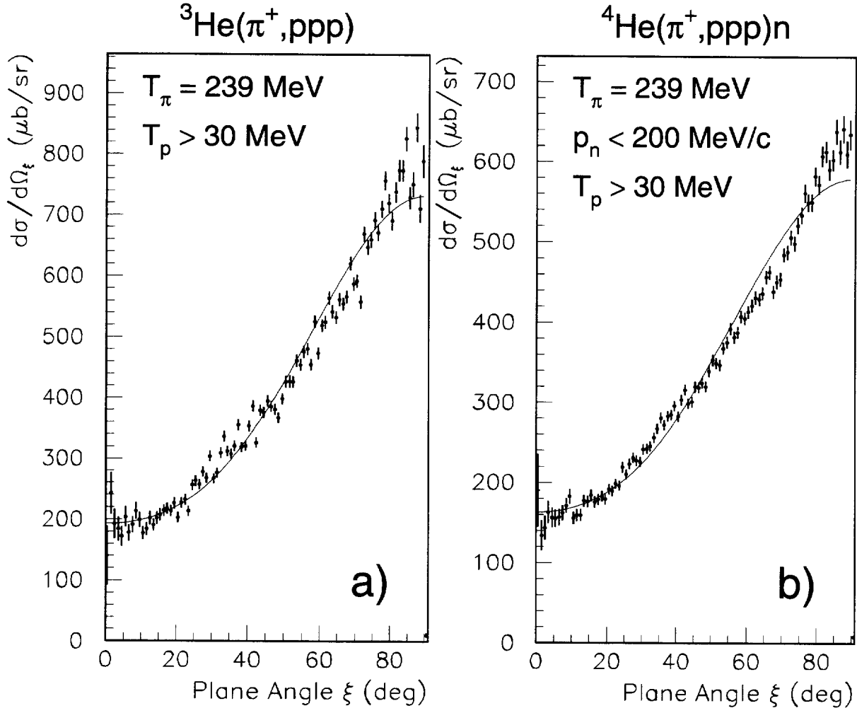
FIG. 11. Plane angle distribution of the (ppp) (a) and (ppp)n (b) channel after absorption by {}^3\text{He} and {}^4\text{He} , respectively, for 239 MeV incident pion energy. The dots with error bars are the efficiency corrected data, the solid lines show a fit of the Legendre expansion Eq. (5.1).
