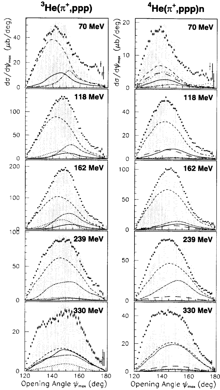
FIG. 17. Maximum opening angle \psi_{max} distributions of the {}^3\text{He}(\pi^+, ppp) (left column) and {}^4\text{He}(\pi^+, ppp)n (right column) reactions for T_\pi = 70, 118, 162, 239 and 330 MeV. All spectra are acceptance corrected with a threshold of T_p = 30 MeV. The dots with the error bars are the data and the shaded areas the sums of the simulations. The lines are the fitted contributions of the simulations for 2NA (solid), summed 3N phase space for L \geq 0 and L \geq 1 (short-dashed), ISI (dashed-dotted), and HFSI (dotted). The long-dashed lines of the {}^4\text{He} fits are the sums of the tails of the 4NA_{(pppn)} and 3NA_{(ppn)p} simulations.
