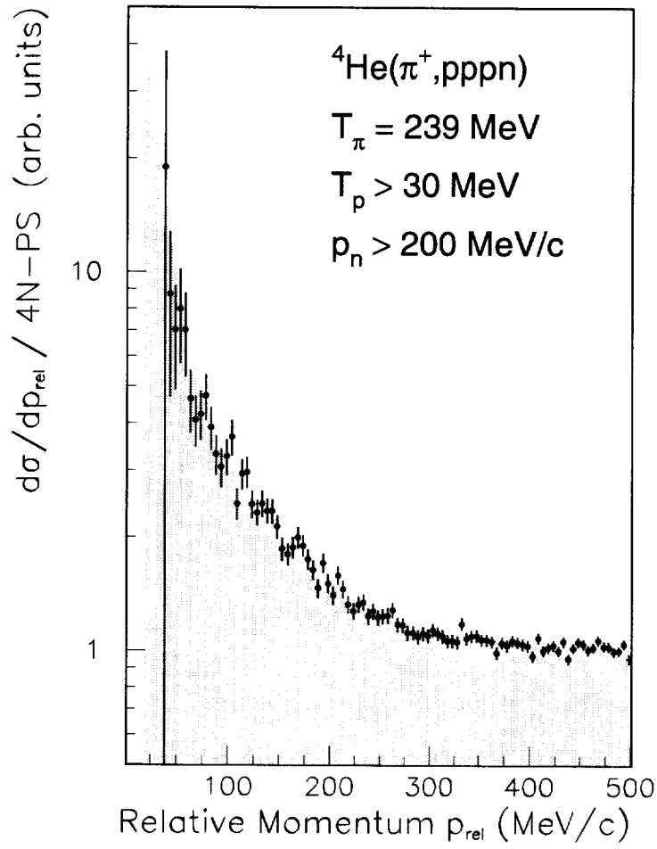
FIG. 7. Measured relative momentum of proton-neutron pairs from the reaction {}^4\text{He}(\pi^+,pppn) at 239 MeV divided by a LADSON30 4NA_{(pppn)} simulation. The shaded area represents the Jost pn -SFSI enhancement function.
