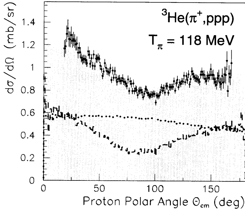
FIG. 8. Proton polar angle distribution with T_p > 30 MeV in the ppp -subframe following the absorption of 118 MeV pions by {}^3\text{He} . The dots with error bars are the efficiency corrected data, the lines are the fitted 2NA_{(pp)p} (dashed) and 3NA_{(ppp)}^{L>0} (dotted) simulations with the shaded area as the sum of these.
