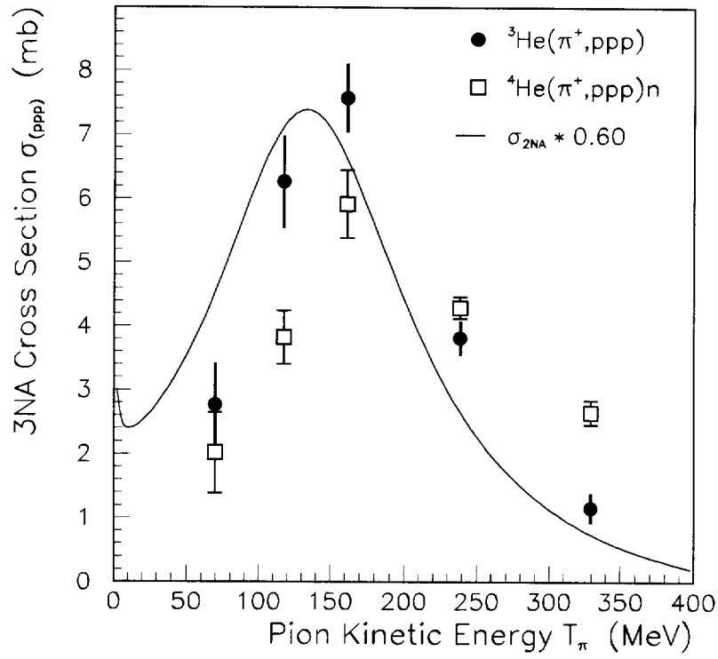
FIG. 21. 3NA( ppp ) cross sections for {}^3\text{He} and {}^4\text{He} . The solid line is the parametrized deuteron absorption cross section [31] scaled by a factor of 0.60.
