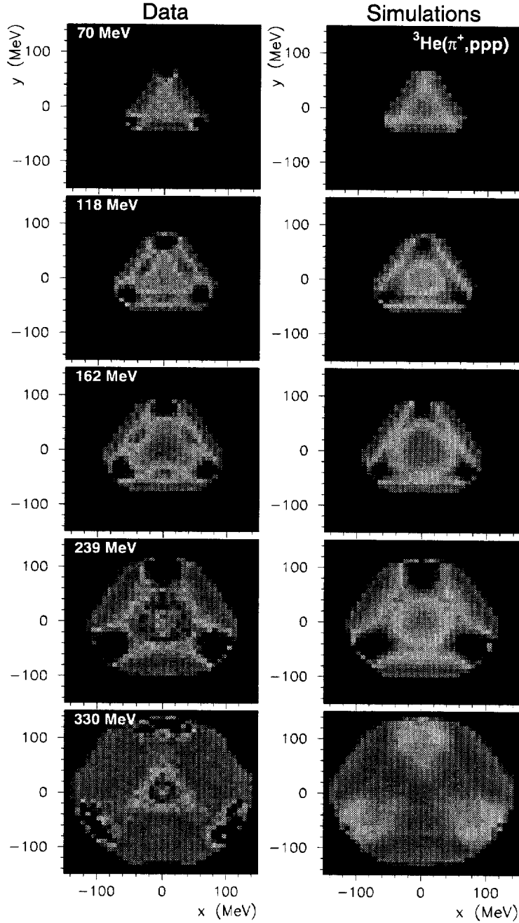
FIG. 19. (Colour). Triangular Dalitz plots for the reaction {}^3\text{He}(\pi^+, ppp) at T_\pi = 70, 118, 162, 239 and 330 MeV with T_p > 30 MeV. Left column: acceptance corrected data; right column: sum of simulations normalized to the data according to the fractional decomposition of Table V. For each energy the plots of the data and the simulations are normalized to the same maximum value in the z direction. The colour sequence blue, green, yellow, brown, black indicates the increasing yield.
