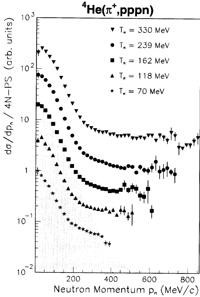
FIG. 6. Momentum density distribution of the neutron from the reaction {}^4\text{He}(\pi^+, pppn) with T_p > 30 MeV for five incident pion energies, divided by a 4N phase space simulation ( 4NA_{(pppn)} ). The solid points are the data, arbitrarily normalized, while the shaded area represents a Monte Carlo 3NA_{(ppn)}^{L \geq 0} simulation at 162 MeV where the neutron was weighted to be a spectator.
