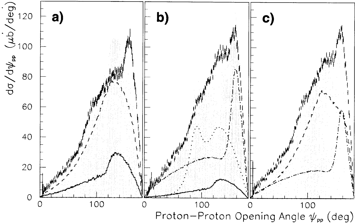
FIG. 9. Proton-proton opening angle \psi_{pp} in the laboratory frame for the reaction {}^3\text{He}(\pi^+, ppp) with T_p > 30 \text{ MeV} at T_\pi = 239 \text{ MeV} . The data were fitted with different combinations of 2NA_{(pp)p} (solid line), 3NA_{(ppp)} (dashed), ISI_{(ppp)} (dashed-dotted) and HFSI_{(ppp)} (dotted), as described in the text. The shaded areas are always the sums of the fitted simulations. The slightly different shapes of the data are due to changes in the acceptance correction when different models are used.
