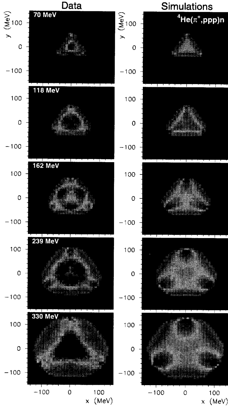
FIG. 20. (Colour). Triangular Dalitz plots for the reaction {}^4\text{He}(\pi^+, ppp)n at T_\pi = 70, 118, 162, 239 and 330 MeV with T_p > 30 MeV and p_n < 200 MeV/c. Left column: acceptance corrected data; right column: sum of simulations normalized to the data according to the fractional decomposition of Table V. For each energy the plots of the data and the simulations are normalized to the same maximum value in the z direction. The colour sequence blue, green, yellow, brown, black indicates the increasing yield.
