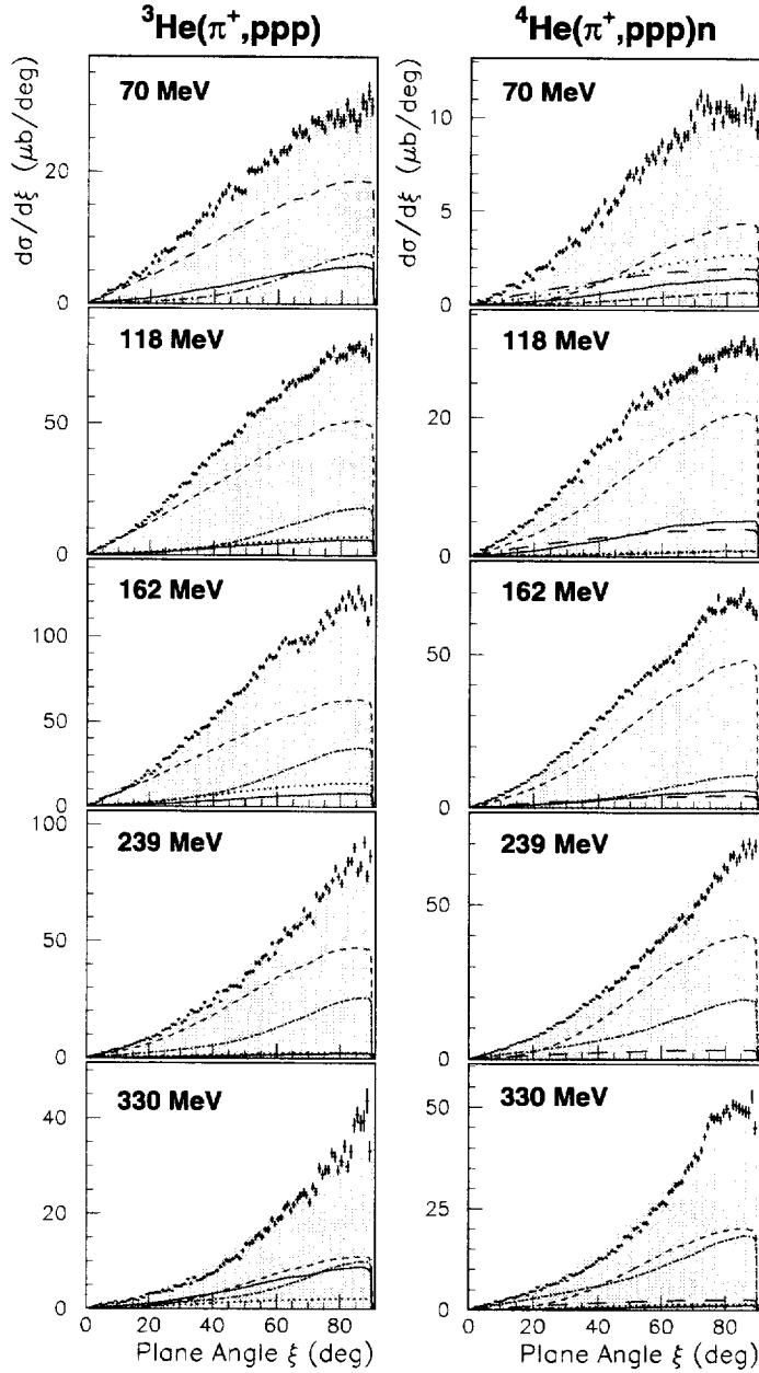
FIG. 13. Plane angle \xi distributions of the {}^3\text{He}(\pi^+, ppp) (left column) and {}^4\text{He}(\pi^+, ppp)n (right column) reactions for T_\pi = 70, 118, 162, 239 and 330 MeV. All spectra are acceptance corrected with a threshold of T_p = 30 MeV. The dots with the error bars are the data and the shaded areas the sums of the simulations. The lines are the fitted contributions of the simulations for 2NA (solid), summed 3N phase space for L \geq 0 and L \geq 1 (short-dashed), ISI (dashed-dotted), and HFSI (dotted). The long-dashed lines of the {}^4\text{He} fits are the sums of the tails of the 4NA_{(pppn)} and 3NA_{(ppn)p} simulations.
