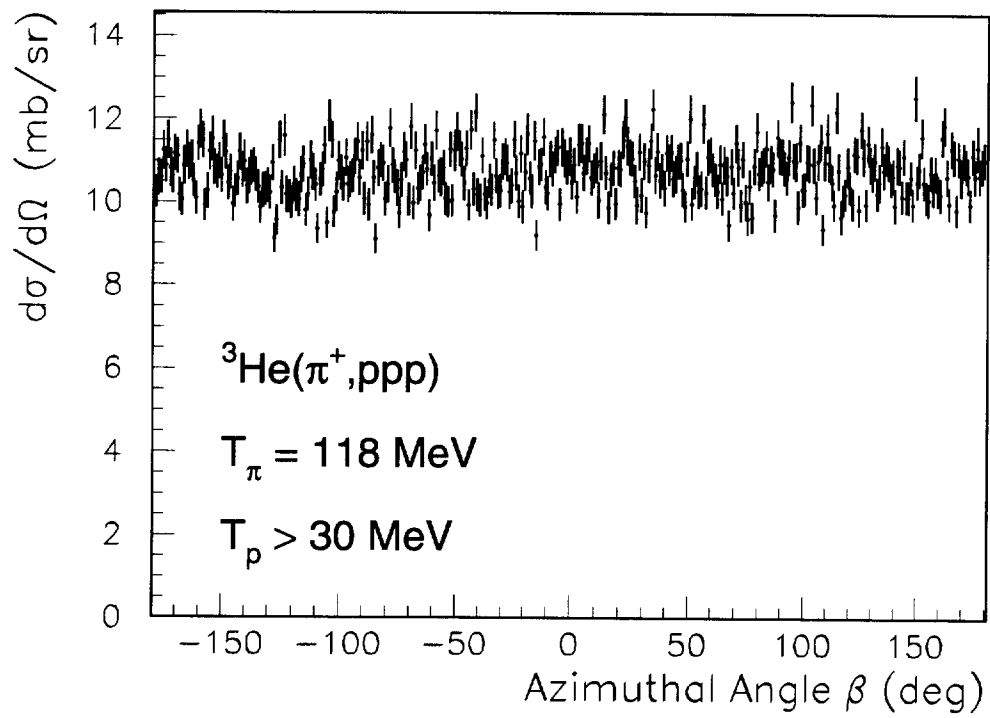
FIG. 10. Distribution of the azimuthal angle \beta for the reaction {}^3\text{He}(\pi^+, ppp) at T_\pi = 118 MeV.
