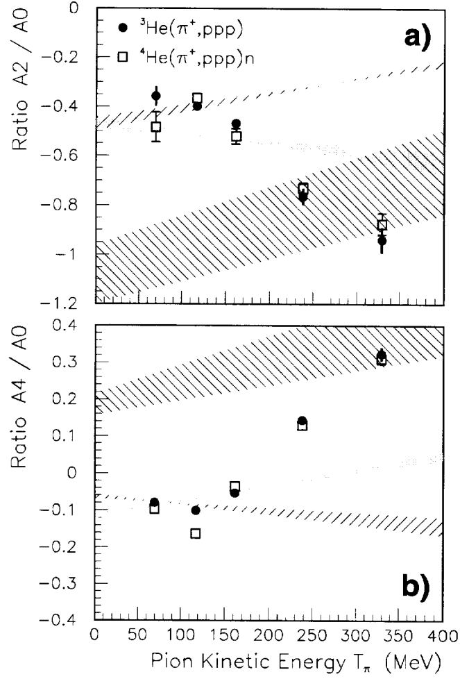
FIG. 12. Ratios A_2/A_0 (a) and A_4/A_0 (b) of the Legendre expansion Eq. (5.1) of the plane angle \xi as obtained from fits to the ppp data ( T_p > 30 MeV; p_n < 200 MeV/c for {}^4\text{He} ) for the nuclei {}^3\text{He} and {}^4\text{He} . The error bars include the fit and normalization uncertainties. The bands reflect the predicted energy dependences from our semi-classical cascade models: 2NA [shaded], (ISI+2NA) [left-hatched, e.g. bottom of (a)], and (2NA+HFSI) [right-hatched].
