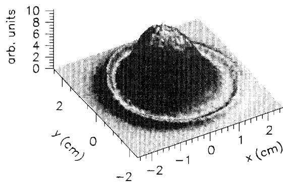
FIG. 3. Vertex reconstruction plots with the target cell filled with {}^4\text{He} gas. Upper: For the projection in the beam direction ( z ) a radial cut of 17 mm was applied. The two sharp peaks reflect background events from the target wall end-caps. Lower: For the projection onto the transverse ( x - y ) plane a cut of 10 cm upstream and downstream of the target centre was applied. The events from the target gas (broad bump) can be clearly distinguished from those of the target walls (ring around the centre).
