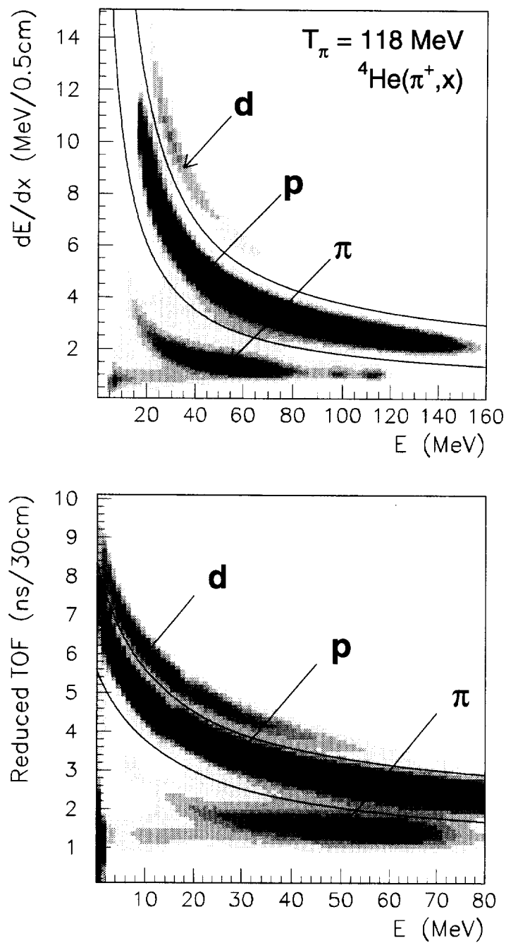
FIG. 4. E - dE/dx (upper) and E - TOF (lower) spectra used for the particle identification. The kinks around 20 MeV in the lower plot are caused by the transition from the \Delta E to the E scintillators. The cuts applied for proton selection are also shown (solid curves).
