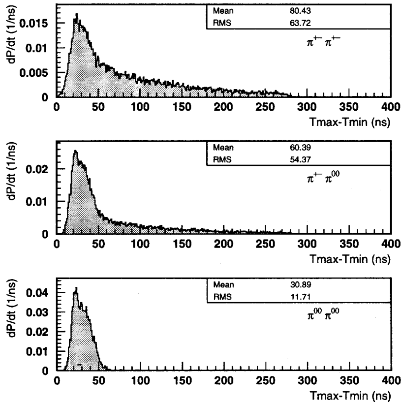
Figure 3.1. Distribution of arrival times at the calorimeter.
