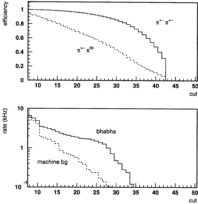
Figure 4.2. Efficiency and background rates as a function of the cut on the parameter N_c .
