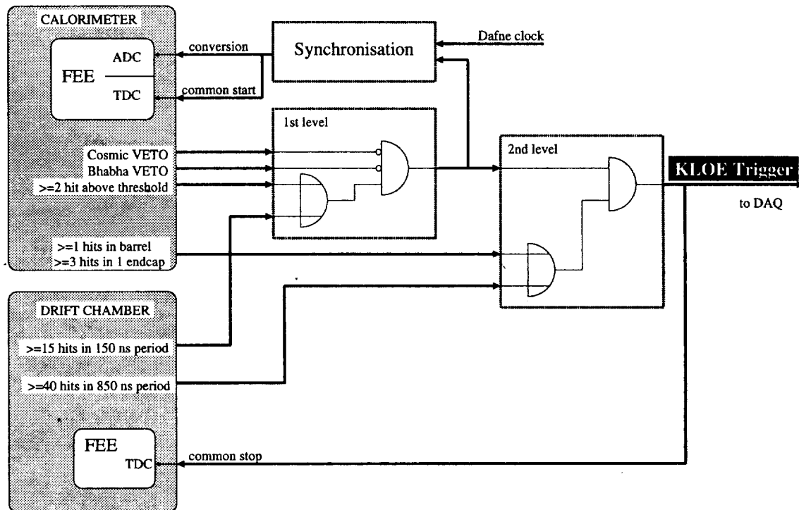
Figure 3.2. Block diagram of the two level trigger.
