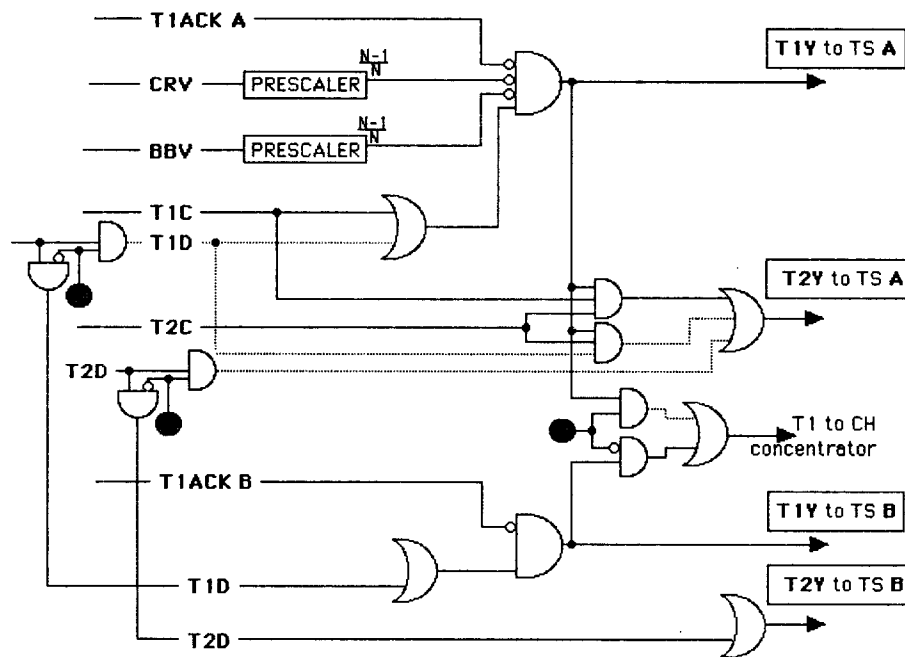
Figure 5.9. The partitioning capability of the trigger system is sketched: the calorimeter and chamber information is independently managed by two identical sections of the TORTA and two trigger supervisors (TS A and TS B).
