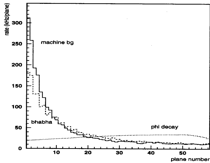
Figure 3.11. Plane distribution of the D.C. hits
