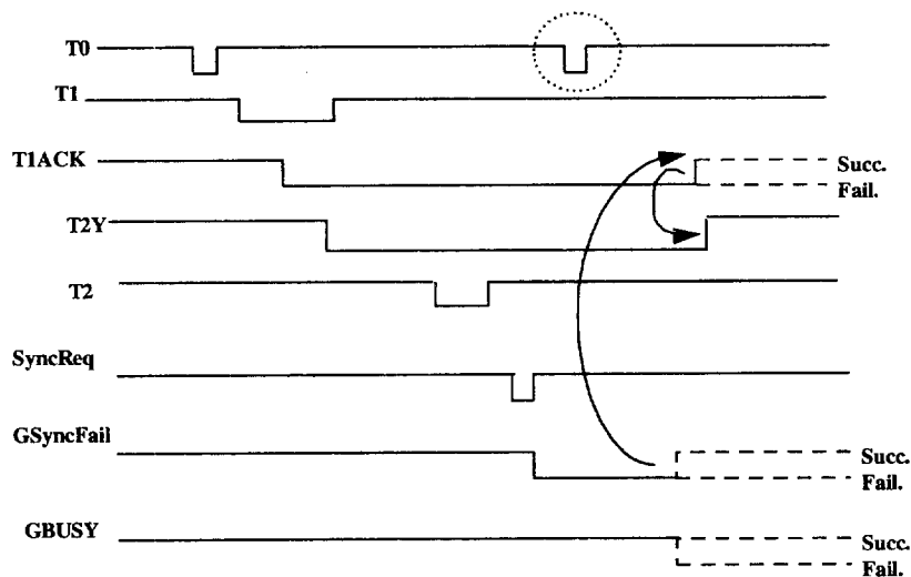
Figure 6.3. Synchronization cycle
