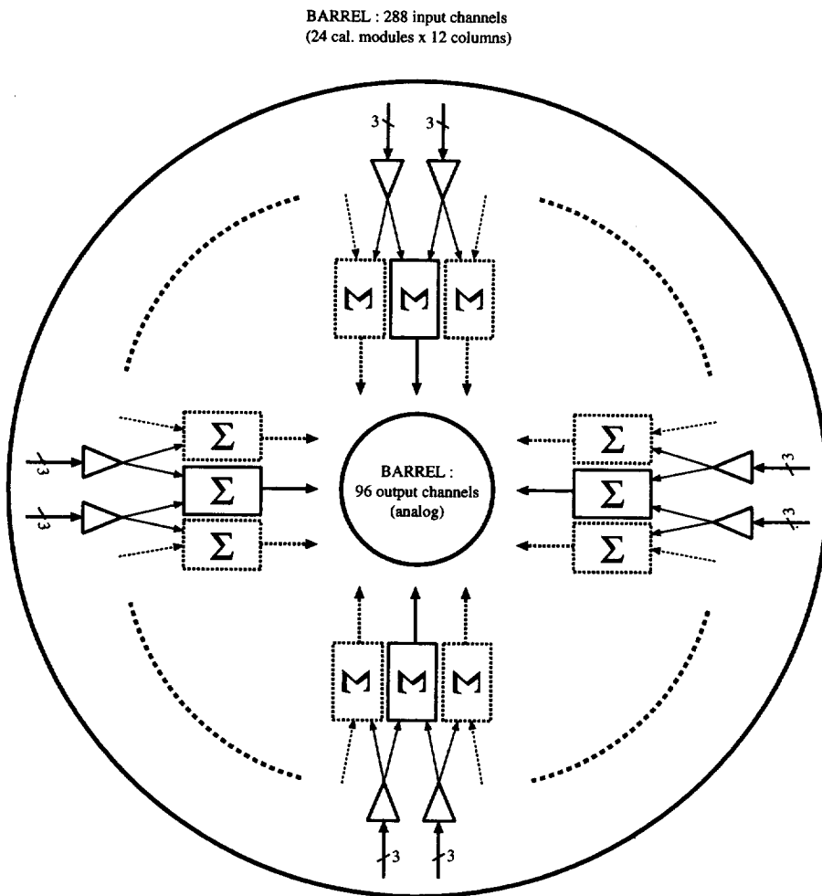
Figure 5.2. Block diagram of the barrel Trigger-Pizza.
