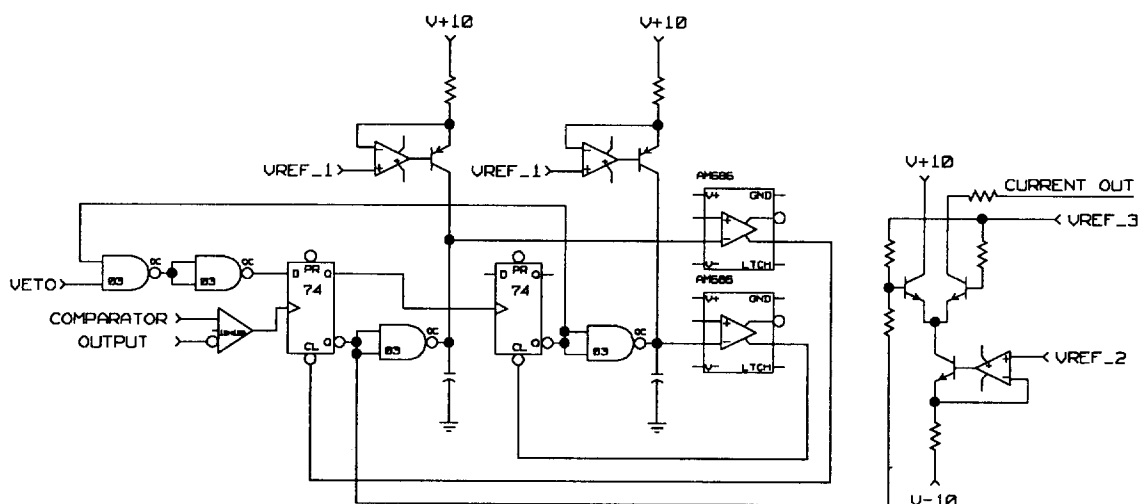
Figure 5.4. Simplified layout of one of the 48 channels of the discriminator card.
