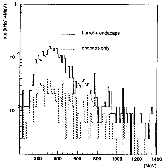
Figure 2.9. Energy deposited by cosmic rays.
