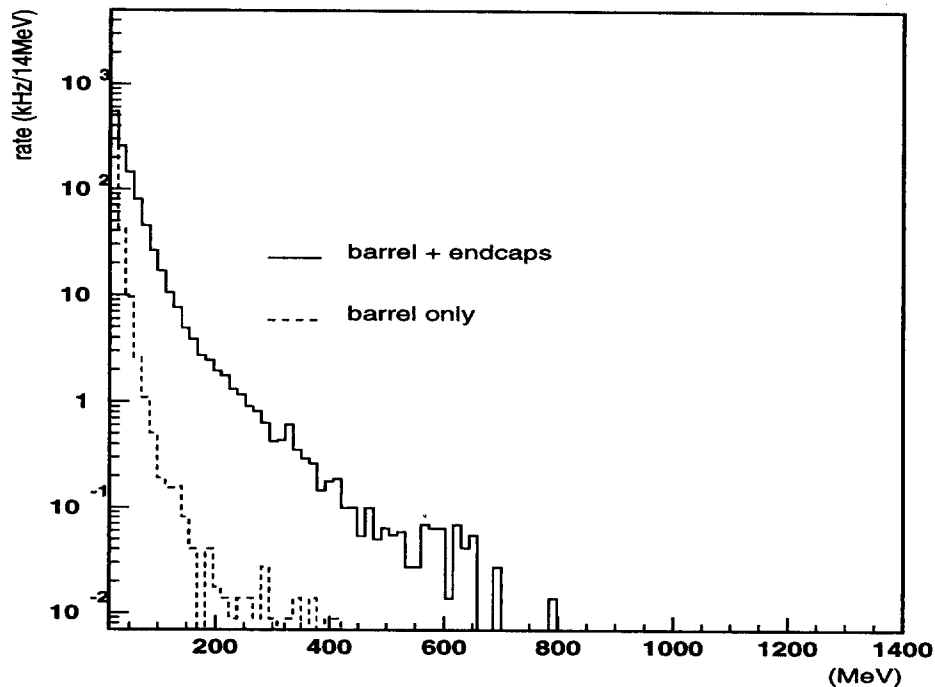
Figure 2.7. Energy deposited in the EMC by background radiation.
