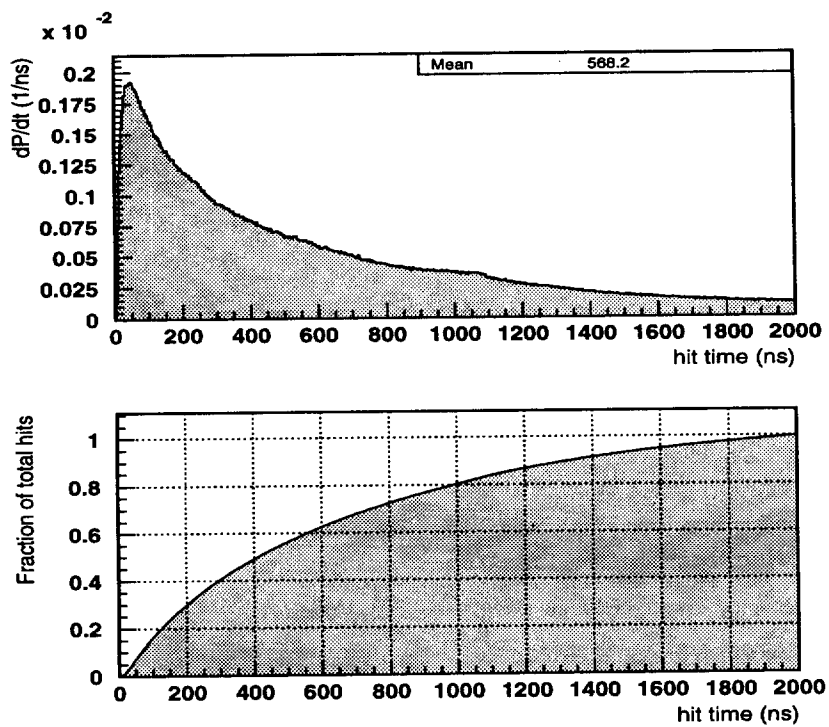
Figure 3.9. Differential and integral time distributions of the DC hits for a 3 \times 3 cell. The time is measured from the bunch crossing and include TOF, drift and propagation along wire.
