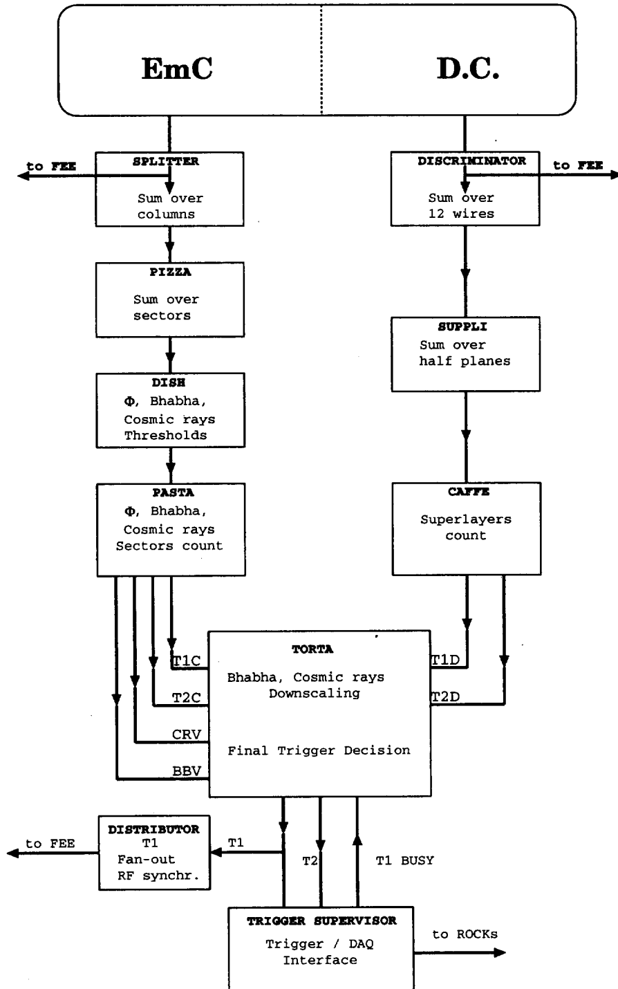
Figure 5.1. Block diagram of the Trigger System Architecture.
