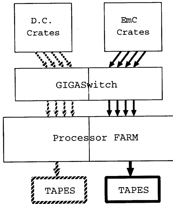
Figure 6.6. Partitioning scheme at the FARM level.
