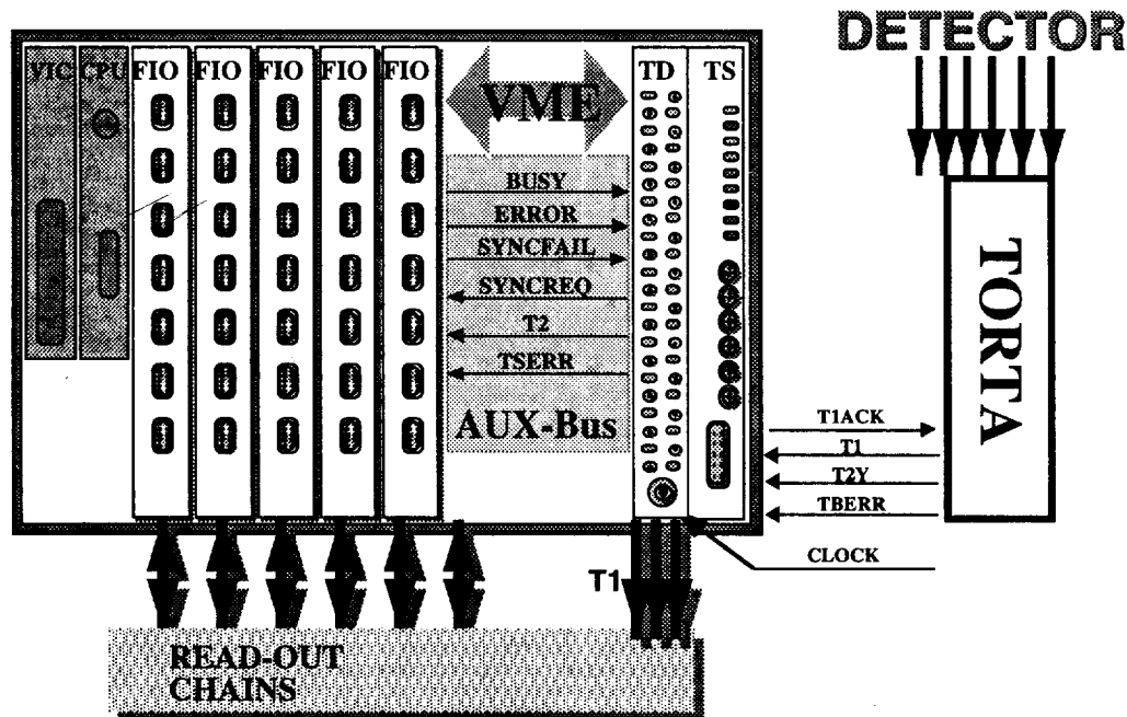
Figure 6.1. Trigger supervisor crate.
