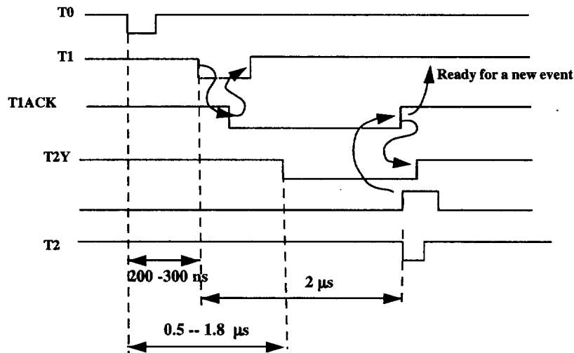
Figure 6.2. Normal cycle.
