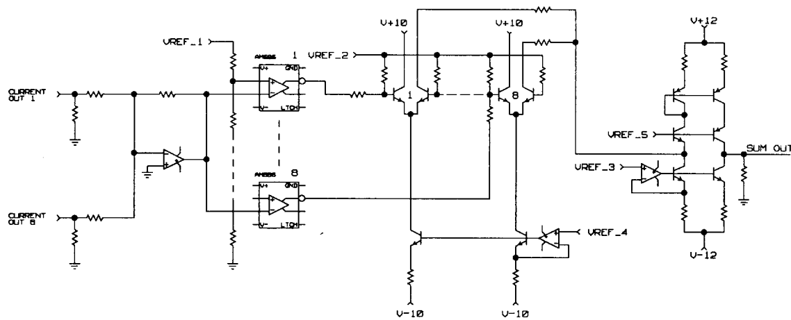
Figure 5.5. Simplified schematics of one of the 12 sum and rediscritization circuits used in the SUPPLI board.
