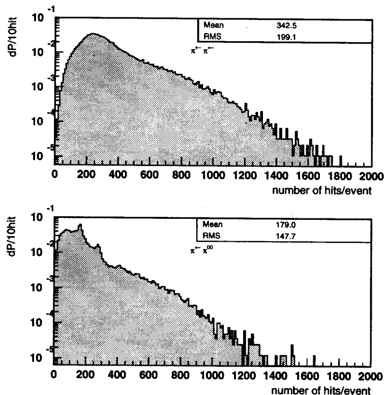
Figure 2.3. Number of DC hits for \pi^{\pm,00}, \pi^{\pm,\pm} events
