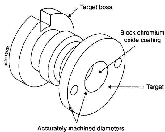
Figure 8. Plasma compatible target.
