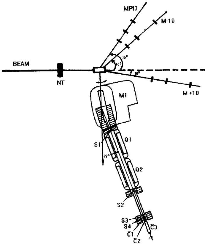
Figure 1. Experimental layout.
