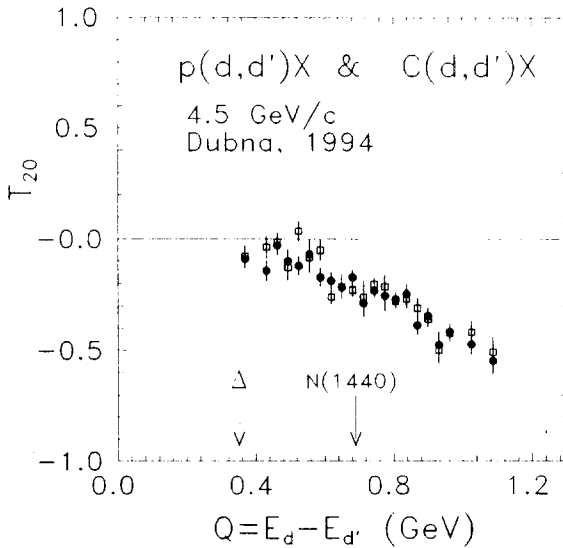
Figure 2: Tensor analysing power of the C(d,d')X (squares) and p(d,d')X (full circles) inelastic scattering at 0^\circ versus the energy transfer Q defined in the text.
