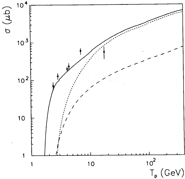
Figure 5: Total cross section of inclusive K^+ production. The dots show experimental data from [5]. The lines show the contribution from associated \Sigma (dashed) and \Lambda production (dashed-dotted), reaction pp \rightarrow NYK^+ (dotted) and their sum (solid).
