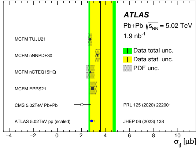
Figure 2: Comparison between observed and predicted values of \sigma_{t\bar{t}} . This measurement is compared with the CMS Collaboration measurement of \sigma_{t\bar{t}} in Pb+Pb collisions at \sqrt{s_{\text{NN}}}=5.02 TeV [13] and the ATLAS measurement in pp collisions at \sqrt{s} = 5.02 TeV [36]. The latter is scaled by A_{\text{Pb}}^2 . The theoretical cross-section is obtained from NLO calculations using the MCFM generator [60] scaled to the NNLO+NNLL precision by the K -factor of K = 1.149 . Predictions are scaled to the Pb+Pb system by A_{\text{Pb}}^2 and given for different nPDF sets. The uncertainty in predictions represents the internal PDF uncertainty.
