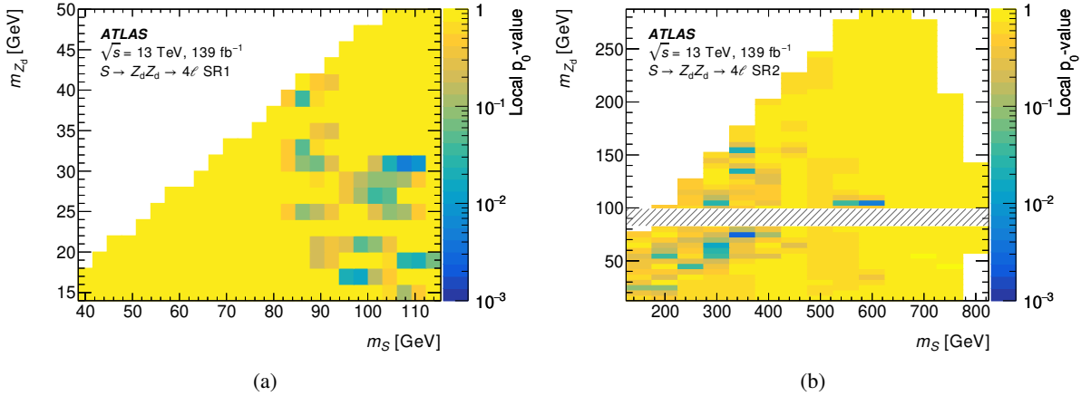
Figure 6: Local p_0 -values in the (m_{d\ell}, \langle m_{\ell\ell} \rangle) plane for (a) SR1 and (b) SR2, evaluated in slices in m_{d\ell} . The horizontal band in the SR2 figure shows the region excluded by the Z boson veto requirement, |m_{ab,cd} - m_Z| > 8 GeV.
