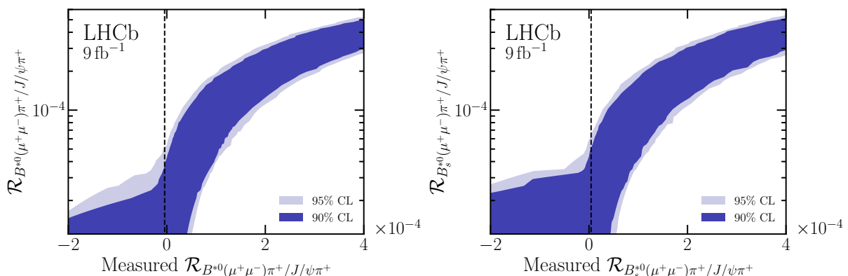
Figure 4: Confidence belts generated using pseudoexperiments according to the Feldman–Cousins prescription. The vertical black line shows the results of the fit to data.
