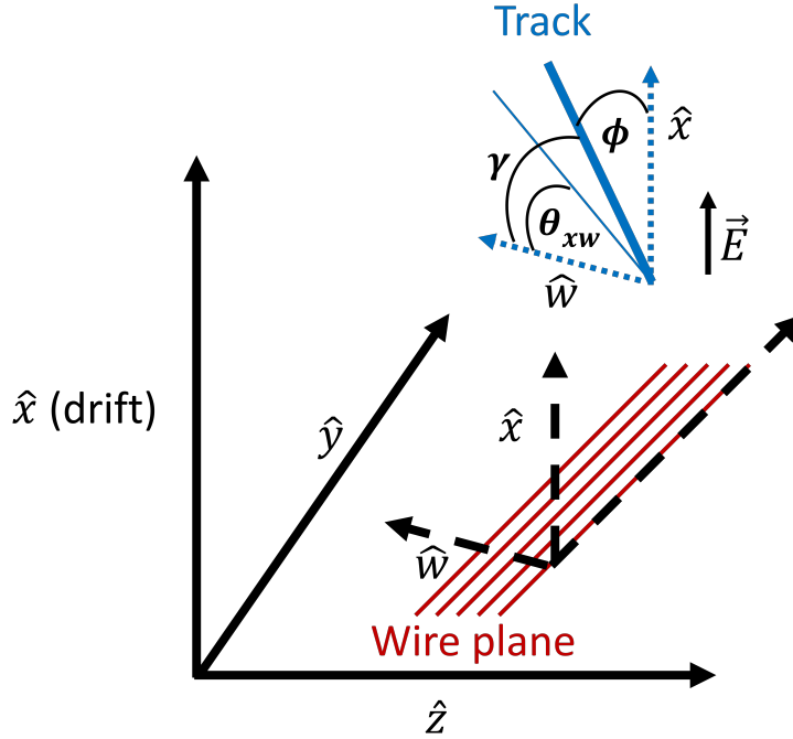
Figure 2. Diagram of relevant track angles. \gamma , the angle of the the track to the direction perpendicular to the wire direction, determines the track pitch. \phi , the angle of the track to the drift electric field, controls any angular dependence in electron-ion recombination. \theta_{xw} , the angle of the track between the drift electric field direction and the direction perpendicular to the wire direction, controls the track ionization signal shape.
