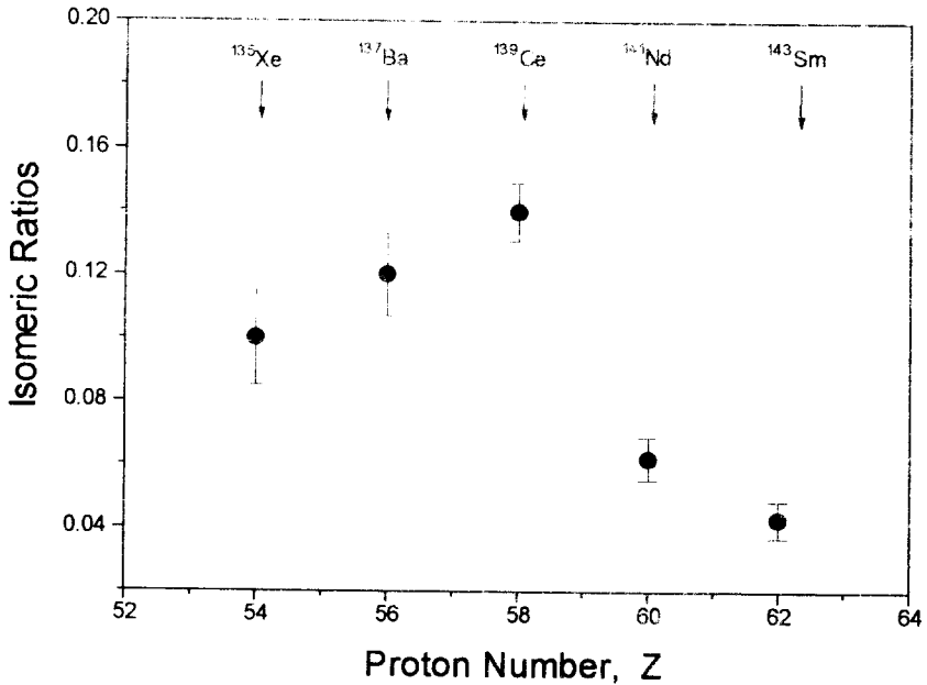
Fig.3. IR versus Z for isotopes with N = 81
