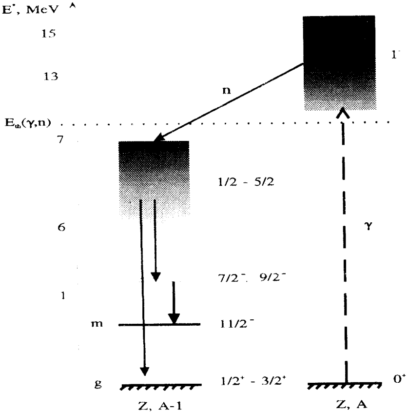
Fig.4. Excitation of isomeric states 11/2^- in (\gamma, n) -reactions
