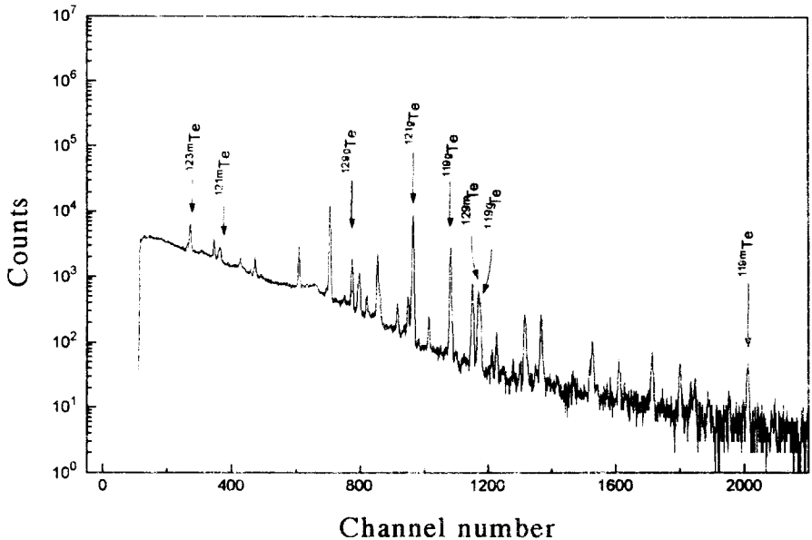
Fig.1. T_{\text{a,nat}} \gamma -spectrum produced upon irradiation by bremsstrahlung E_{\gamma\max} = 25 MeV. (Irradiation time is 4 hours, cooling time - 23 hours and time of spectrum collecting - 15 minutes)
