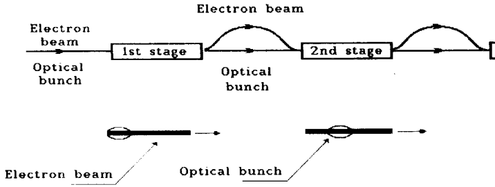
Fig. 1. The scheme of optical power summation.
