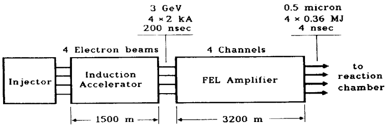
Fig. 2. General scheme of FEL based ICF energy driver.
