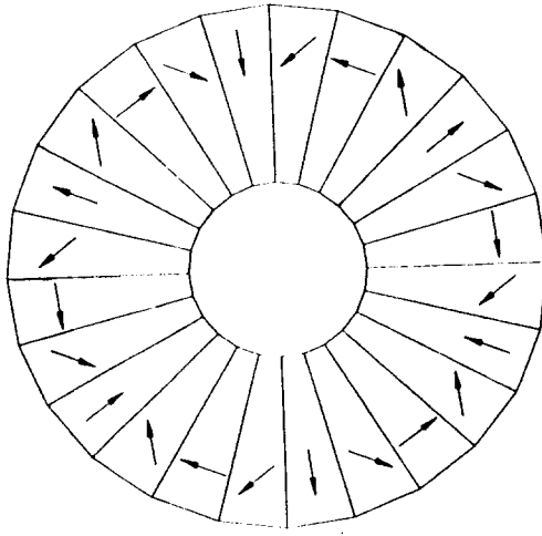
Fig.3 The cross section of the hexapole at the central part
