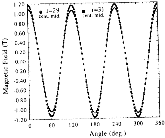
Fig.6 The measured radial magnetic field distribution in azimuthal direction at the center of the hexapole
