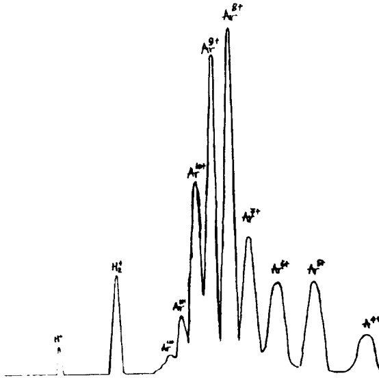
Fig.8 Argon spectrum optimizing for Ar^{11+}
