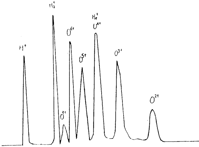
Fig.7 Oxygen spectrum optimizing for O^{6+}
