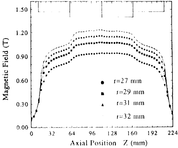
Fig.5 The measured radial magnetic field of the hexapole along the axis at different radius.
