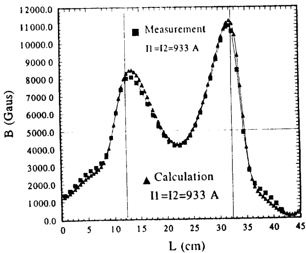
Fig.2 Axial magnetic field distribution
