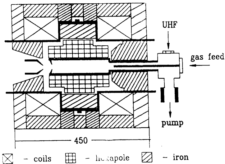
Fig.1 Schematic form of DECRIS-14-2
