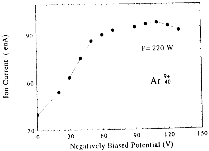
Fig.10 Dependence of the ion current ( Ar^{9+} ) on the negatively biased potential.
