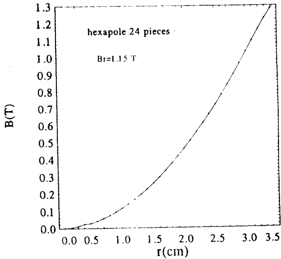
Fig.4 Calculated radial magnetic field of the hexapole at the central part ( 24 pieces )
