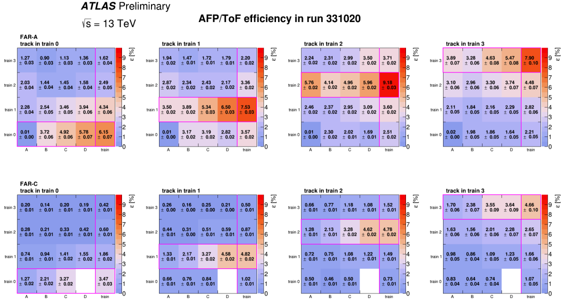
Figure 3: The ToF detector single-channel and train efficiencies (in percent) in the ATLAS run 331020 [16]
