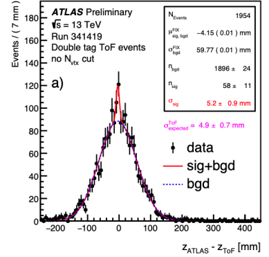
Figure 5: Vertex resolution of AFP ToF detector [16].
