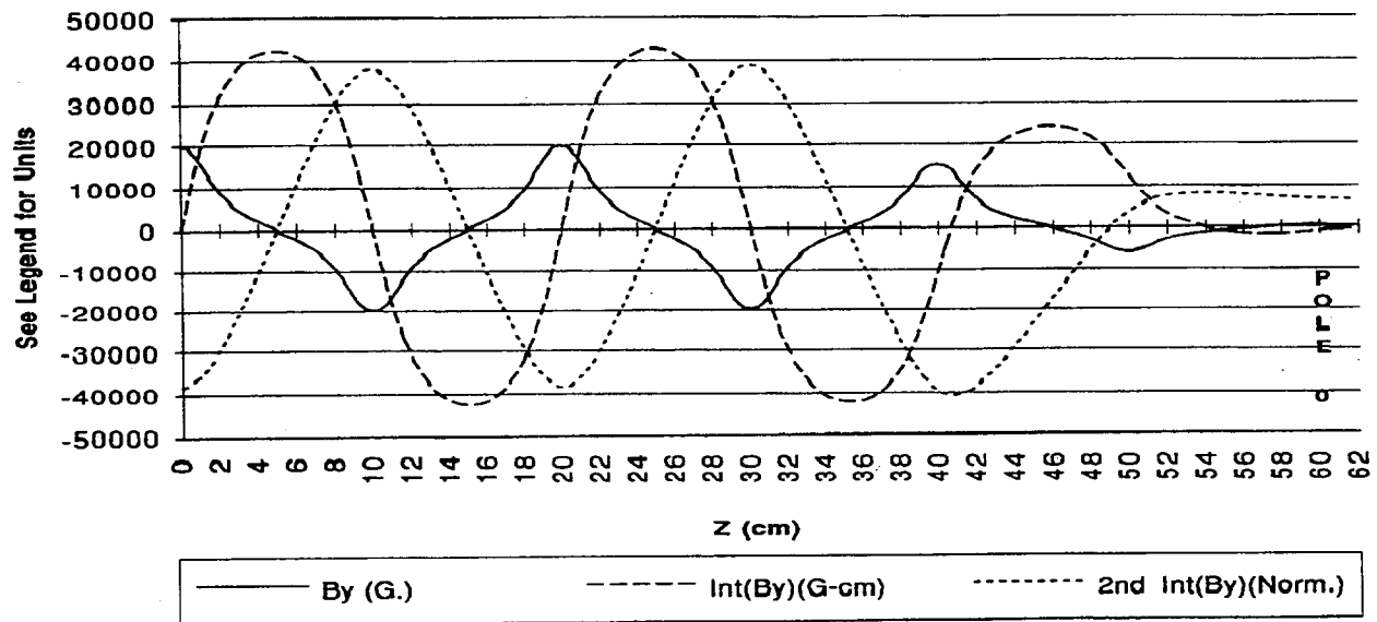
Figure 3: B_y , integral of B_y and trajectory (2nd Integral) from AMPERES calculation
