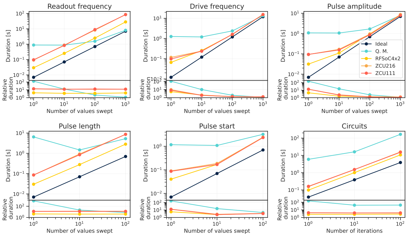
FIG. 5. The top plots illustrate the scaling of execution time with respect to the number of points in a sweep, while the bottom plots depict the ratio between actual execution times on various instruments and the minimum ideal time. “Q.M.” stands for Quantum Machines. The corresponding values were obtained using the same Qibocal interface. The ideal time corresponds to how long the qubit is really used during the experiment, the difference from ideal and real time comes from software delays and communication latency.
