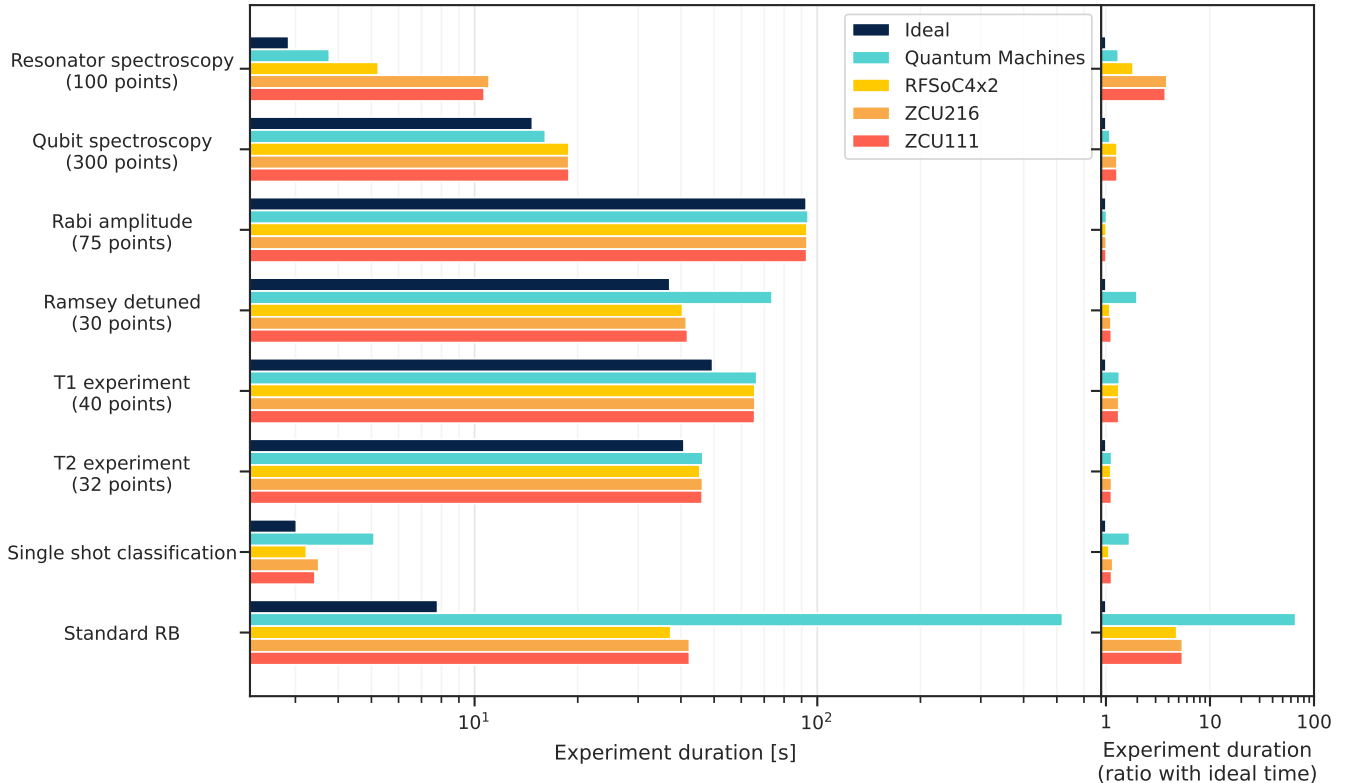
FIG. 4. Execution time of various qubit calibration routines on different electronics. On the left side we show the absolute times in seconds for each experiment. The black bar, that represents the ideal time, shows the minimum time theoretically required for each experiment. On the right side we show the ratio between actual execution time and ideal time, the difference from ideal and real time comes from software delays and communication latency.
