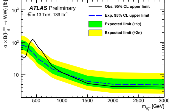
Figure 5: Expected and observed exclusion limits at 95% CL are given for \sigma \times \text{BR}(H_5^{\pm\pm} \rightarrow W^\pm W^\pm) as a function of m_{H_5^{\pm\pm}} in the GM model [3].
