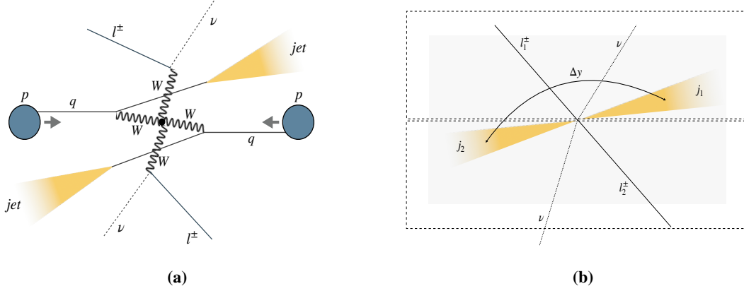
Figure 1: A simplified picture of a proton-proton collision event resulting in the scattering of two W bosons with the same electric charge (left) and a schematic view of the event as seen in the ATLAS detector (right) are given.
