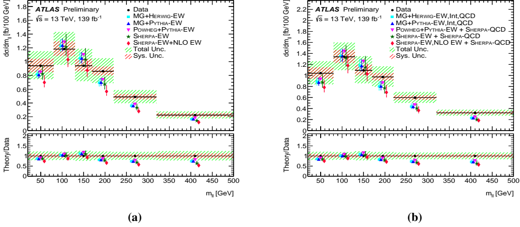
Figure 3: The measured differential cross-section as a function of the dilepton invariant mass is shown for the electroweak production in (a) and the inclusive production in (b) [3]. The results are compared with Standard Model predictions modeled by various MC generators.
