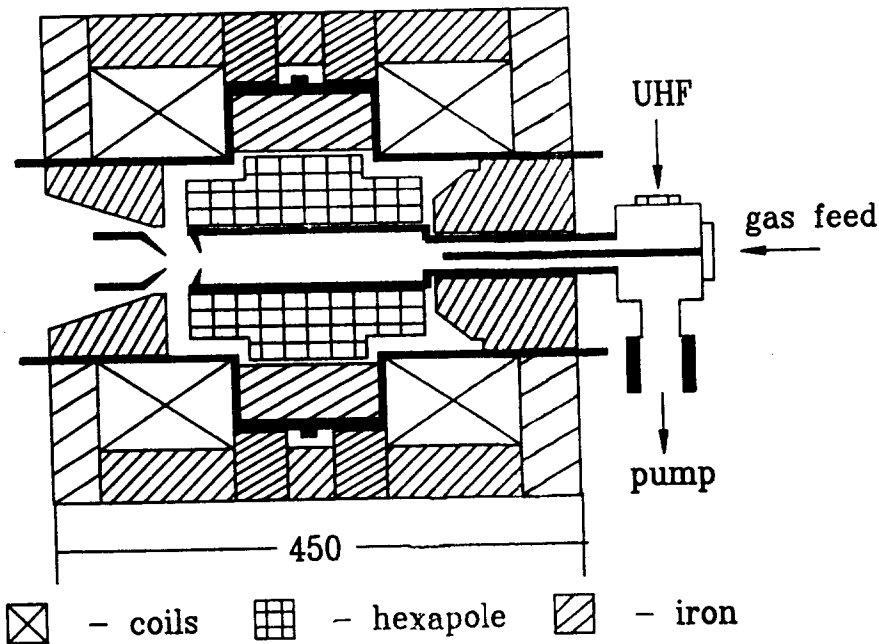
Fig.1 Schematic form of DECRIS-14-2
