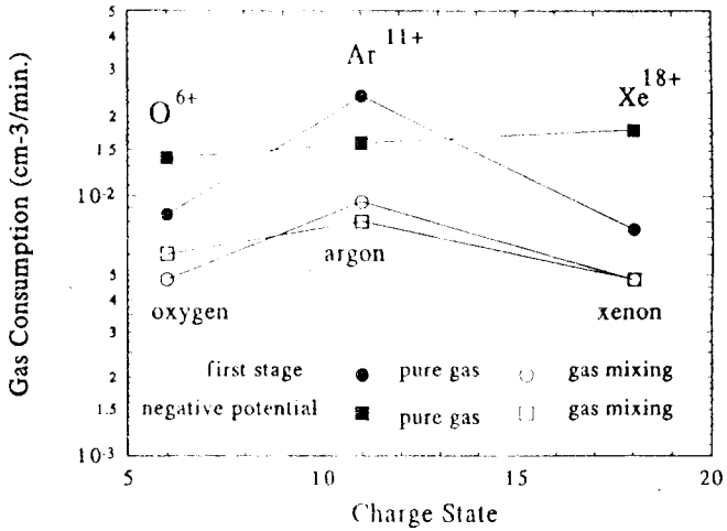
Fig.3 The consumption of the main gases oxygen, argon and xenon with and without the gas mixing.
