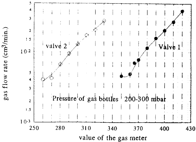
Fig.4 The calibrated curves of the two piezo valves used in the experiments.
